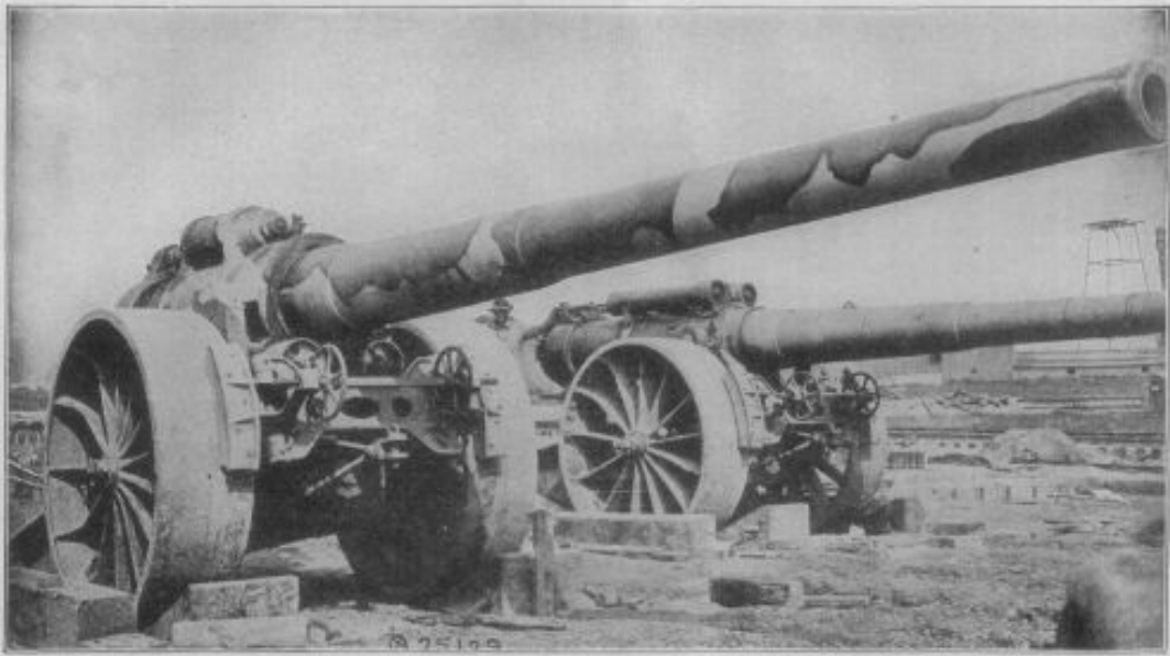
The longest-range field gun in the world, produced by the Ordnance Department, U. S. Army, for service in France, though the hostilities ceased before they reached General Pershing. More than a hundred of these guns are said to have been prepared for shipping to France, and their range and power would probably have astonished the Germans, as did the great naval guns, mounted on railway cars and manned by American seamen, that did such effective work in the closing days of the conflict. (U. S. Official Photo.)
