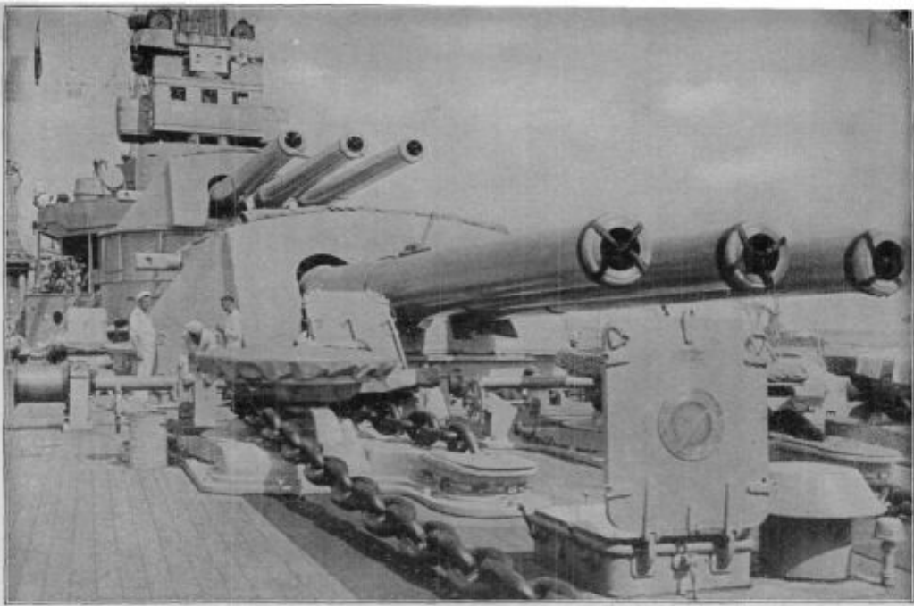
The United States battleship Pennsylvania, showing an unusual view of some of her heavy guns. This vessel is the pride of the Navy and was selected to escort President Wilson on his voyage to Europe to attend the Peace Conference. She led the way across the Atlantic, steaming ahead of the George Washington, on which the President and his party of 200 were passengers. She carries twelve 14-inch and twenty-two 5-inch guns.
