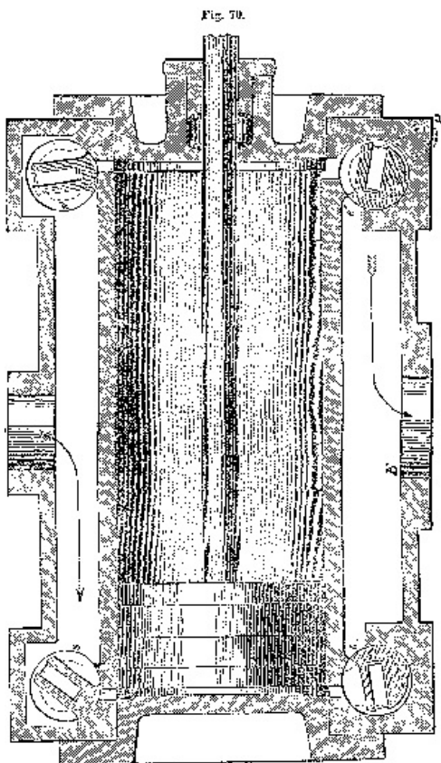
Fig. 70 is a section of the cylinder and valve chests of a horizontal Corliss engine. S is the steam
