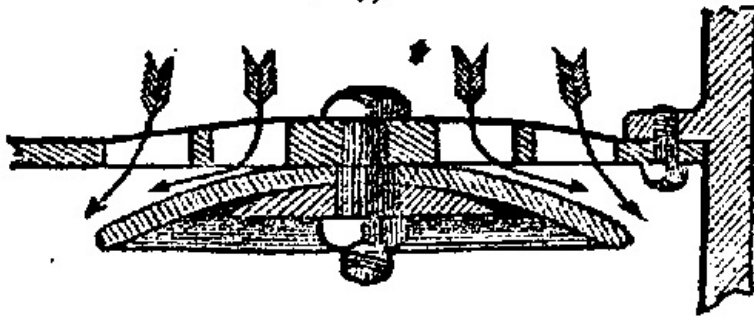
PENN'S DISC VALVE FOR AIR PUMP. Section.
