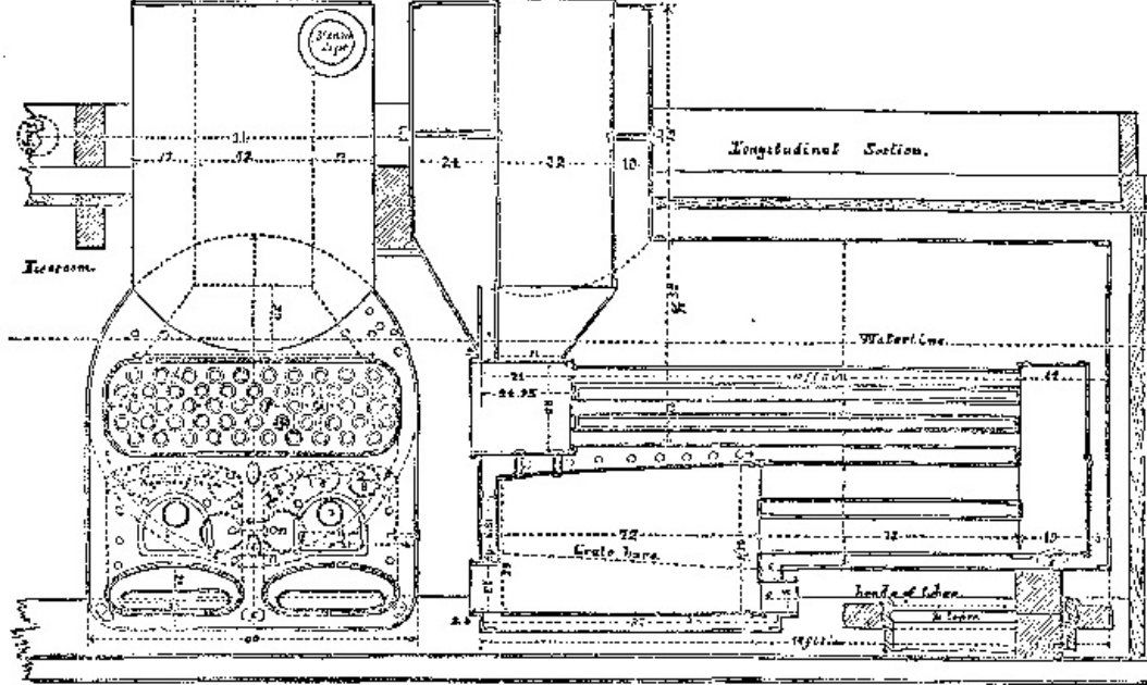
Figs. 14 and 15 are the front and sectional elevation of one of the boilers of the U.S. steamer Water Witch.
