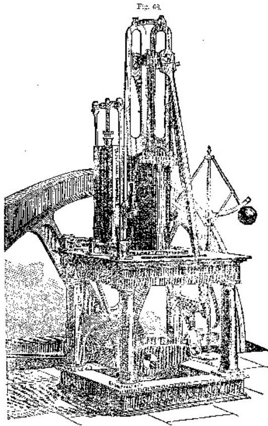
Fig. 68 is a compact vertical engine, as built by R. Hoe & Co., of this city. It is intended to drive printing presses, but is adapted to any kind of work, and is especially suited to such places as require economy of space. Although the value of expansion has been called in question by some of the engineers of the United States Navy, and under an appropriation from Congress is now to be made the subject of experiment; yet, in almost all the manufactories and workshops of the United States, no matter what the form of steam engine, or the purposes to which it is applied, whether stationary, locomotive, or marine, some form of cut-off, by which expansion of the steam can be availed of, is considered indispensable. Many varieties are in use, but those engines are most popular in which the cut-off is applied directly to the valves on the cylinder, opening them quickly and shutting off almost instantly, avoiding all wire drawing of the steam at the ports, and regulating the speed of the engine promptly. Of this class of engines, those manufactured by the Corliss Steam Engine Company, of Providence, R.I., are perhaps the widest known, not only for their extensive introduction, but also from having, by a long and successful litigation, established the claims of the patentee, Mr. George H. Corliss.
