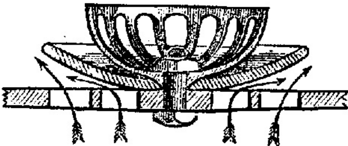
MAUBLAY'S DISC VALVE FOR AIR PUMP. Section.
