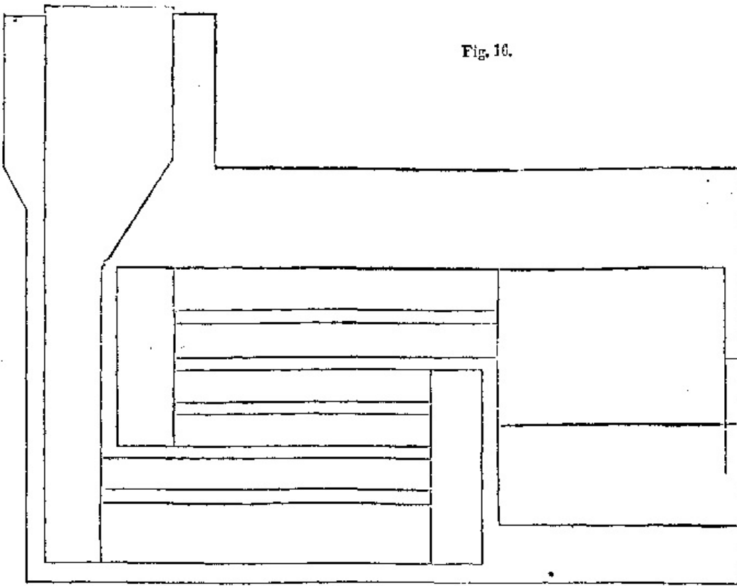
Fig. 16 is a longitudinal section of a boiler of the drop flue variety. For land purposes the lowest range of tubes is generally omitted, and the smoke makes a last return beneath the bottom of the boiler.
