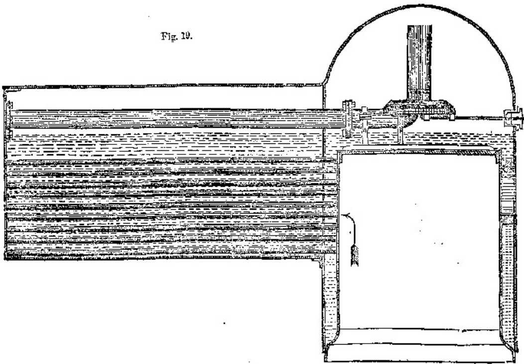
Fig. 19 is a longitudinal section of a common wood-burning locomotive.
