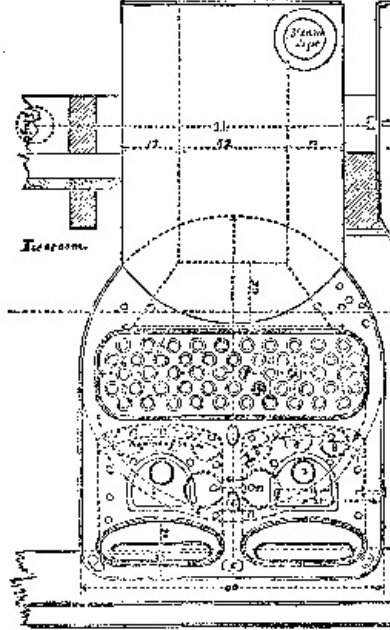
Figs. 14 and 15 are the front and sectional elevation of one of the boilers of the U.S. steamer Water Witch.
