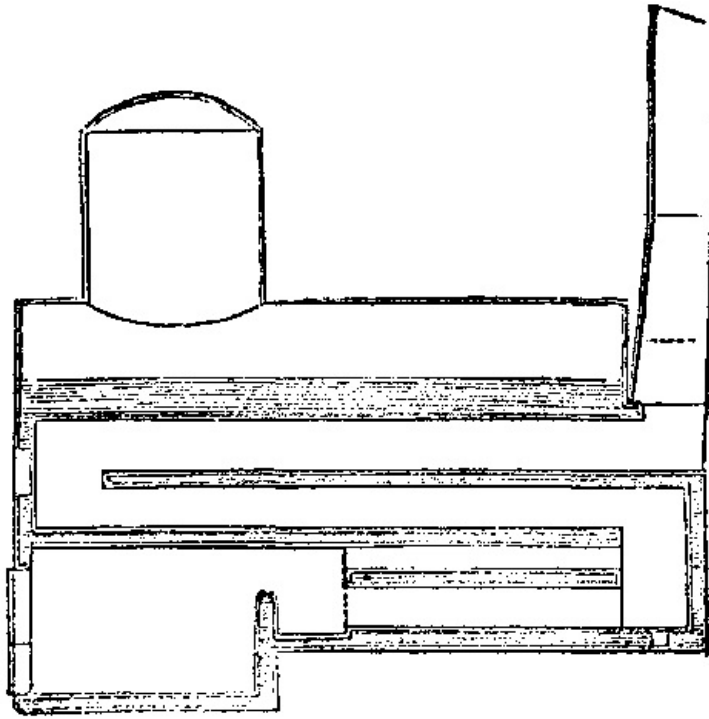
Figs. 12 and 13 are the transverse and longitudinal sections of a common form of American marine boiler.
