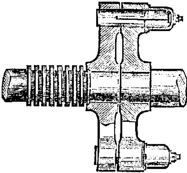
COUPLING CRANKS. Messrs. Bourne & Co.
