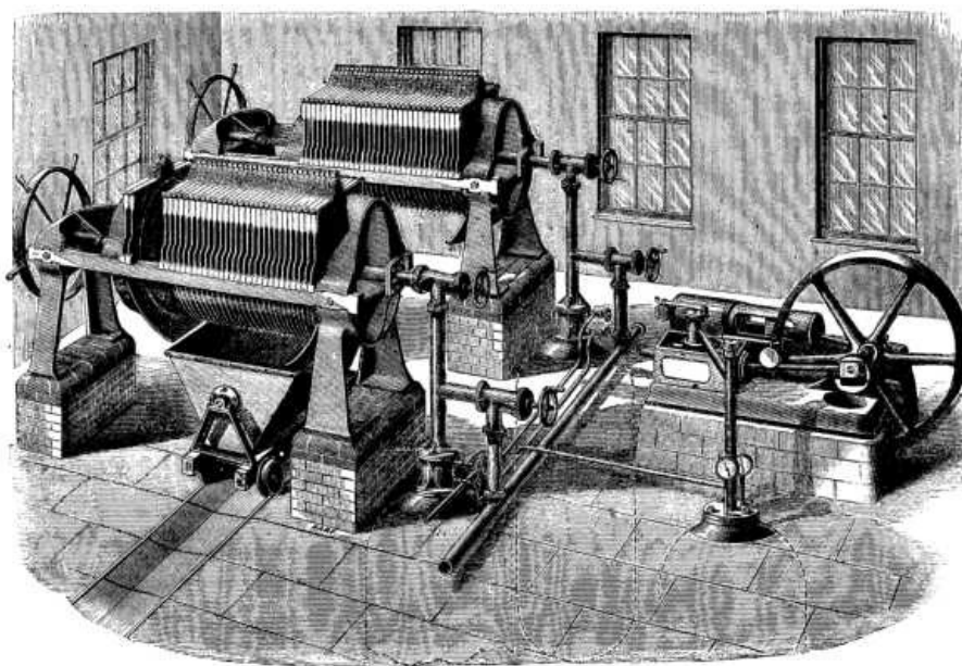
IMPROVED PNEUMATIC FILTERING PRESSES.
