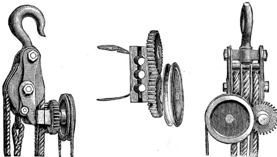
ROPE PULLEY FRICTION BRAKE.
