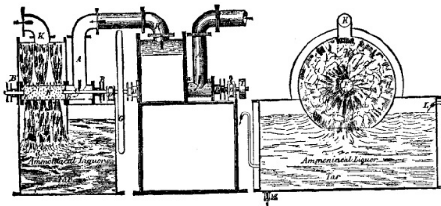
Longitudinal Section. Elevation. Transverse Section.
