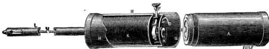
Fig. 2. MECHANISM OR THE INDUCTION SPARK GAS LIGHTER.
