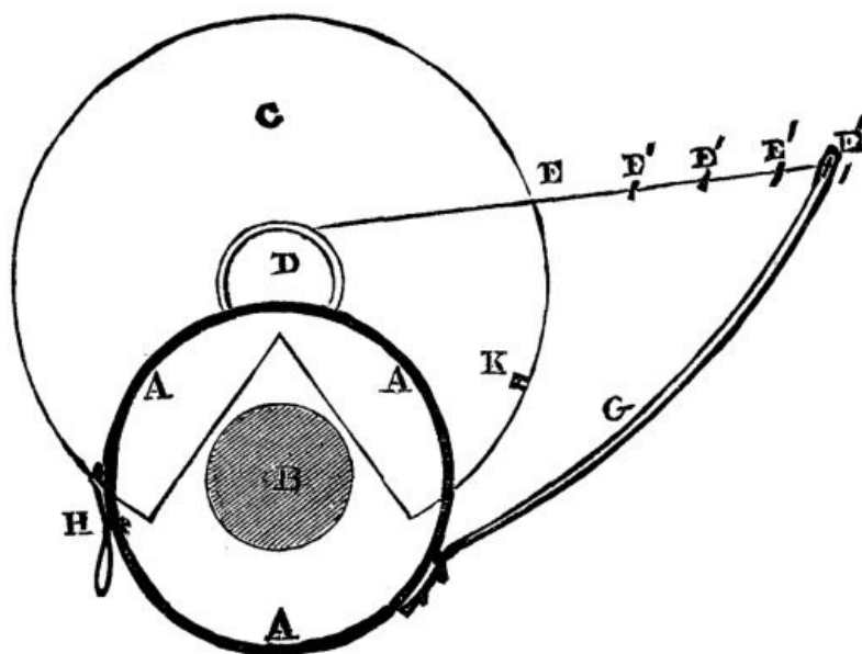
AAA, lens; B, aperture of lens; C, metallic disk; D, wheel on the axis; E, cord or string; E 1 E 1 E 1 E 1 , knots in string; G, steel spring; H, catch; K, socket for catch.
