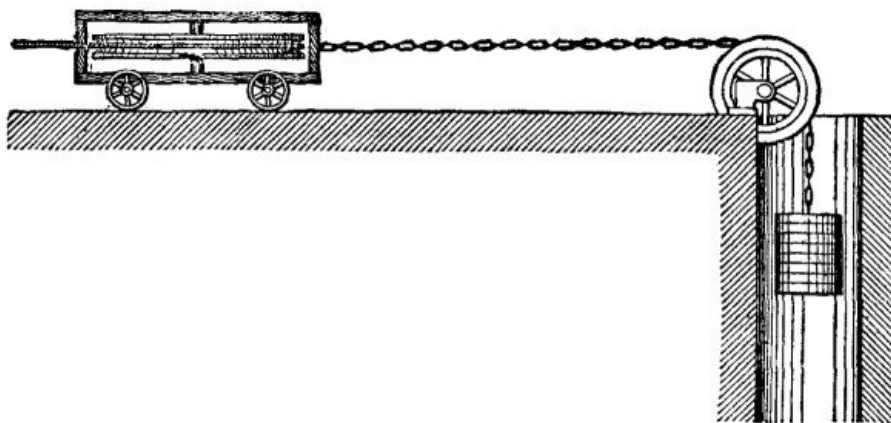
TIGHTENING ARRANGEMENT—ENDLESS ROPE HAULAGE.
