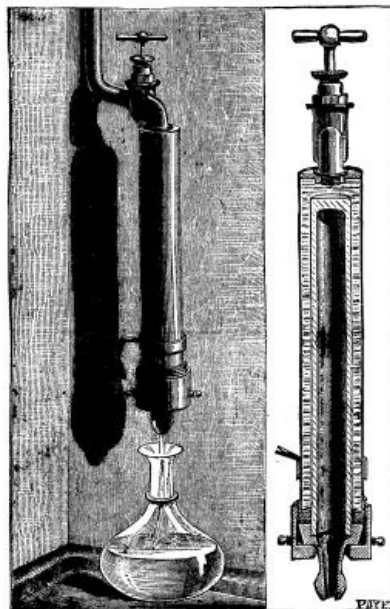
CHAMBERLAND'S WATER FILTER.
