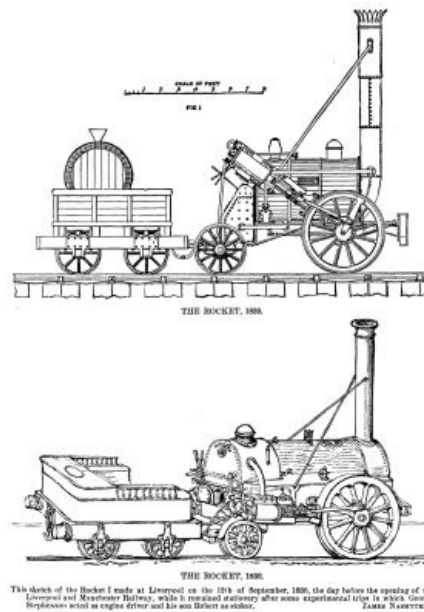
FIG. 1. THE ROCKET, 1829. THE ROCKET, 1830.
