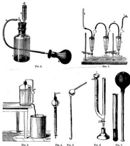
APPARATUS FOR ESTIMATING THE CARBONIC ACID OF THE AIR. 3.—Bertin-Sans Apparatus. FIG. 4.—Bubbling Glass. FIG. 5.—Pipette. FIG. 6.—Arrangement of the U-shaped Tube. FIG. 7.—Wolpert's Apparatus.
