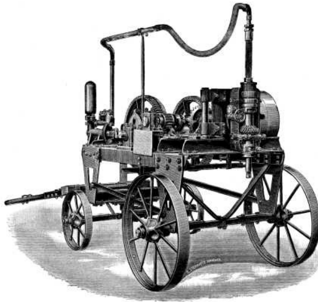
PORTABLE PROSPECTING DRILL.
