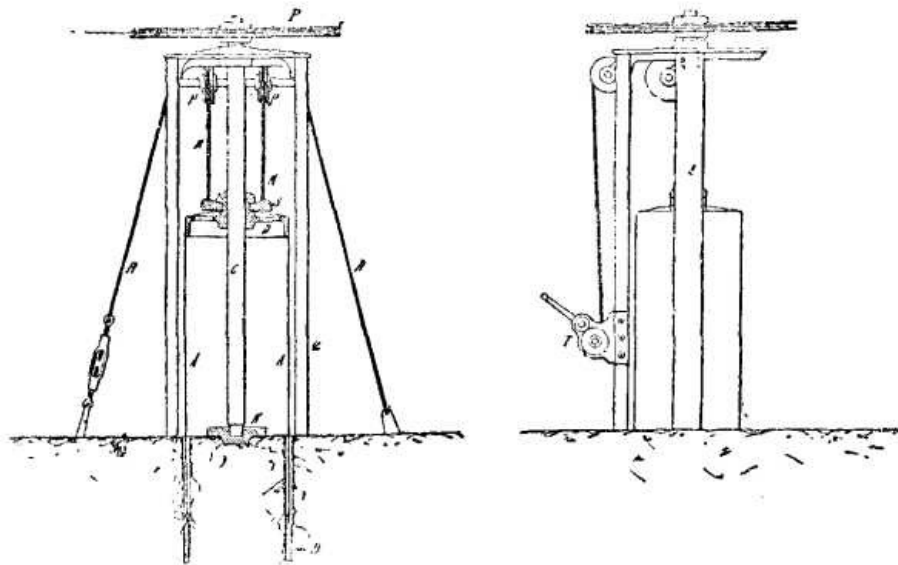
FIG. 6.—TUBULAR PERFORATOR.
