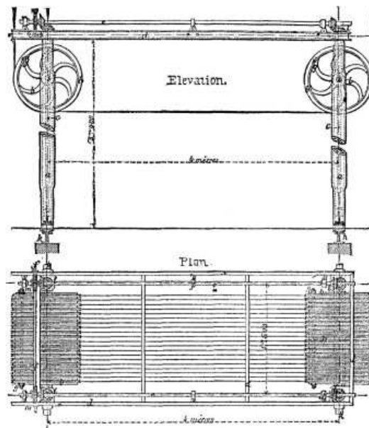
FIG. 4.—APPARATUS FOR SAWING STONE INTO SLABS.
