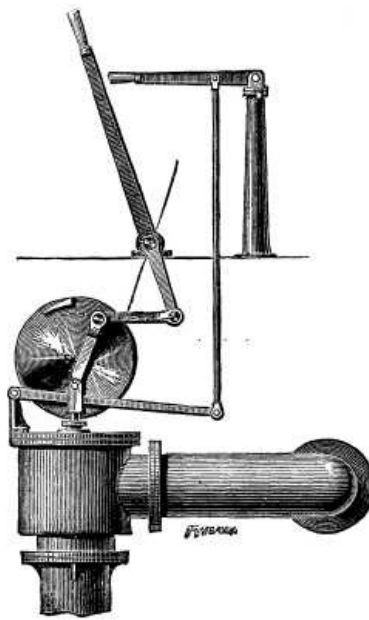
LEWIS & MASSEY'S AUTOMATIC SAFETY GEAR.
