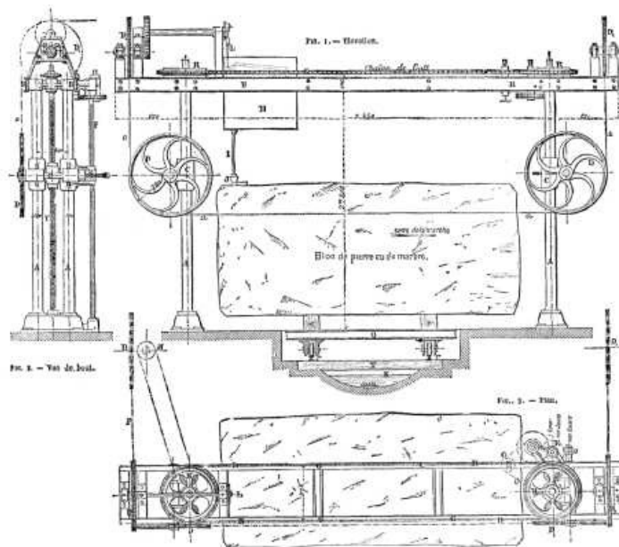
FIGS. 1, 2 and 3.—APPARATUS FOR SAWING STONE.
