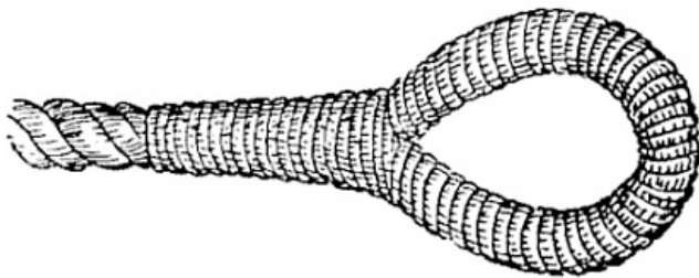
FIG. 94.—Artificial eye (whipped).
