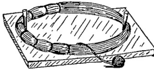
FIG. 89.—Seizing a selvagee strap.
