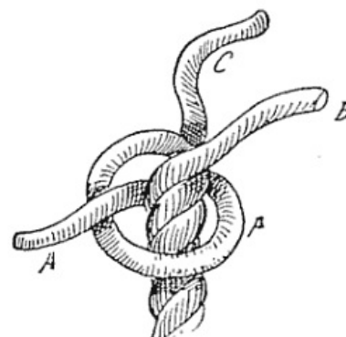
FIG. 131.—Matthew Walker (making)
