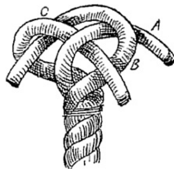
FIG. 111.—Single crown (making).
