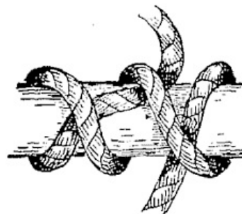
FIG. 48.—Rolling hitch.
