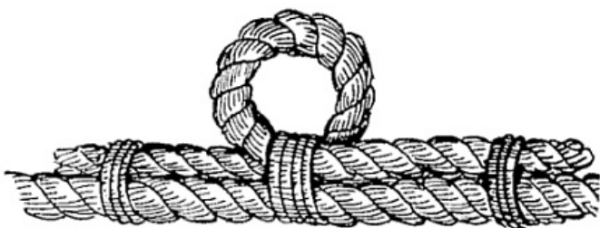
FIG. 96.—Lashed cut-splice.
