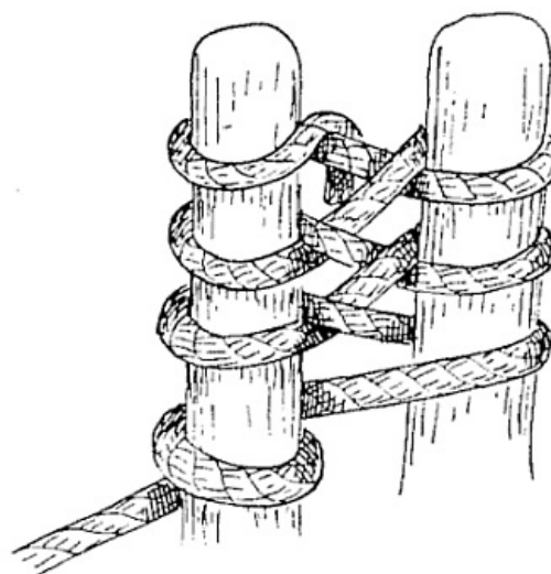
FIG. 57.—Cleat and wharf ties.
