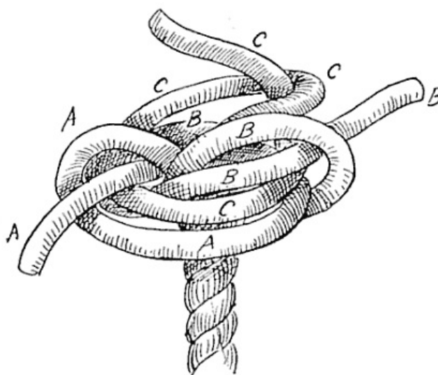
FIG. 132.—Matthew Walker (complete but slack).
