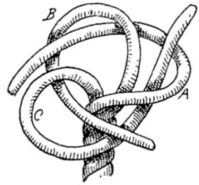
FIG. 115.—Wall knot (making).
