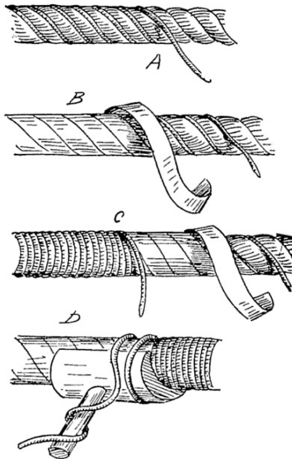
FIG. 138.—Worming, parcelling, and serving.
