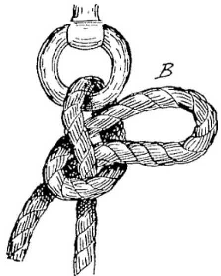
FIG. 32.—Slippery hitch (complete).
