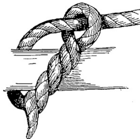
FIG. 38.—Timber hitch.
