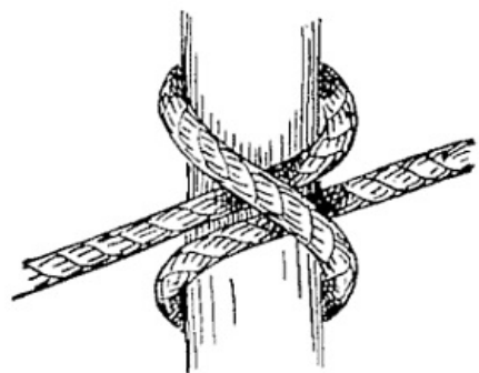
FIG. 55.—Waterman's knot.
