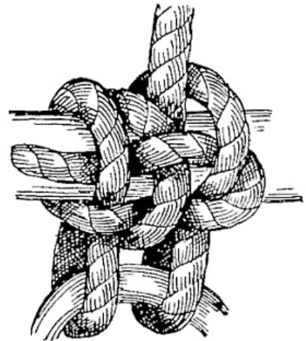
FIG. 51 B. —Roband hitch (back).
