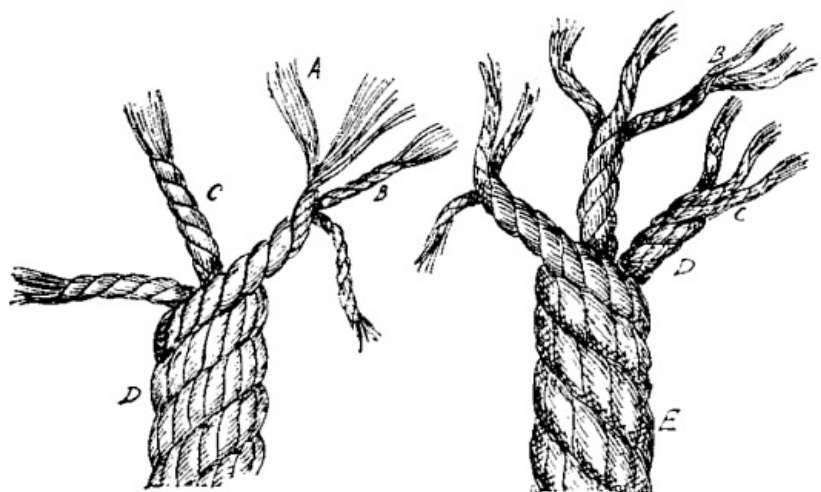
FIG. 1.—Construction of rope.
