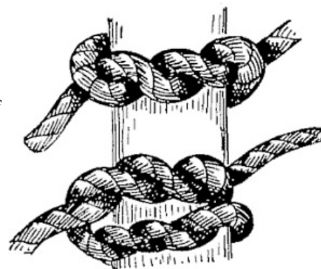
FIGS. 40 and 41.—"Twists."
