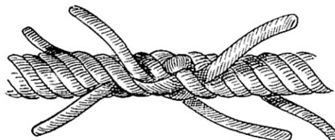
FIG. 106 D .—Short splice (continued).
