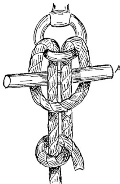
FIG. 30.—Lark's head with toggle ( A ).
