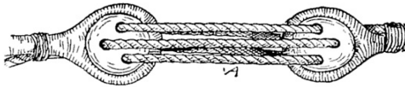
FIG. 98.—Deadeye lashing.
