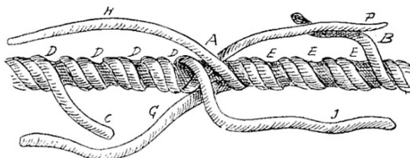
FIG. 107.—Long splice.
