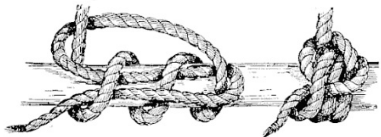
FIG. 54.—Gaff-topsail halyard bend.
