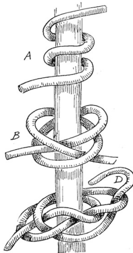
FIG. 135.—Making Turk's head.
