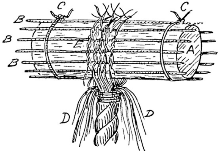
FIG. 90 A.—Making Flemish eye.
