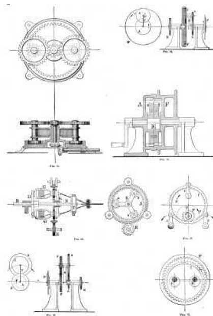
PLANETARY WHEEL TRAINS.
