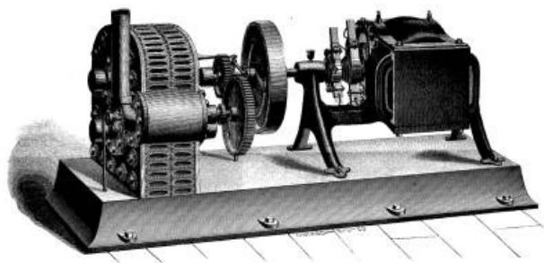
Fig. 1.—THE HARRINGTON ROTARY ENGINE COUPLED TO A DYNAMO.
