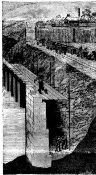
FIG. 1.—CONSTRUCTION OF A DOCK WALL BEHIND PAPONOTS IRON PILE PLANKS.
