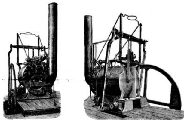
TREVITHICK'S HIGH PRESSURE ENGINE AT CREWE.
