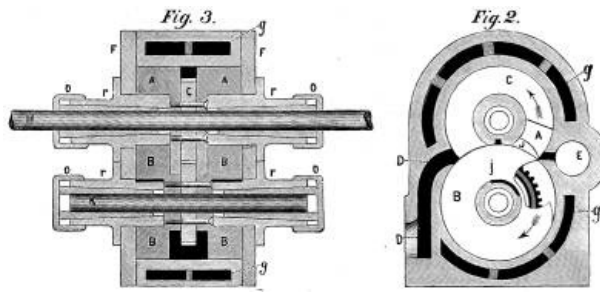
Figs. 2 and 3.—DETAILS OF HARRINGTON ENGINE.
