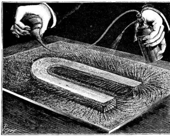
METHOD OF FIXING MAGNETIC PHANTOMS.
