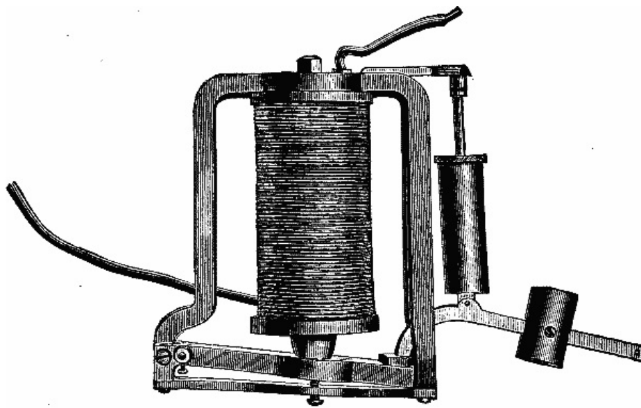
THE CURRENT REGULATOR
