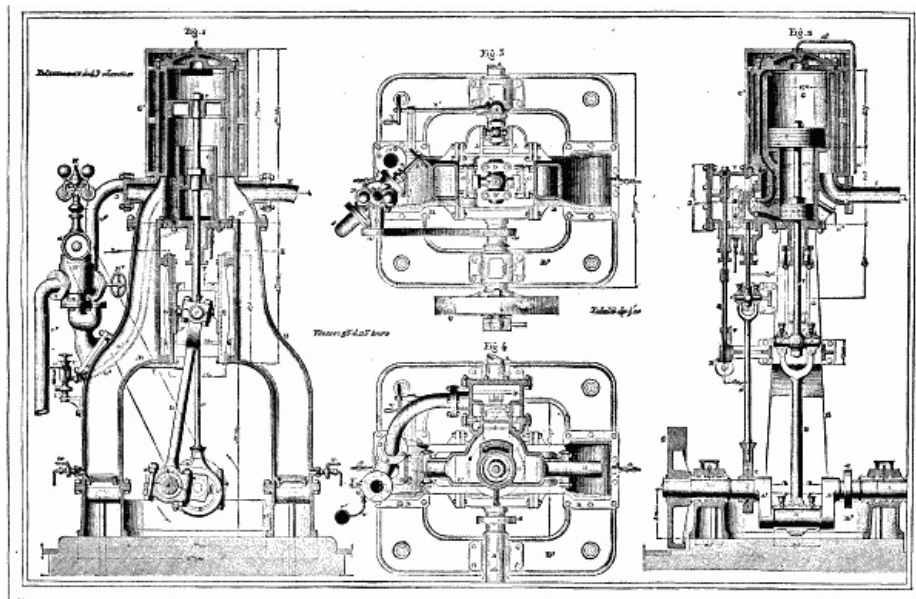
FARCOT'S IMPROVED WOOLF COMPOUND ENGINE.
