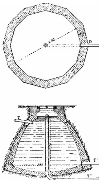
A CEMENT RESERVOIR.
