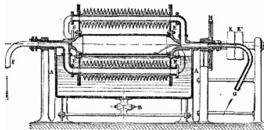
FIG. 1.—LONGITUDINAL SECTION.
