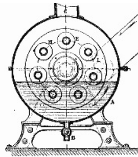
FIG. 2.—TRANSVERSE SECTION.
