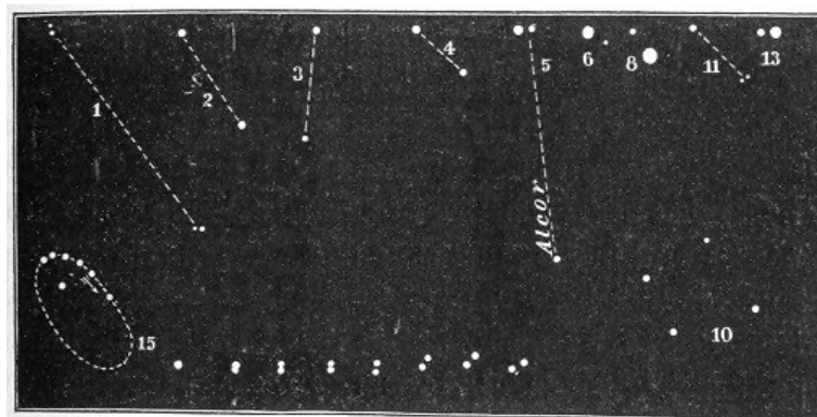
Fig. 75.—Aspects and Revolution of Double Stars.
