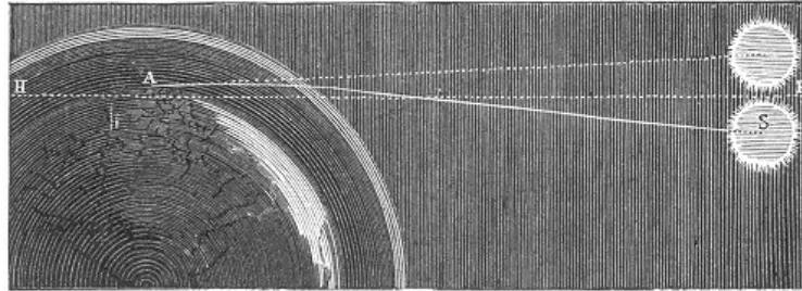
Fig. 12.—Atmospherical Refraction.
