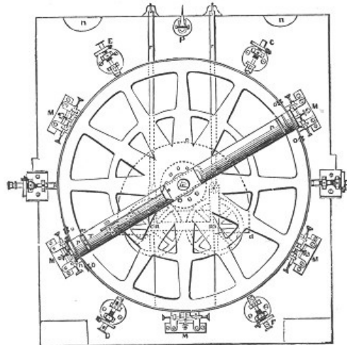
Fig. 21.—Mural Circle.
