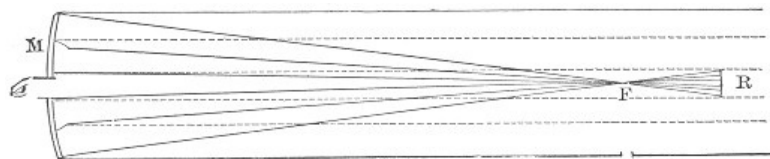
Fig. 14.—Reflecting Telescope.
