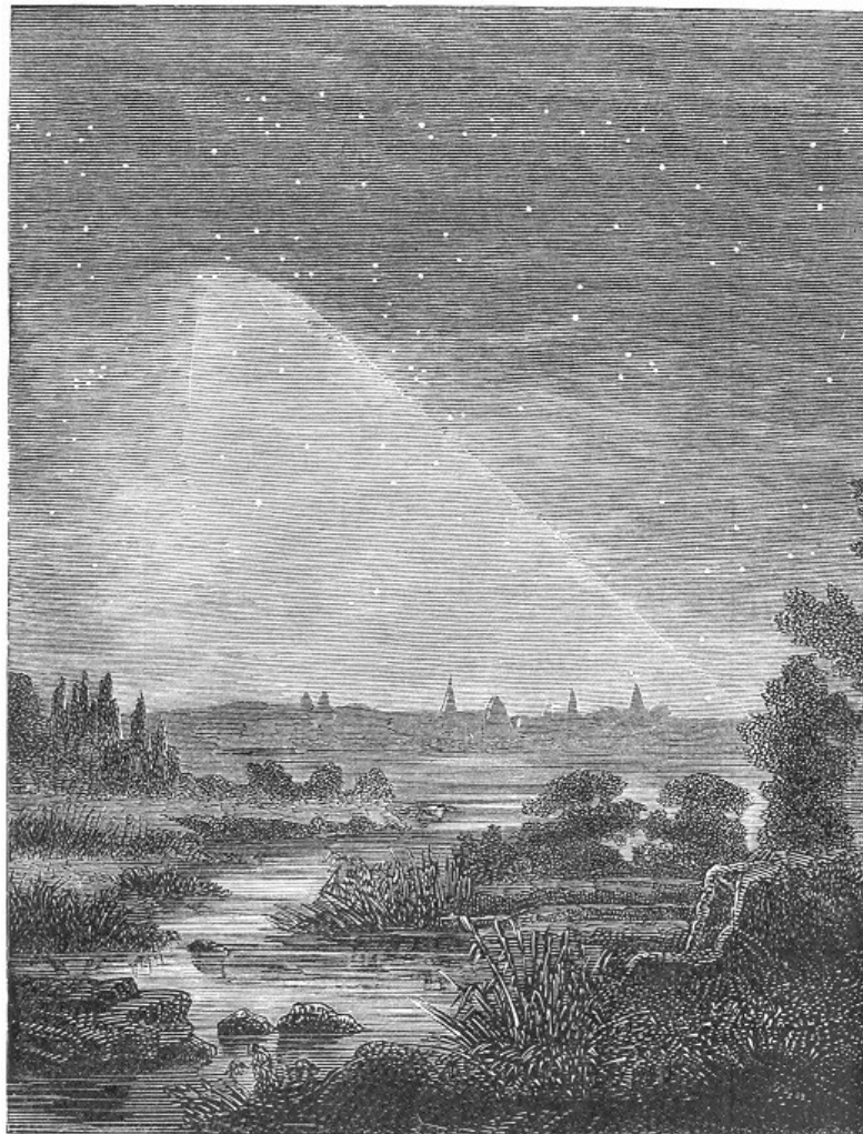
Fig. 31.—Zodiacal Light.
