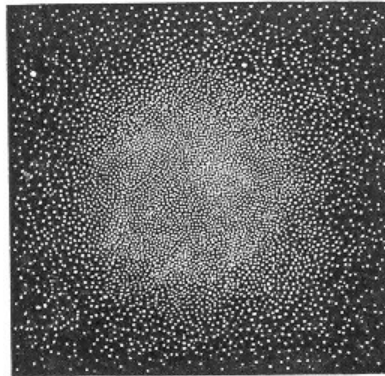
Fig. 77.—Globular Cluster.
