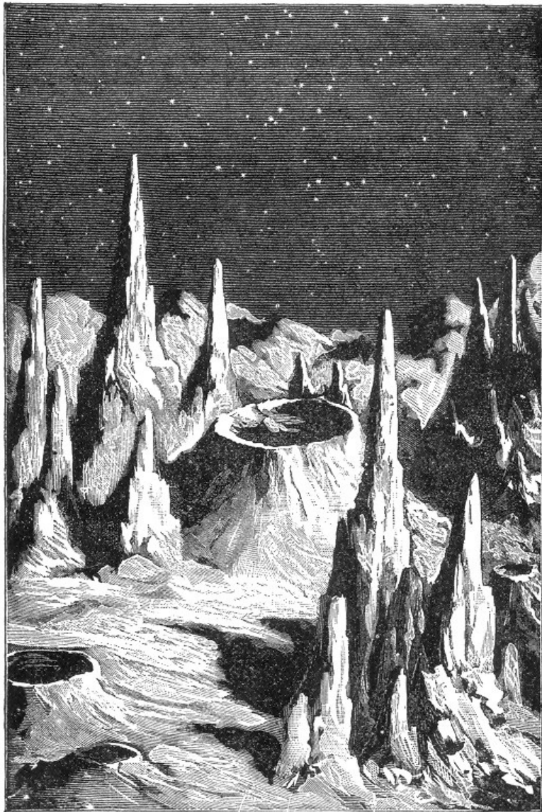
Fig. 57.—Lunar Day.
