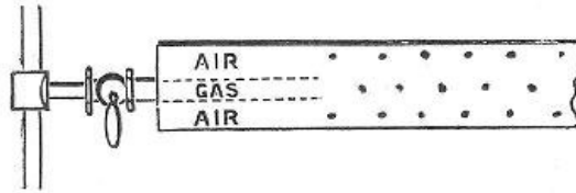
FIG. 4.—Bunsen Burner.
