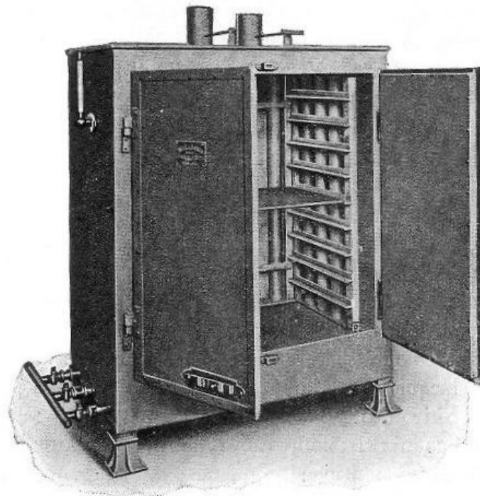
FIG. 13.—Portable Gas Heated Japping and Enamelling Stove fitted with Shelves, Thermometer, etc.
