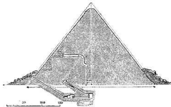
SECTION OF THE THIRD PYRAMID, SHOWING PASSAGES.
