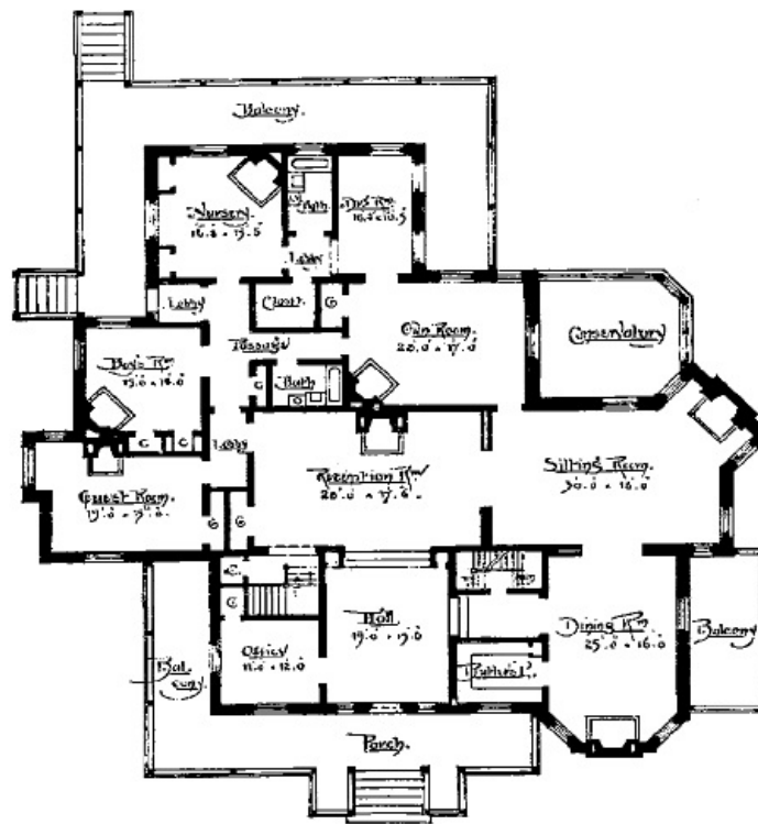
FIRST FLOOR PLAN OF "THE OAKS."
