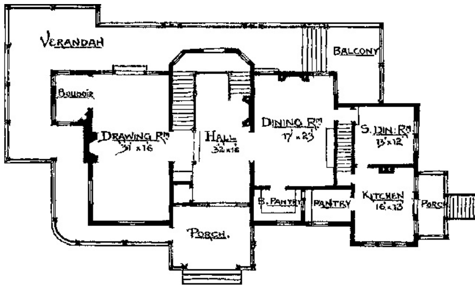
FIRST FLOOR OF WILL'S MASTERPIECE.
