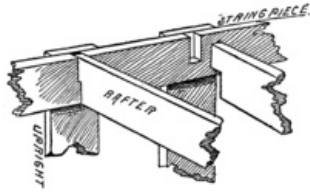
Fig. 185. Notching in the Rafters.
