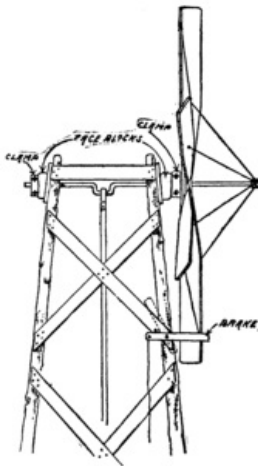
Fig. 290. Side View of the Wind Wheel, showing Brake.
