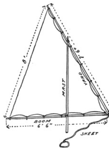
Fig. 11. The Lanteen Sail.
