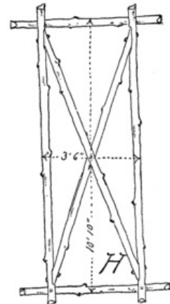
Fig. 312. H Frame (make one).
