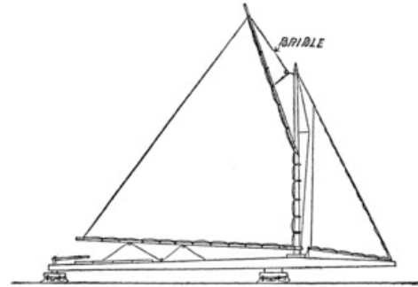
Fig. 173. The Ice Boat Completed.
