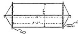
Fig. 6. Dimensions of Double Swedish Sail. N. B.—The mark (') means feet and (") means inches.
