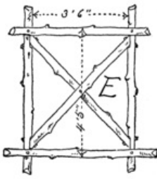
Fig. 309. E Frame (make four).
