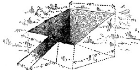
Fig. 182. Excavation for the Cave.
