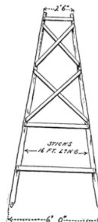
Fig. 283. Frame for the Tower.
