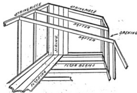
Fig. 184. The Siding and Flooring.
