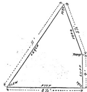
Fig. 169. The Mainsail.
