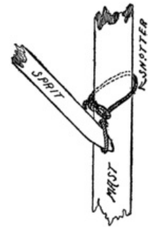
Fig. 193. The Snotter.
