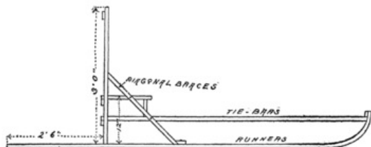
Fig. 179. Dimensions of Rennwolf.
