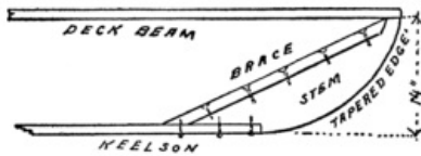
Fig. 105. Stern of the Canoe.
