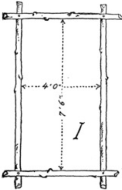
Fig. 313. I Frame (make one).
