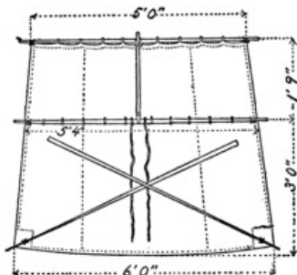
Fig. 15. The Danish Sail.
