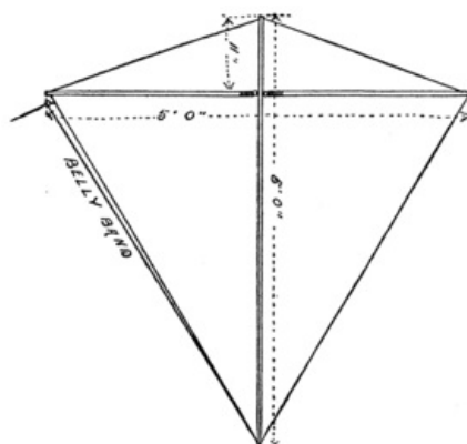
Fig. 241. The 5-foot Malay Kite.
