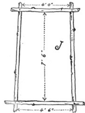
Fig. 314. J Frame (make one).
