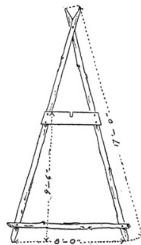
Fig. 251. Frame for Large Tower.
