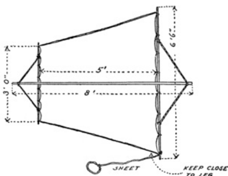
Fig. 9. Changing Tack.
