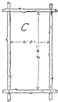
Fig. 307. C Frame (make four).
