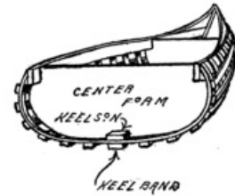
Fig. 128. Section at Center of Canoe.
