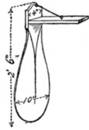
Fig. 121. A Lee Board.
