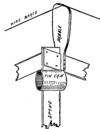
Fig. 258. How the Paddles and Cans Were Attached.
