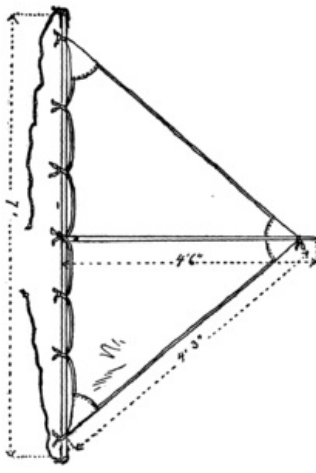
Fig. 5. "Bill's" Sail Complete.
