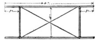
Fig. 246. The Narrow Frame.
