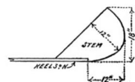
Fig. 126. The Stem Piece.
