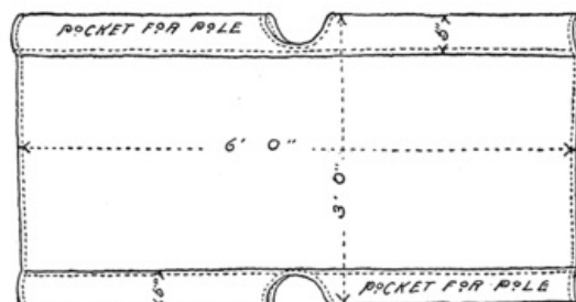
Fig. 208. Canvas Bed.
