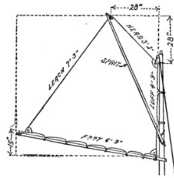
Fig. 192. Mainsail of Scooter Scow.
