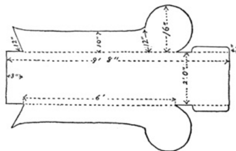
Fig. 200. Bottom Piece of Sleeping Bag.
