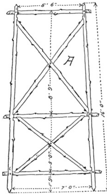
Fig. 305. A Frame (make four).
