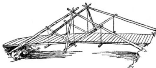
Fig. 100. The King Rod Bridge.
