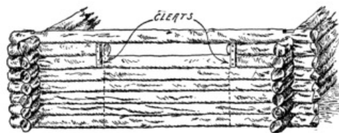
Fig. 269. Piece Cut Out to Admit Saw.
