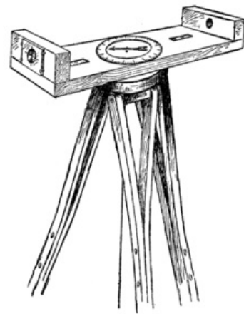
Fig. 75. The Surveying Instrument Complete.
