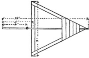
Fig. 164. Frame of the Ice Boat.
