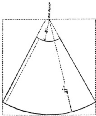
Fig. 55. Layout of the Megaphone.
