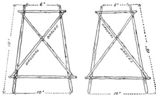
Figs. 91 and 92. Frames for the Spar Bridge.
