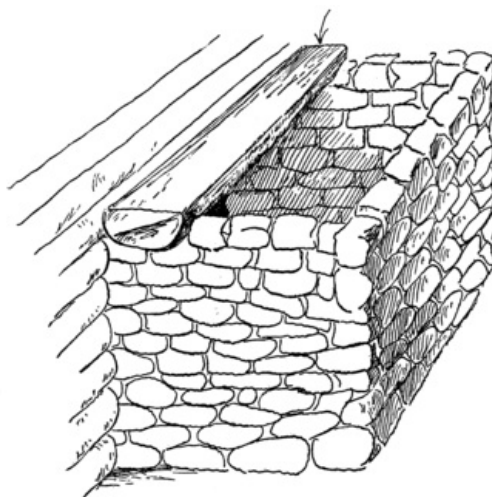
Fig. 274. Building the Chimney.
