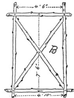
Fig. 306. B Frame (make four).
