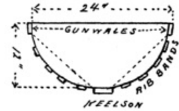
Fig. 106. Center Form.
