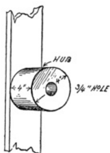
Fig. 255. The Hub.
