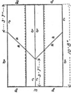
Fig. 39. Cutting out the Door Flaps.
