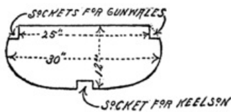
Fig. 124. Center Form.
