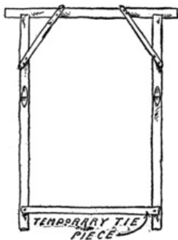
Fig. 101. The King Post Frame.
