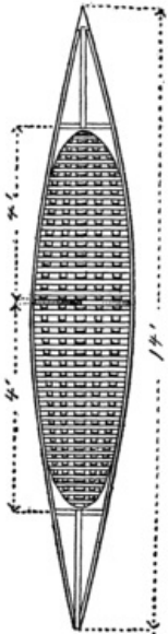
Fig. 109. Top View of the Canoe Frame.
