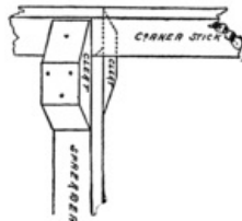
Fig. 245. Corner Stick and Spreader.
