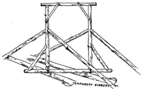
Fig. 103. The Permanent Cross Beam Made Fast.
