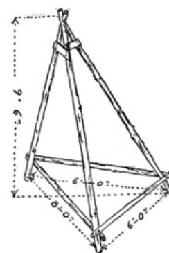
Fig. 254. The Small Tower.
