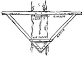
Fig. 138. Main Girder of the Tree House.
