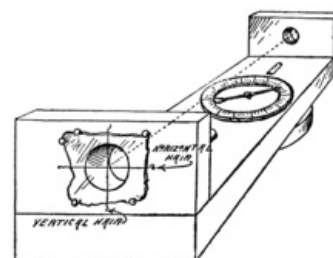
Fig. 72. Sighting Blocks on the Baseboard.
