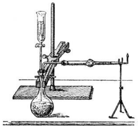
ANALYTICAL APPARATUS.
