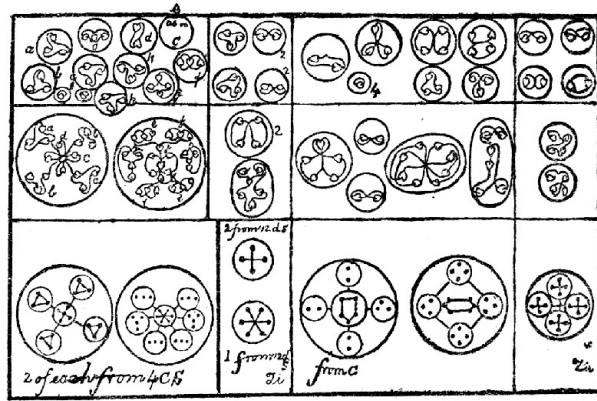
ZIRCONIUM (Plate XV, 2, 5).
