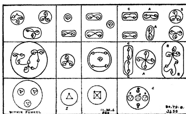
CHLORINE (Plate V, 2).
