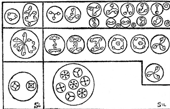
SILICON (Plate XVI, 1).
