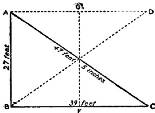
How to mark out a tennis court
