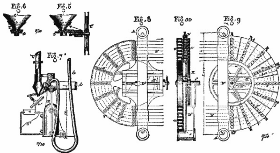
FIGS. 5 through 10 AUGUSTE'S STONE SAW.
