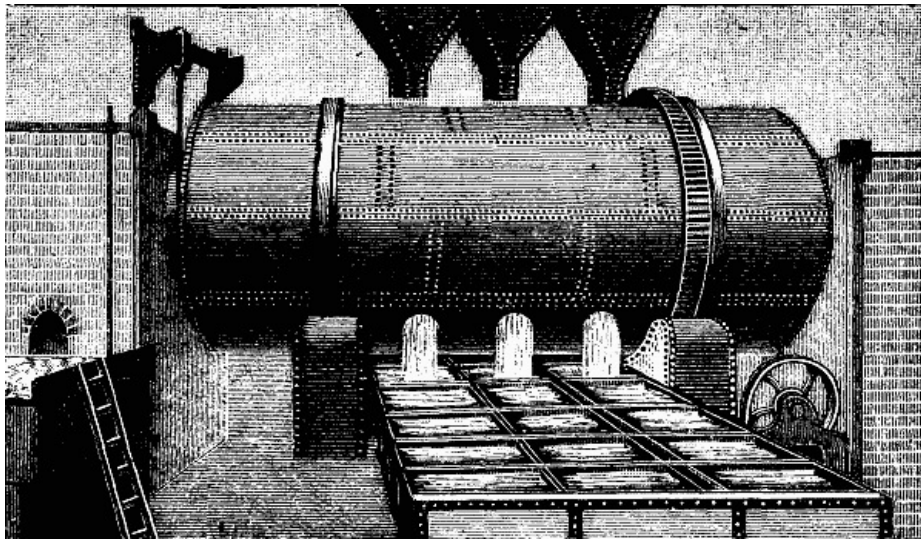
A NEW MONSTER REVOLVING BLACK ASH FURNACE.
