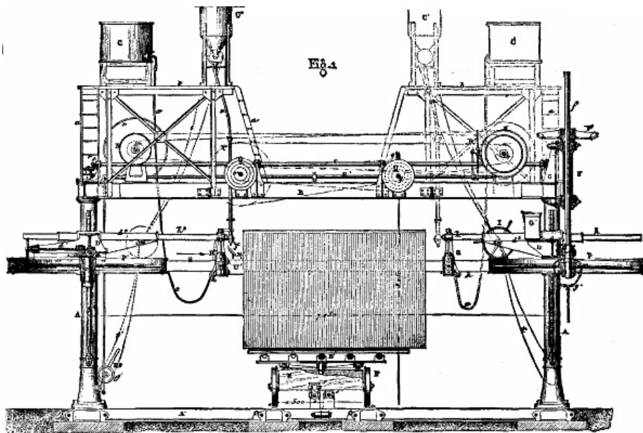
FIG. 1 AUGUSTE'S STONE SAW.
