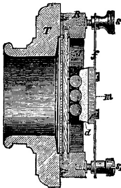
FIG. 3. THE MIX AND GENEST TELEPHONE.
