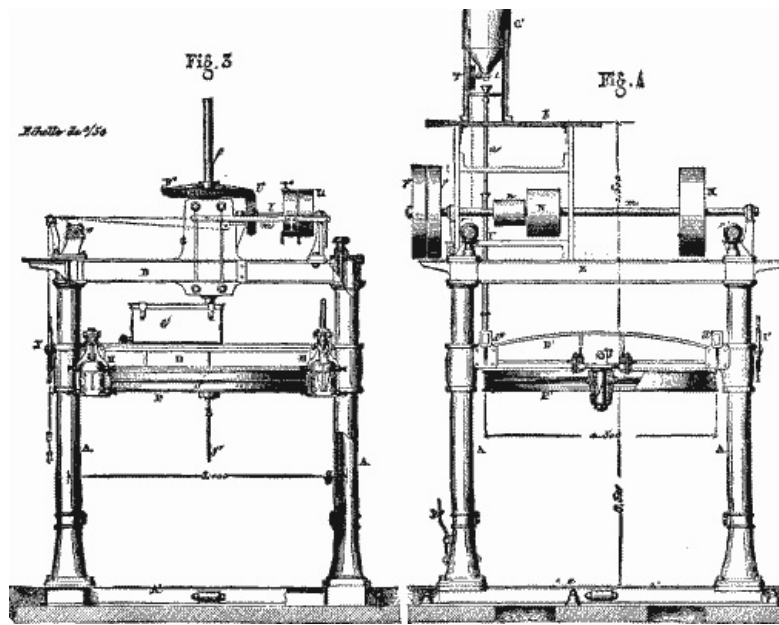
FIGS. 3 and 4 AUGUSTE'S STONE SAW.
