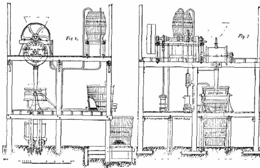
THE NEWBERY-VAUTIN CHLORINATION PROCESS.
