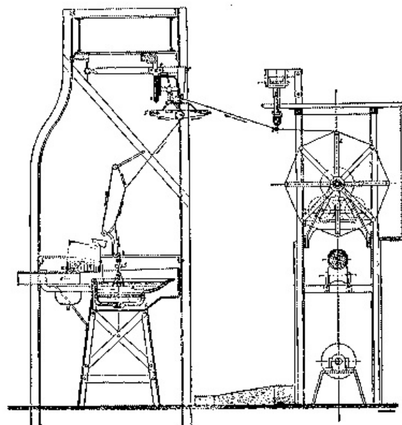
Fig. 1 THE MECHANICAL REELING OF SILK.
