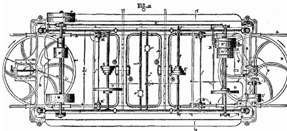
FIG. 2 AUGUSTE'S STONE SAW.
