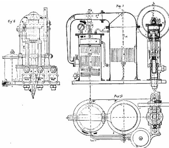
VOLUTE DOUBLE DISTILLING APPARATUS.
