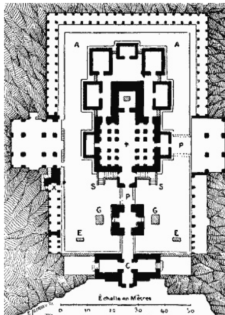
FIG. 2.—PLAN OF THE TEMPLES OF KYLAS.
