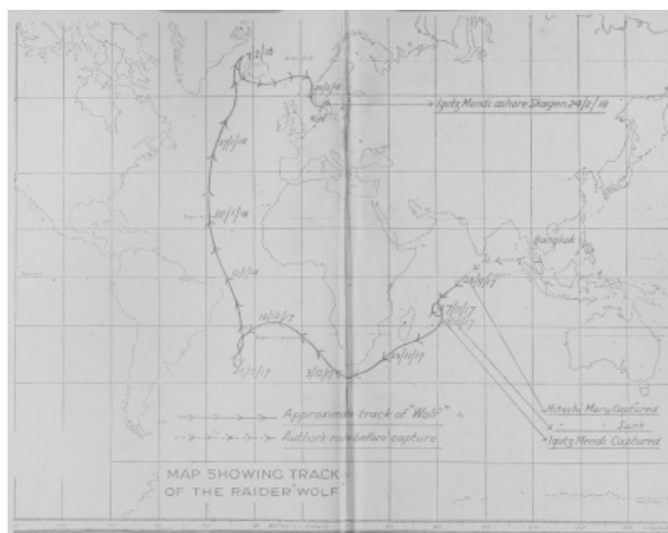
MAP SHOWING TRACK OF THE RAIDER "WOLF"
