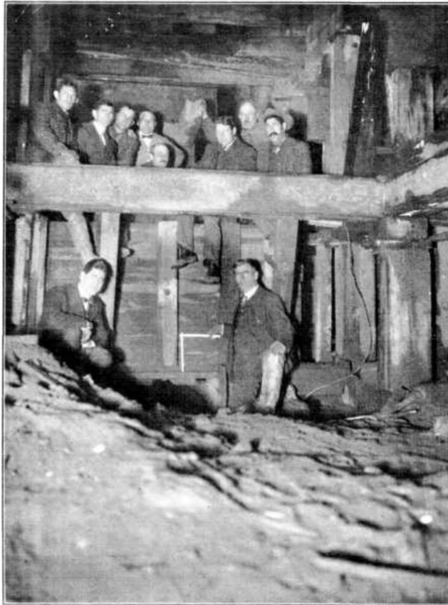
PLATE XXIV, FIG. 1.—INITIAL SETTLEMENT IN 3-FT. SAND ARCH, DUE TO COMPRESSION OF MATERIAL ON REMOVING SUPPORTS FROM BOTTOM.
