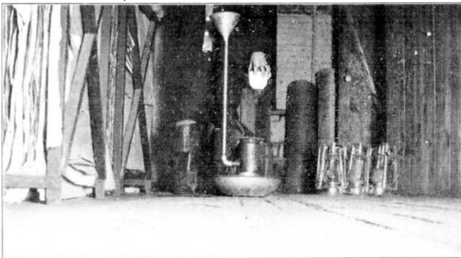
PLATE XXVII, FIG. 2.—SAND PUSHED UP FROM BOWL BY WATER PRESSURE THROUGH GOOSE-NECK.
