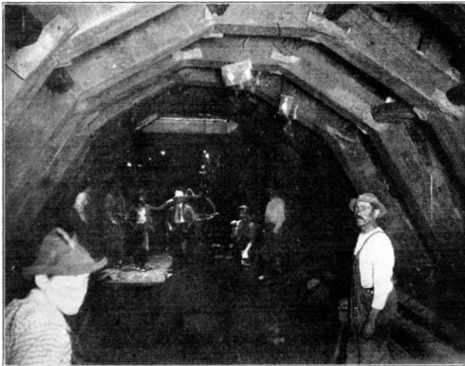
PLATE XXVI, FIG. 1.—TYPES OF ARCH TIMBERS USED IN BAY RIDGE TUNNEL SEWER.
