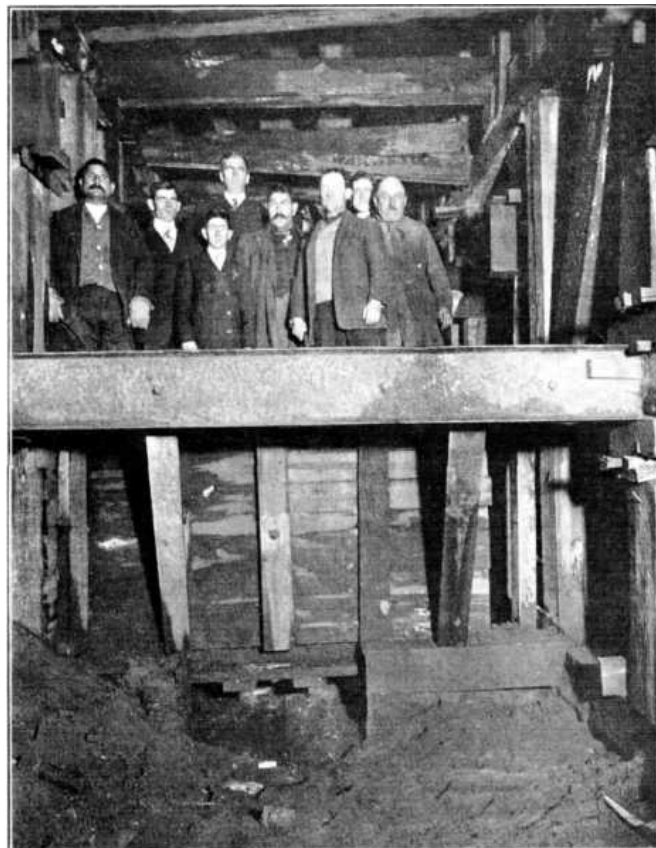
PLATE XXIV, FIG. 2.—FINAL SETTLEMENT OF SAND ARCH, DUE TO COMPRESSION IN EXCESS LOADING.
