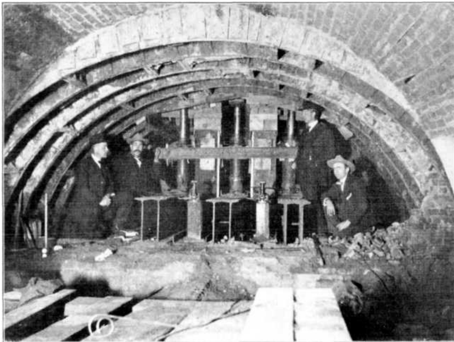
PLATE XXVIII, FIG. 2.—RAISING ROOF OF BATTERY TUBES, IN BROOKLYN, BY "BLEEDING" SAND THROUGH DISPLACED PLATES.
