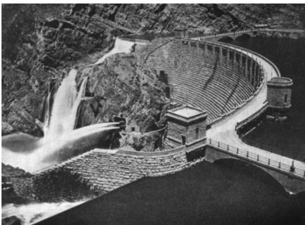
THE ROOSEVELT DAM, PHOENIX, ARIZONA
