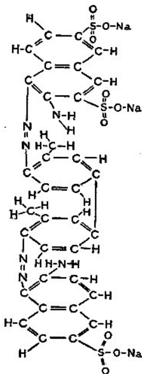
A molecule of a coal-tar dye
