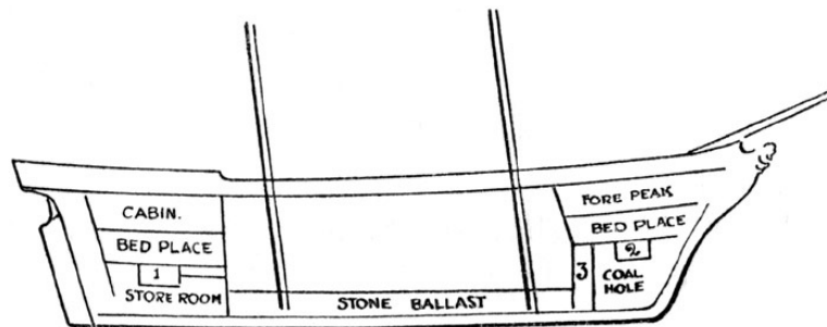
The Schooner Spartan .
