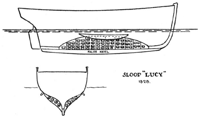
The Sloop Lucy showing Concealments.
