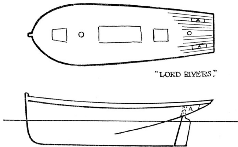
Deck Plan and Longitudinal Plan of the Lord Rivers (see Text).
