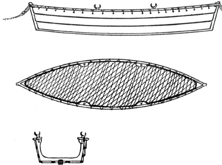
Flat-Bottomed Boat found off Selsey.
