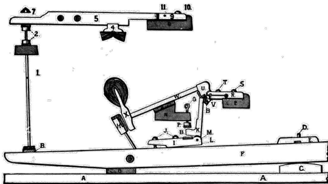
ACTION OF THE SQUARE PIANO.
