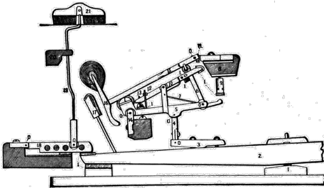
ACTION OF THE GRAND PIANO.
