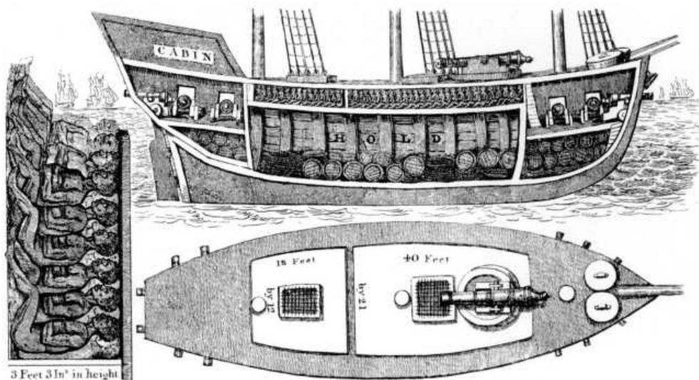
SECTIONS OF A SLAVE SHIP.
