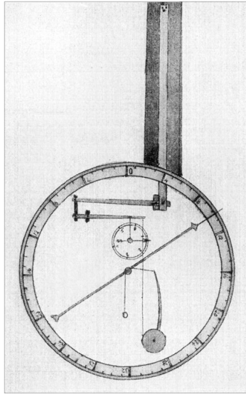
THERMOMETER
