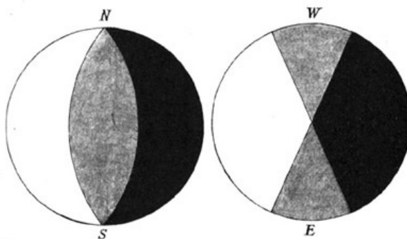
THE REGIONS OF PERPETUAL DAY, PERPETUAL NIGHT, AND ALTERNATE DAY AND NIGHT ON MERCURY. IN THE LEFT-HAND VIEW THE OBSERVER LOOKS AT THE PLANET IN THE PLANE OF ITS EQUATOR; IN THE RIGHT-HAND VIEW HE LOOKS DOWN ON ITS NORTH POLE..
