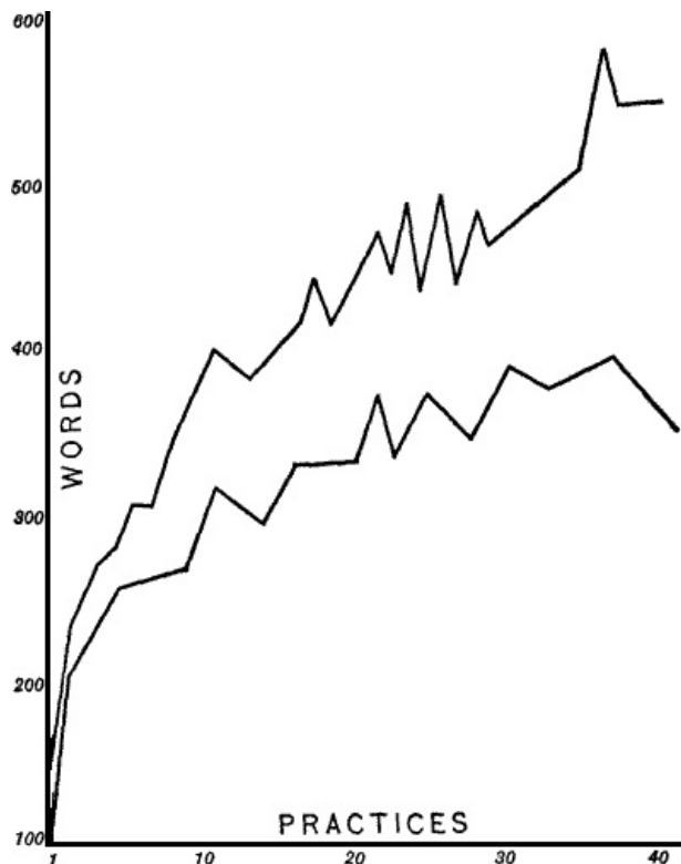
FIGURE III.—LEARNING CURVES
