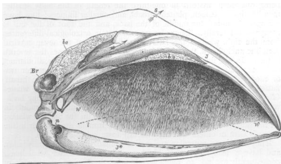
Br, brain cavity; J J*, upper and lower jawbones; the arrows indicate narial passages; S, spout-hole; W, whalebone; t , tongue in dotted line; n , nerve aperture in lower jaw; bo , bone sawed through.
