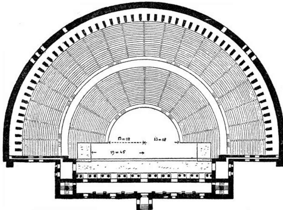
From Durm THE THEATRE AT ASPENDUS
