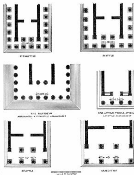
THE CLASSIFICATION OF TEMPLES ACCORDING TO INTERCOLUMNIATION
