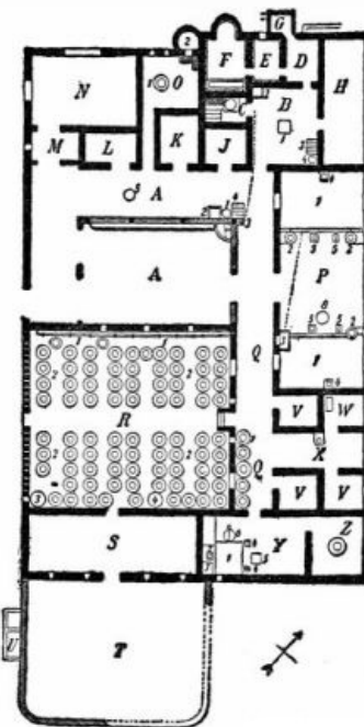
From Mau THE VILLA RUSTICA AT BOSCOREALE NEAR POMPEII A. Court. B. Kitchen. C-F. Baths. H. Stable. J. Toolroom. K, L, V, V. Bedrooms. N. Dining Room. M. Anteroom. O. Bakery. P. Room with two winepresses. Q. Corridor. R. Court for fermentation of wine. S. Barn. T. Threshing-floor. Y. Room with oil press.
