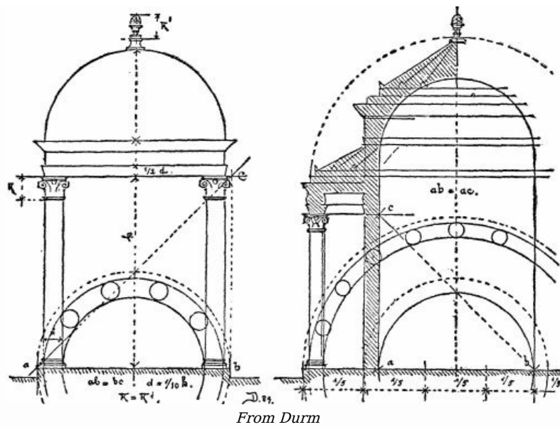
THE CIRCULAR TEMPLE ACCORDING TO VITRUVIUS
