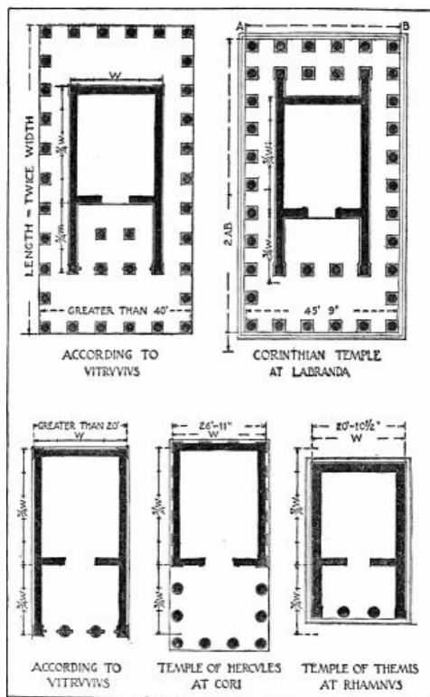
VITRUVIUS' TEMPLE PLAN COMPARED WITH ACTUAL EXAMPLES
