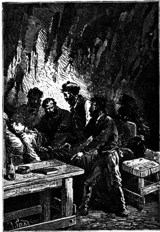
SULPHATE OF QUININE
