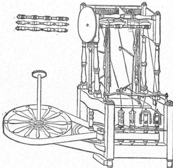
ARKWRIGHT'S FIRST SPINNING-MACHINE. (Ure: History of the Cotton Manufacture. )
