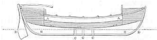
FIG. 1.—SIDE VIEW OF THE LIFEBOAT.
