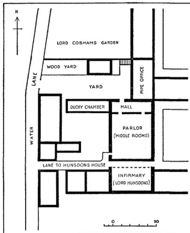
PLAN ILLUSTRATING THE SECOND BLACKFRIARS PLAYHOUSE
