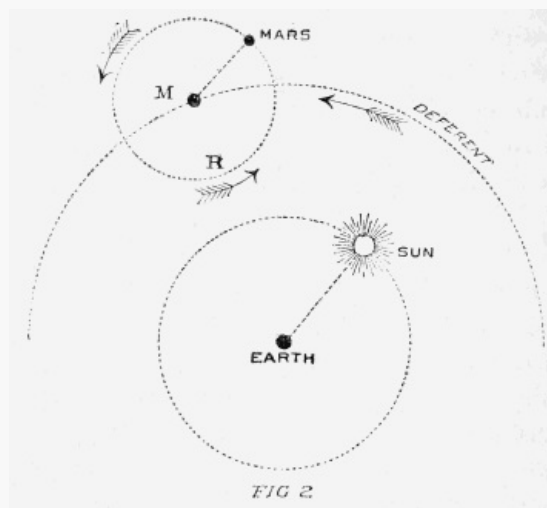
FIG. 2. PTOLEMY'S THEORY OF THE MOVEMENT OF MARS.
