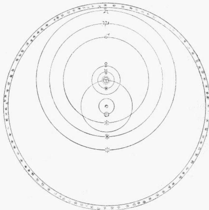
TYCHO'S "NEW SCHEME OF THE TERRESTRIAL SYSTEM," 1577.
