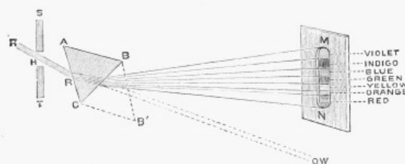
DIAGRAM OF A SUNBEAM.
