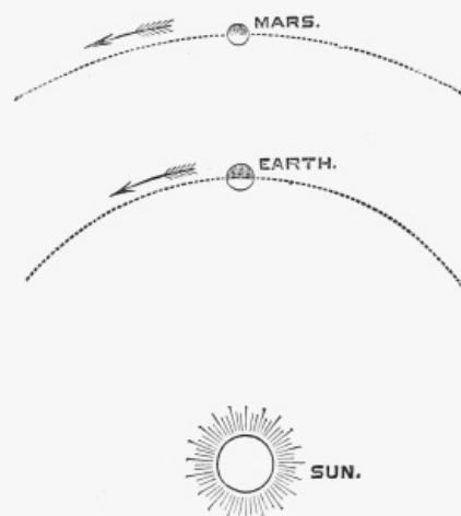
EXPLANATION OF PLANETARY MOVEMENTS.
