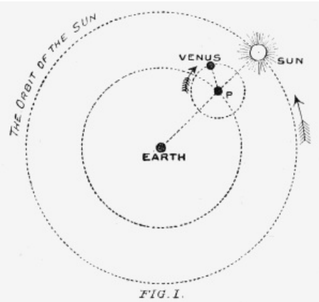
FIG. 1. PTOLEMY'S PLANETARY SCHEME.
