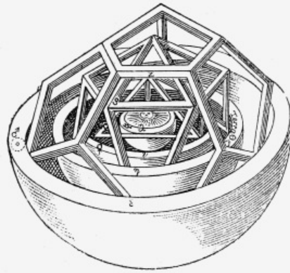
KEPLER'S SYSTEM OF REGULAR SOLIDS.
