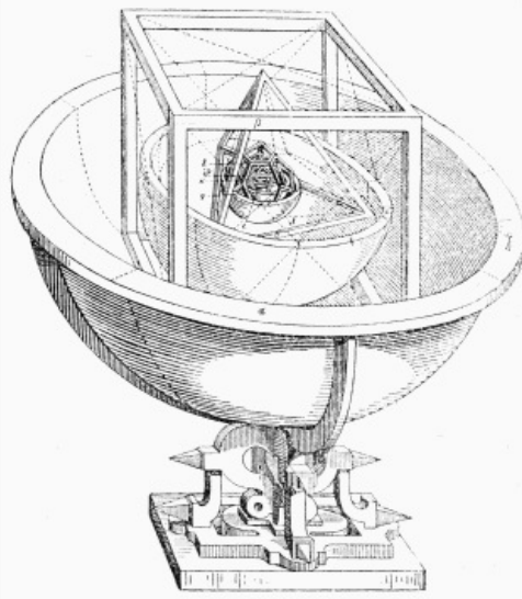
SYMBOLICAL REPRESENTATION OF THE PLANETARY SYSTEM.
