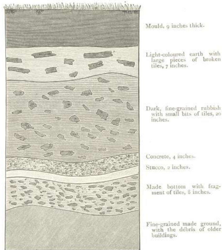
FIG. 12.—Section in the centre of the Basilica at Silchester.
