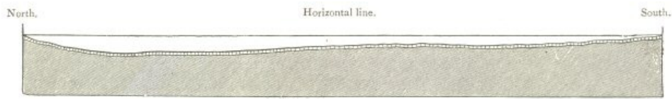
FIG. 13.—Section of the subsided floor of a room, paved with tesserae, at Silchester. Scale \frac{1}{16} .
