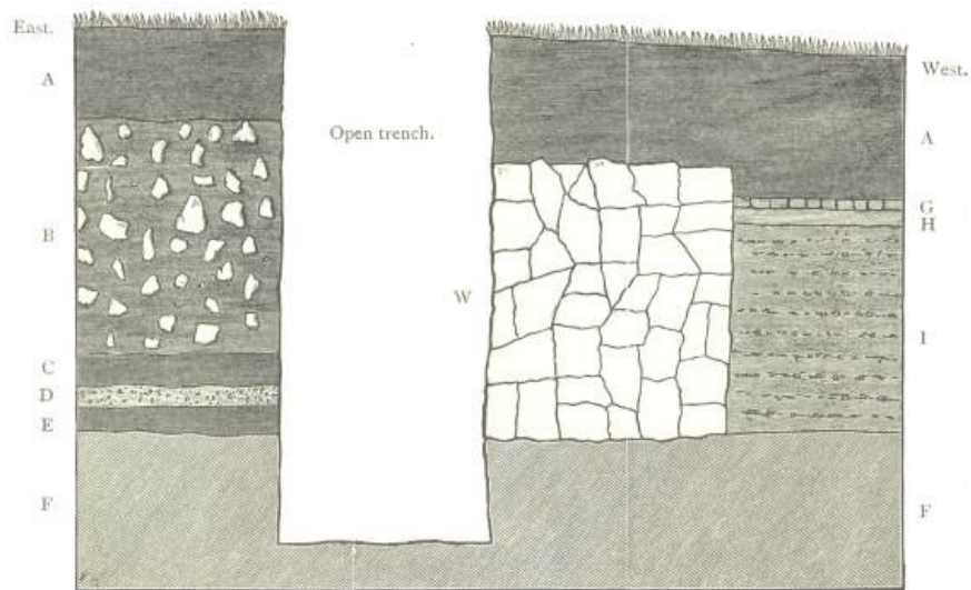
FIG. 8. —Section through the foundations of a buried Roman villa at Abinger. A A, vegetable mould; B, dark earth full of stones, 13 inches in thickness; C, black mould; D, broken mortar; E, black mould; F F, undisturbed sub-soil; G, tesserae; H, concrete; I, nature unknown; W, buried wall. [To face p. 168.]
