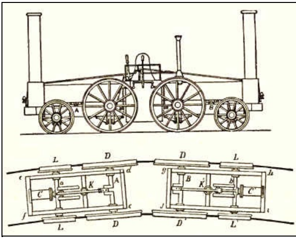
The "South Carolina," 1831, and plan of its running gear.
