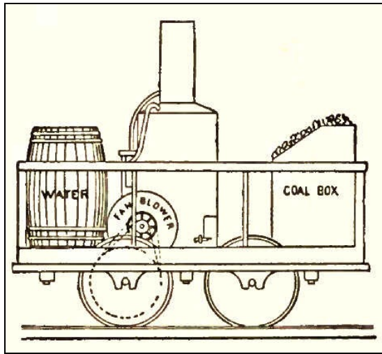
Peter Cooper's Locomotive, 1829.
