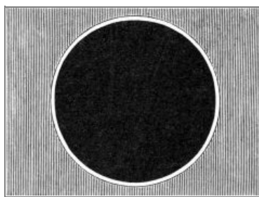
FIG. 4.—ANNULAR ECLIPSE OF THE SUN.
