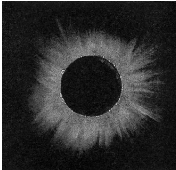
FIG. 10.—CORONA OF 1882. (SUN-SPOT MAXIMUM.)
