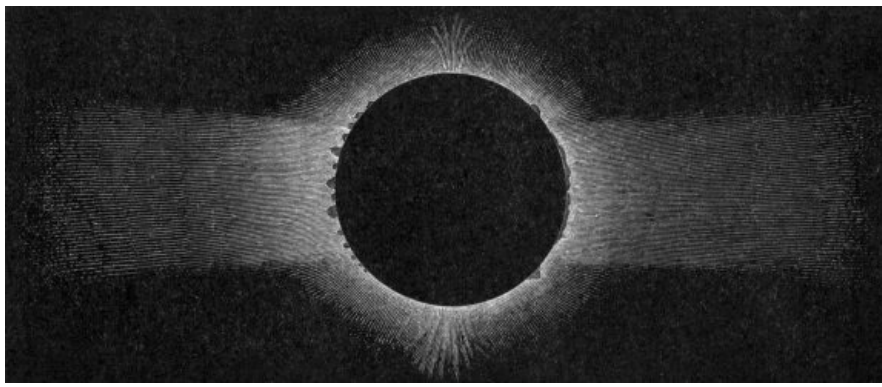
FIG. 11.—CORONA OF 1867. (SUN-SPOT MINIMUM.)
