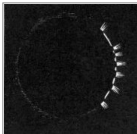
FIG. 8.—BRUSHES OF LIGHT.
