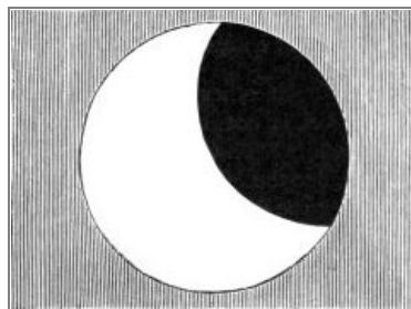
FIG. 5.—PARTIAL ECLIPSE OF THE SUN.
