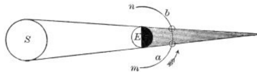
FIG. 13.—THEORY OF AN ECLIPSE OF THE MOON.
