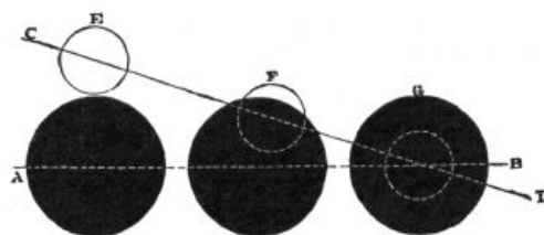
FIG. 14.—CONDITIONS OF ECLIPSES OF THE MOON.
