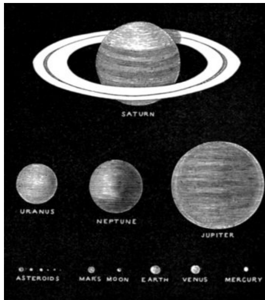
Fig. 5.—Comparative sizes of Planets.
