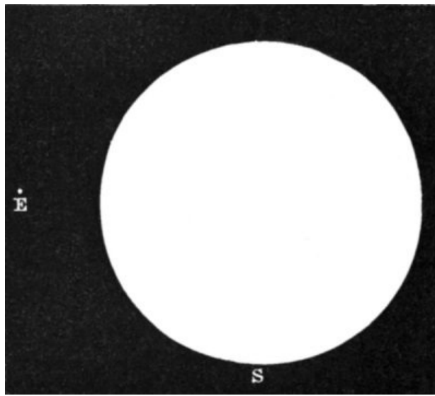
Fig. 4.—Comparative sizes of Earth and Sun.
