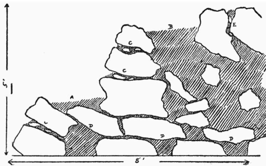
Cross-section of rock garden construction, showing shallow (A) and deep (B) soil pockets; tilting and wedging of rocks (C); bridging (D), and perpendicular crevice soil run (E). Two to three inches of soil between all joints. The lowest rocks are partly buried
