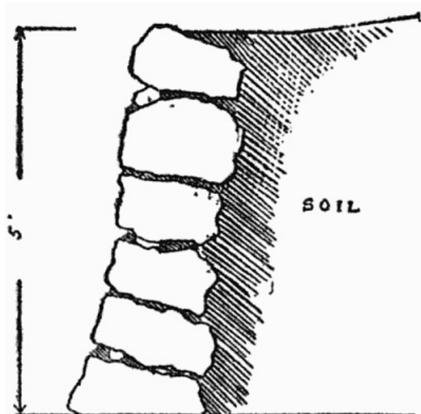
Dry wall for retaining bank. Cross-section,
