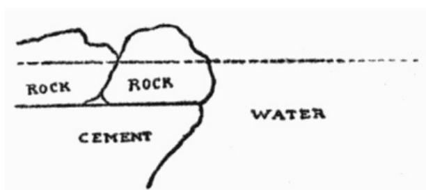
To conceal the cemented bank of a pool or stream, make a shoulder eight inches or so wide and about six inches below the water line. Then place small rocks on the shoulder
