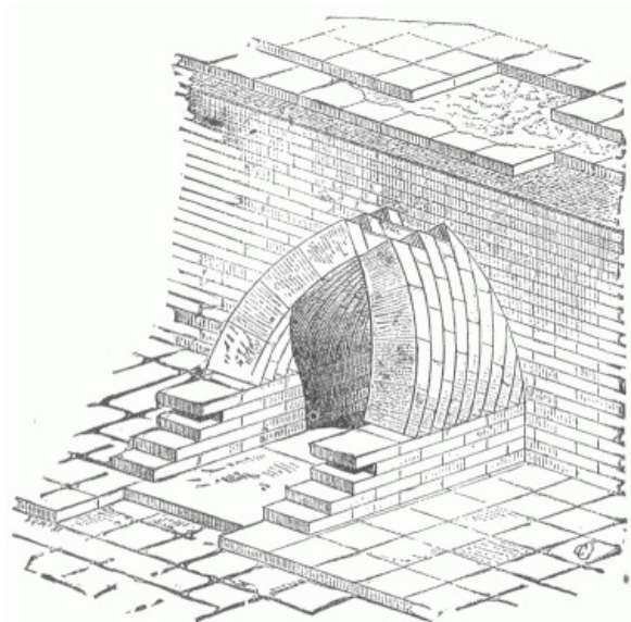
35.—VAULTED DRAIN. (KHORSABAD.)
