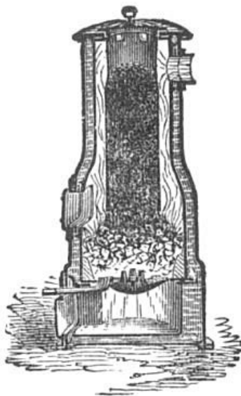
FIG. 6. VERTICAL SECTION.
