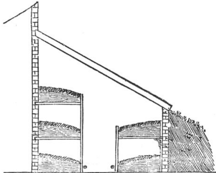
FIG. 7. MUSHROOM HOUSE BUILT AGAINST A NORTH-FACING WALL.
