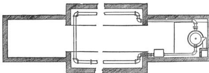
FIG. 4. GROUND PLAN OF THE DOSORIS CELLAR.
