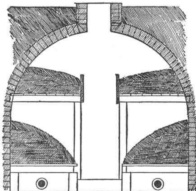
FIG. 3. CROSS-SECTION OF THE DOSORIS MUSHROOM CELLAR.
