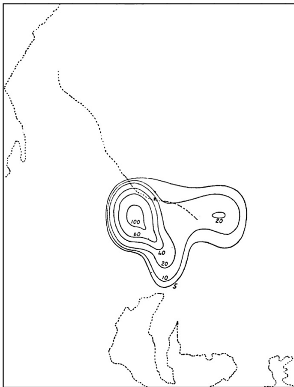
FIG. 56.—Distribution of After-shocks in Space (March-April). ( Davison. )
