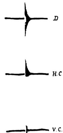
FIG. 21.—Magnetograph records of Andalusian earthquake at Lisbon. ( Fouqué, etc. )
