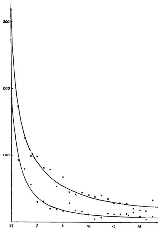
FIG. 51.—Daily frequency of after-shocks at Gifu and Nagoya.
