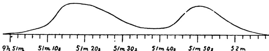
FIG. 26.—Curve of intensity at Charleston. (Dutton.)
