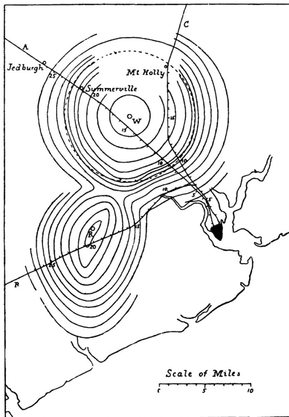
FIG. 29.—Epicentral isoseismal lines of Charleston earthquake according to Major Dutton. (Dutton.)
