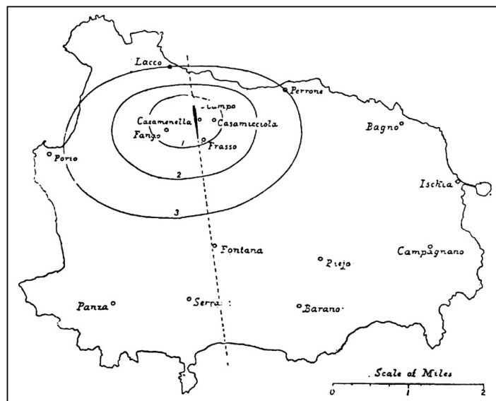
FIG. 15.—Iseismal lines of the Ischian earthquake of 1881. (Johnston-Lavis.)
