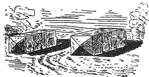
FIG. 6.—Fallen gate-pillars near Saponara. ( Mallet. )
