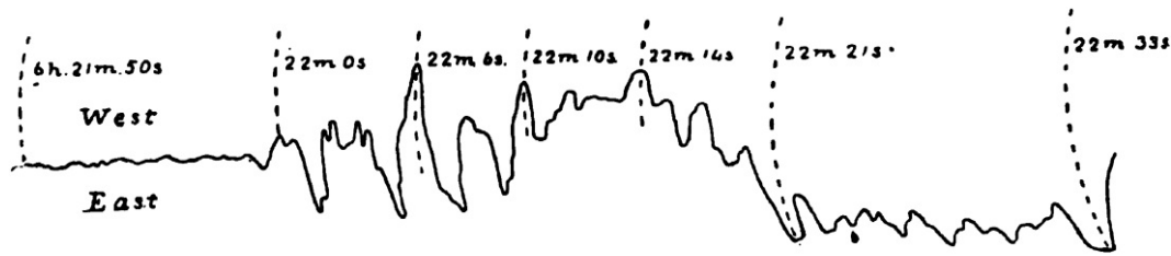
FIG. 36.—Seismographic record of the Riviera earthquake at Moncalieri. ( Denza. )
