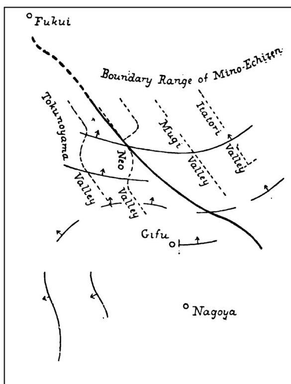
FIG. 42.—General Plan of Geological Structure of Meizoseismal Area. (Koto.)
