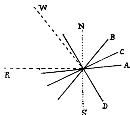
FIG. 30.—Planes of oscillation of stopped pendulum clocks at
