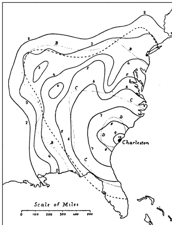
FIG. 25.—Isoseismal lines of Charleston earthquake. ( Dutton, etc. )
