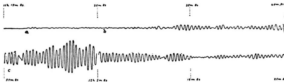
FIG. 71.—Seismographic Record of Indian Earthquake at Rocca di Papa. ( Cancani )
