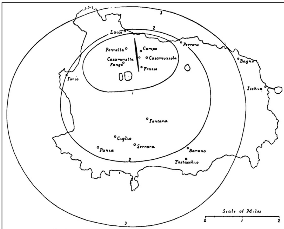
FIG. 16.—Isoseismal lines of the Ischian earthquake of 1883.
