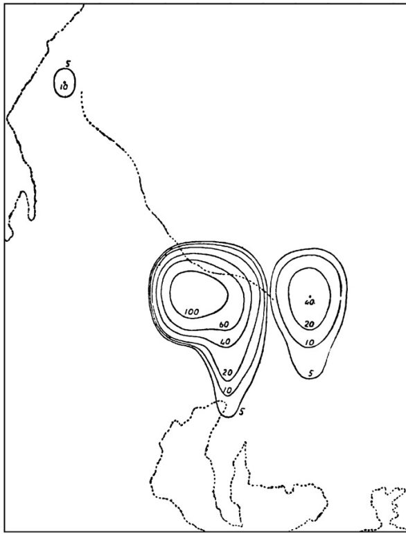
FIG. 55.—Distribution of After-shocks in Space (January-February, 1892). ( Davison. )
