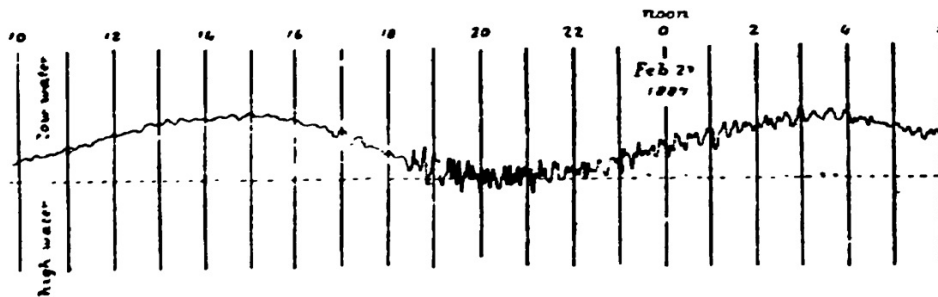
FIG. 39.—Record of tide-gauge at Genoa. (Issel.)
