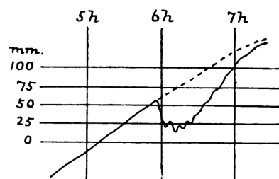
FIG. 38.—Record of tide-gauge at Nice. (Issel.)
