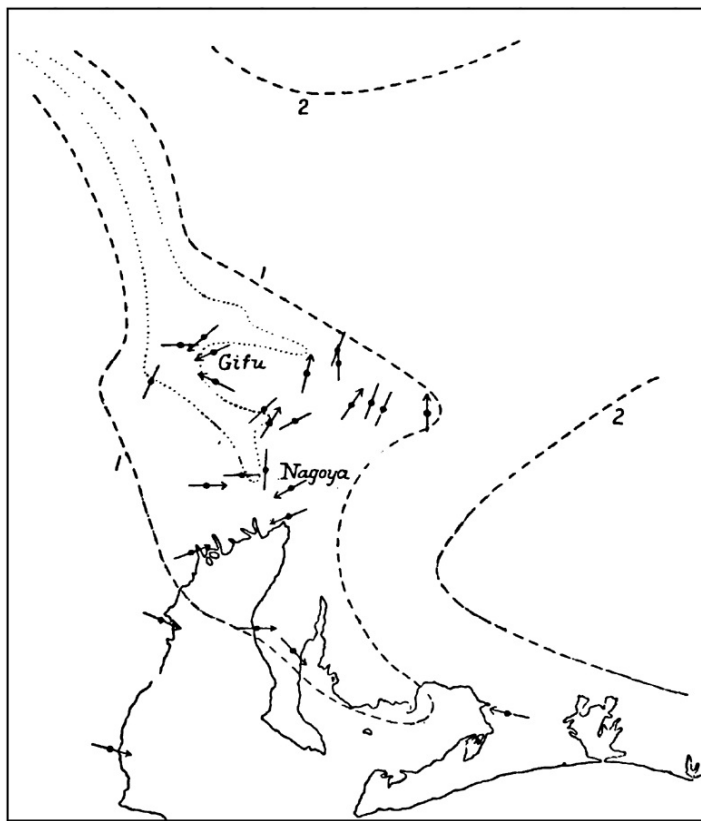
FIG. 44.—Map of Mean Directions of Shock and Ioseismal Lines in Central District. ( Omori )
