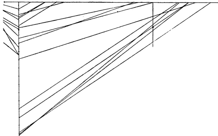
FIG. 17.—Diagram of wave-paths at seismic vertical of Ischian earthquake of 1883. ( Johnston-Lavis. )
