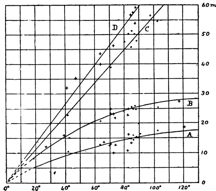
FIG. 80.—Time-curves of principal epochs of earthquake-waves of distant origin. ( Oldham. )
