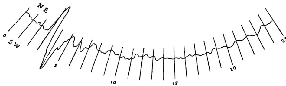
FIG. 79.—Seismographic Record of Tokio Earthquake of 1894. ( Omori )
