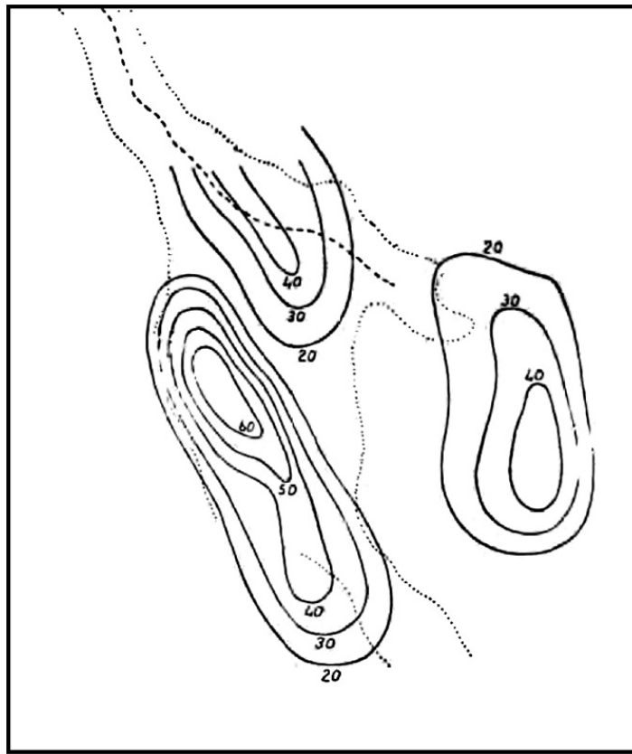
FIG. 58.—Distribution of Audible After-shocks in Space (November 1891-December 1892). ( Davison. )
