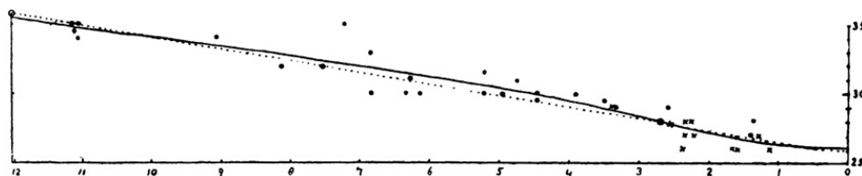
FIG. 70.—Time-curve of Indian earthquake. ( Oldham. )
