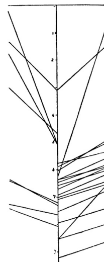
FIG. 13.—Diagram of wave-paths at seismic vertical of Neapolitan earthquake. (Mallet.)
