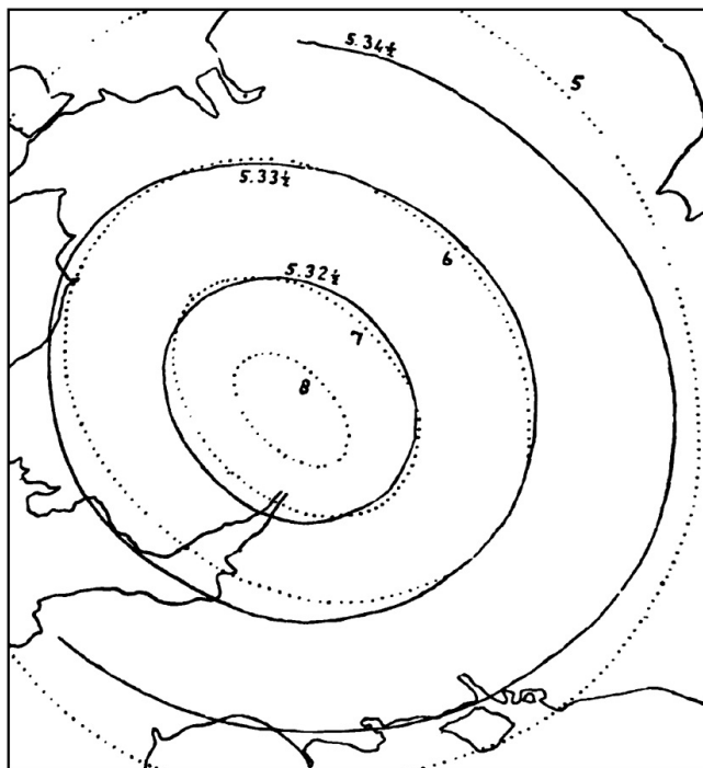
FIG. 62.—Coseismal lines of the Hereford earthquake. ( Davison. )
