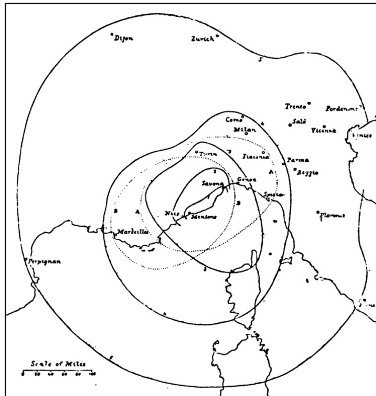
FIG. 33.—Isoseismal lines of the Riviera earthquake. (Mercalli.)
