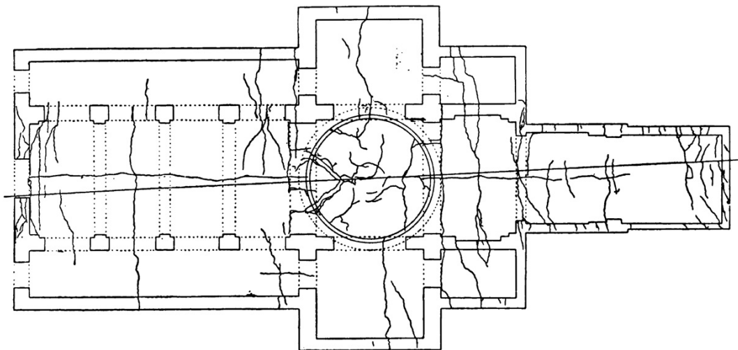
FIG. 5.—Plan of Cathedral Church at Potenza. ( Mallet. )
