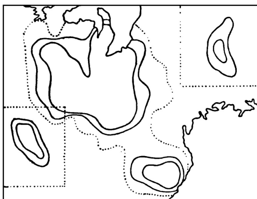
FIG. 59.—Map of Adjoining Regions in which
