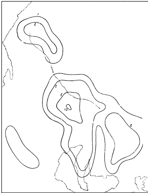
FIG. 53.—Distribution of preliminary Shocks in Space. ( Davison. )
