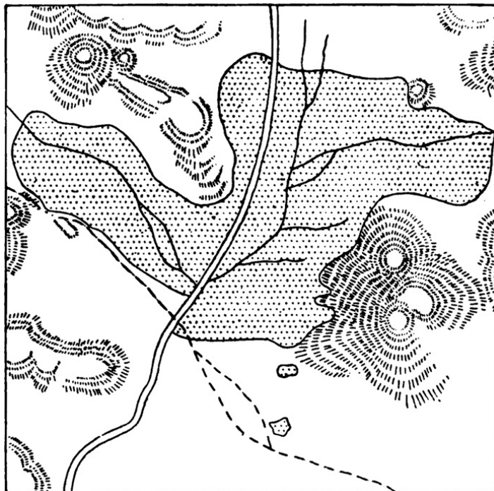
FIG. 49.—Map of Swamp formed by stoppage of River Toba by Fault-scarp. ( Koto. )
