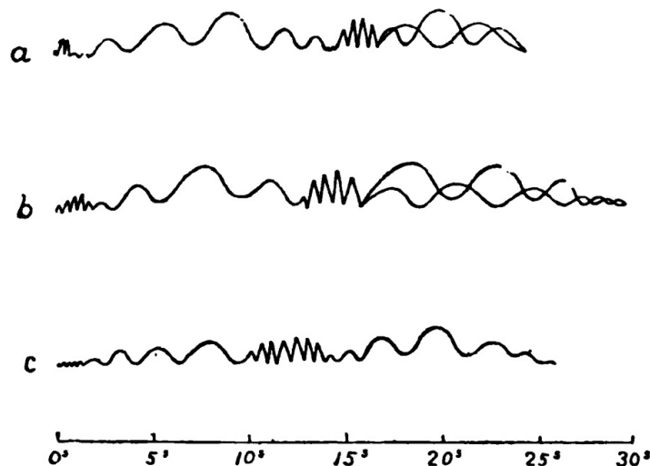
FIG. 35.—Nature of shock of Riviera earthquake. ( Taramelli and Mercalli. )
