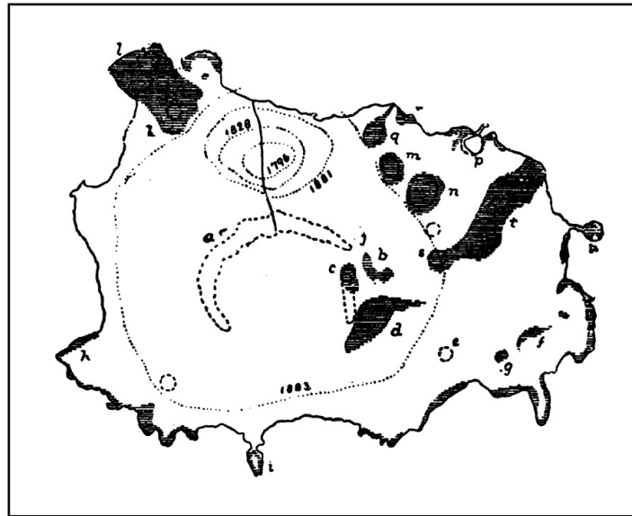
FIG. 14.—Geological sketch-map of Ischia. (Mercalli.) [21]
