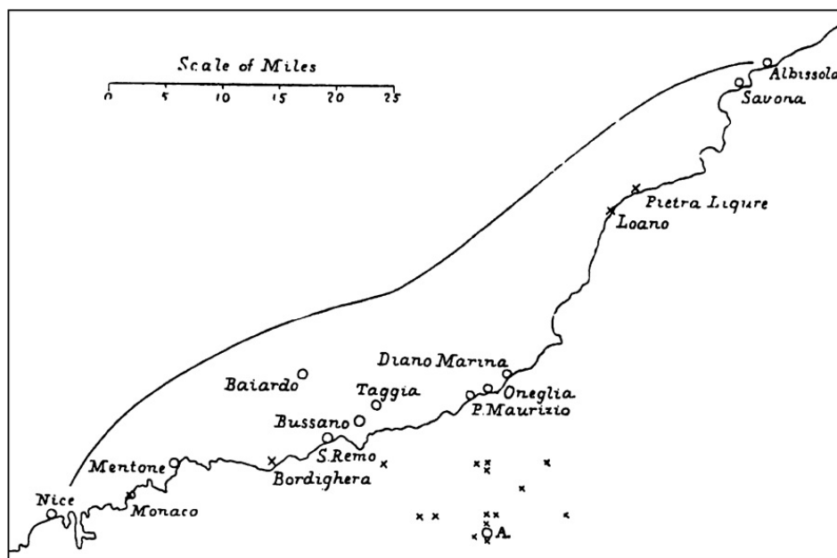
FIG. 34.—Meizoseismal area of the Riviera earthquake. ( Taramelli and Mercalli. )
