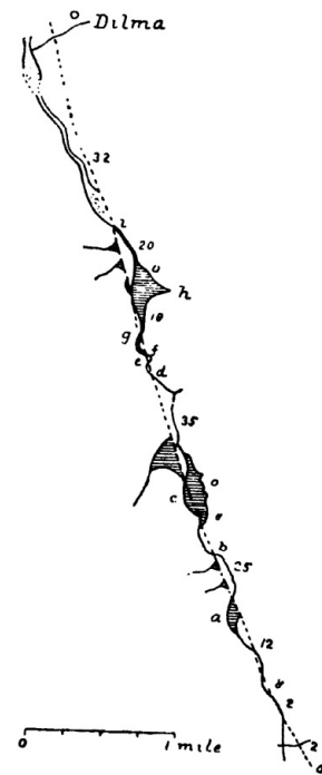
FIG. 76.—Plan of Chedrang fault. (Oldham.)
