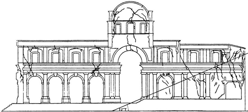
FIG. 12.—Vertical section of Cathedral Church at Potenza. (Mallet.)
