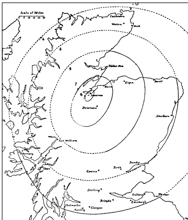
FIG. 65.—Isoseismal lines of the Inverness earthquake. (Davison.)
