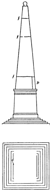
FIG. 74.—Twisting of monument at Chhatak. (Oldham.)
