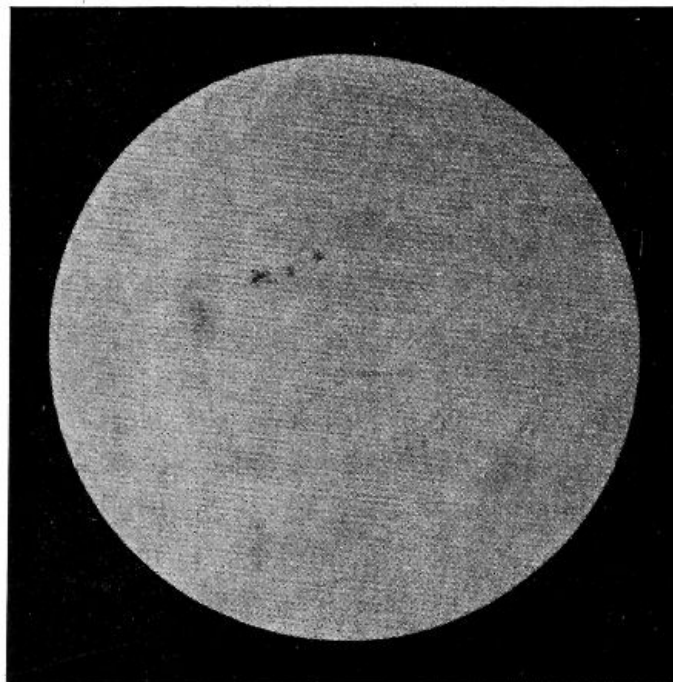
FIG. 29.—Direct photograph of the Sun.
