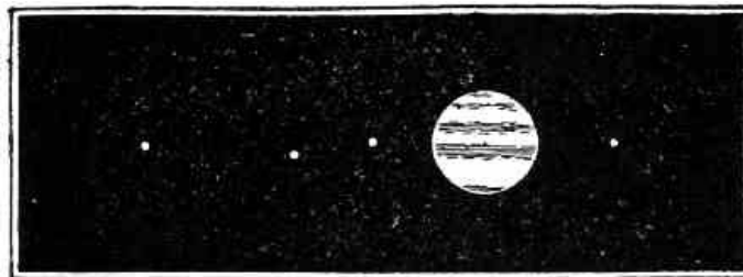
FIG. 46.—Jupiter and his four principal satellites.
