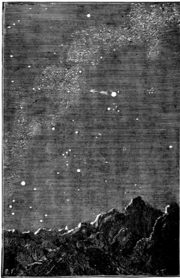
FIG. 35.—The Earth viewed from Mercury.
