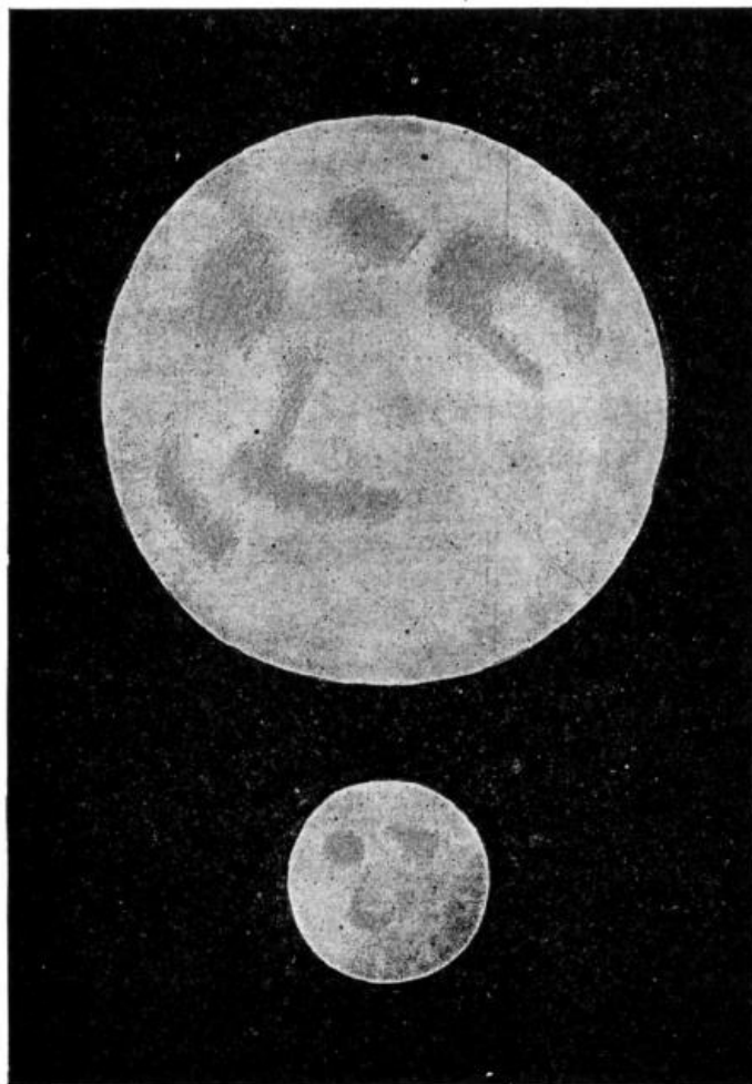
FIG. 65.—The Moon viewed with the unaided eye.
