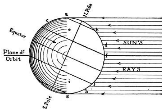
FIG. 61.—Inclination of the Earth.
