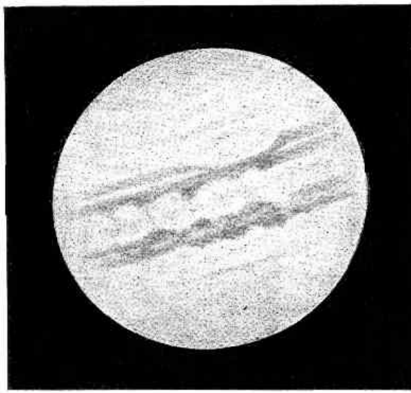
FIG. 45.—Telescopic aspect of Jupiter.
