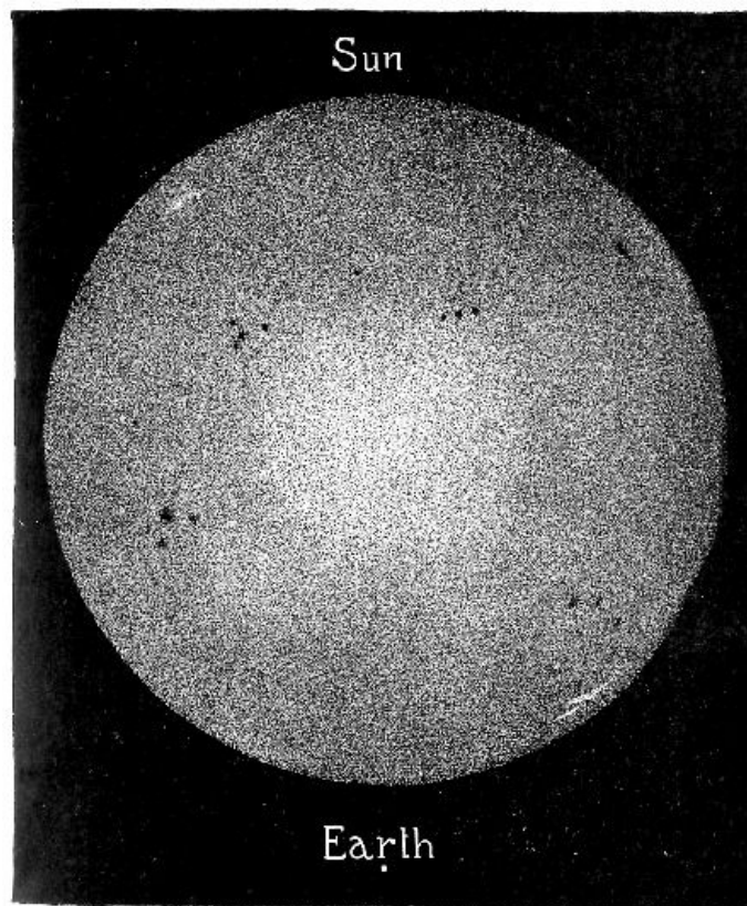
FIG. 28.—Comparative sizes of the Sun and Earth.
