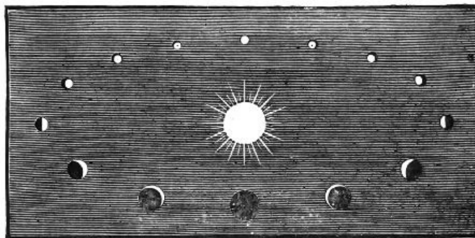
FIG. 37.—Successive phases of Venus.
