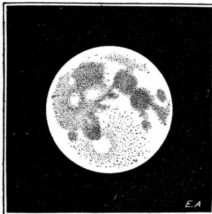
FIG. 66.—The Man's head in the Moon.
