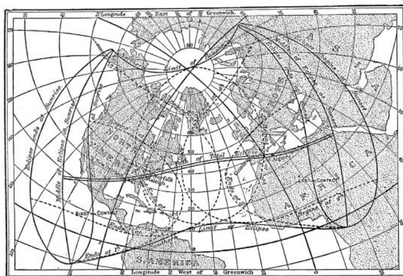
FIG. 77.—The path of the Eclipse of May 28, 1900.
