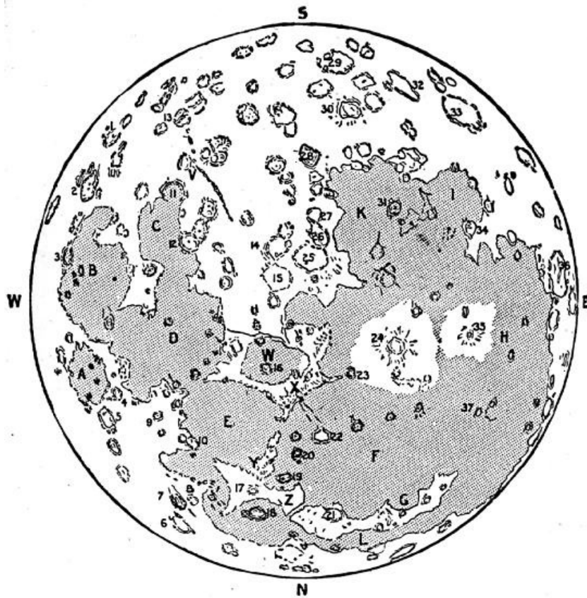
FIG. 71.—Map of the Moon. (From Fowler's "Telescopic Astronomy.")
