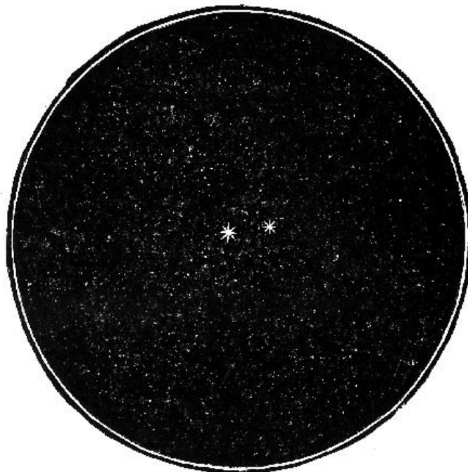
FIG. 17.—The double star Mizar.
