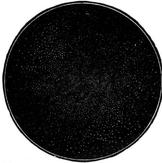
FIG. 22.—The Star-Cluster in the Centaur.
