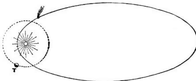
FIG. 52.—The orbit of a Periodic Comet.
