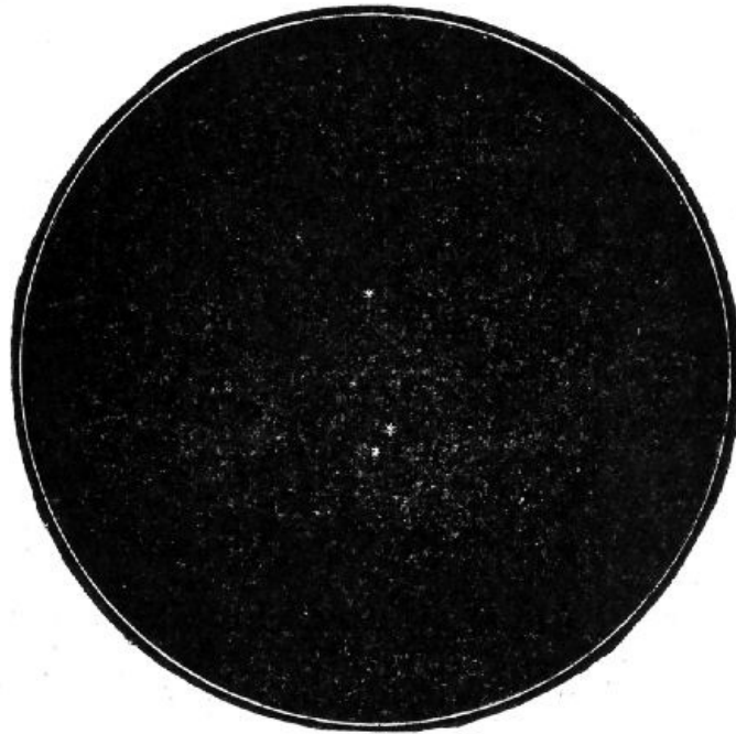
FIG. 18.—Triple star \zeta in Cancer.
