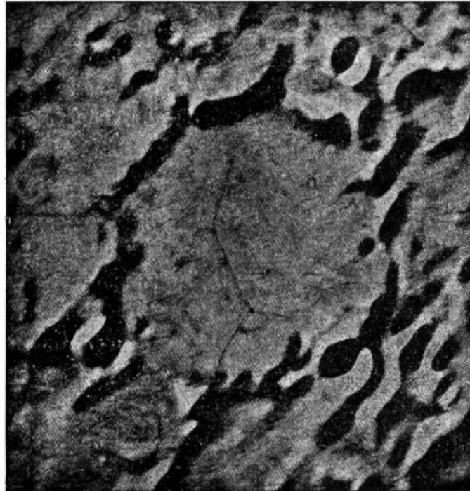
FIG. 73.—Flammarion's Lunar Ring.
