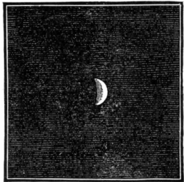
FIG. 34.—Mercury near quadrature.
