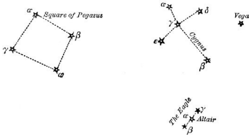
FIG. 9.—The Swan, Vega, the Eagle.
