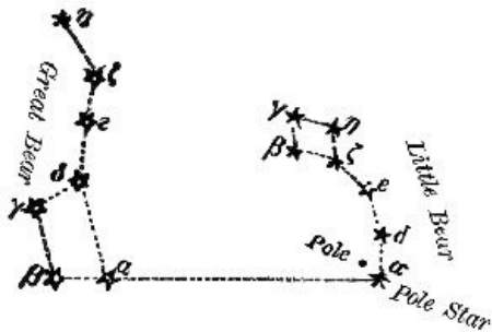
FIG. 4.—To find the Pole-Star.
