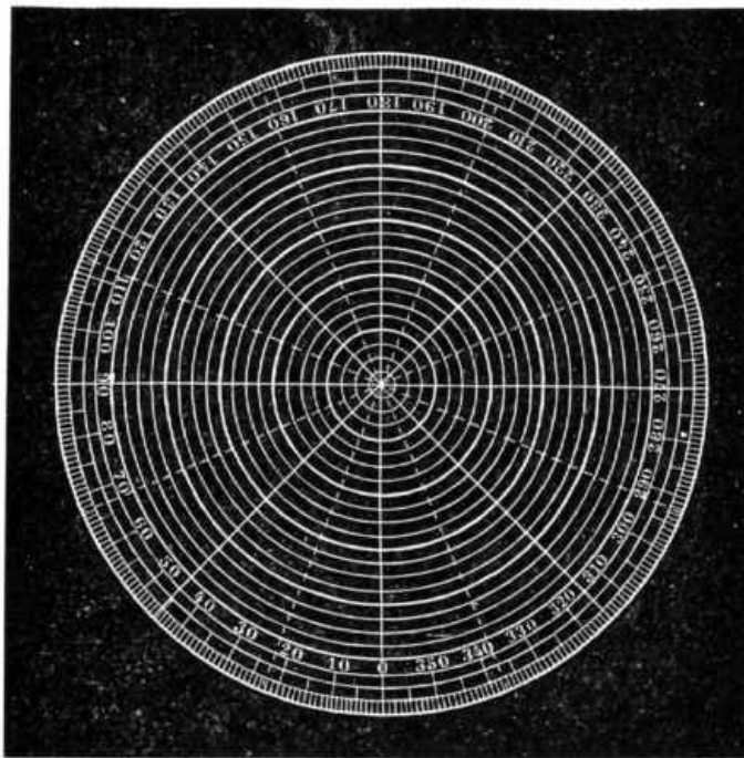
FIG. 81.—Division of the Circumference into 360 degrees.
