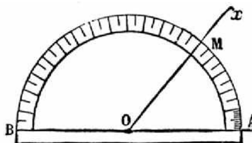
FIG. 80.—Measurement of Angles.
