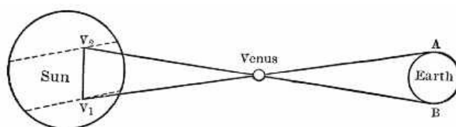
FIG. 83.—Measurement of the distance of the Sun.
