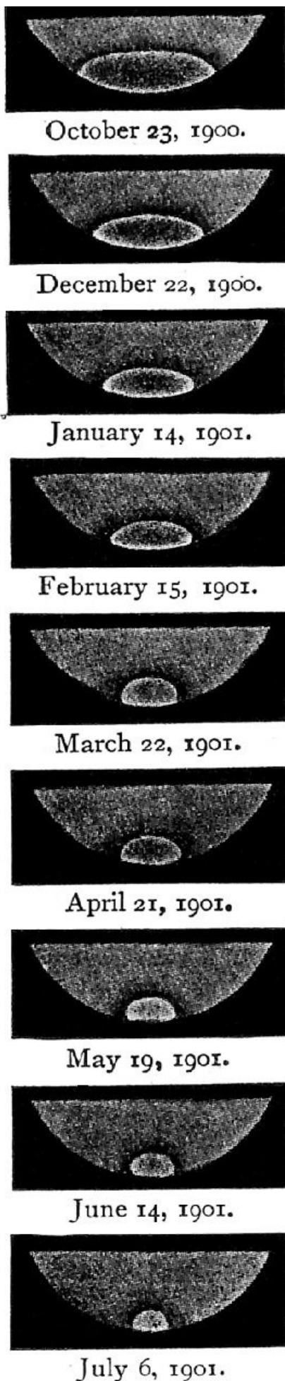
FIG. 40.—Diminution of the polar snows of Mars during the summer.
