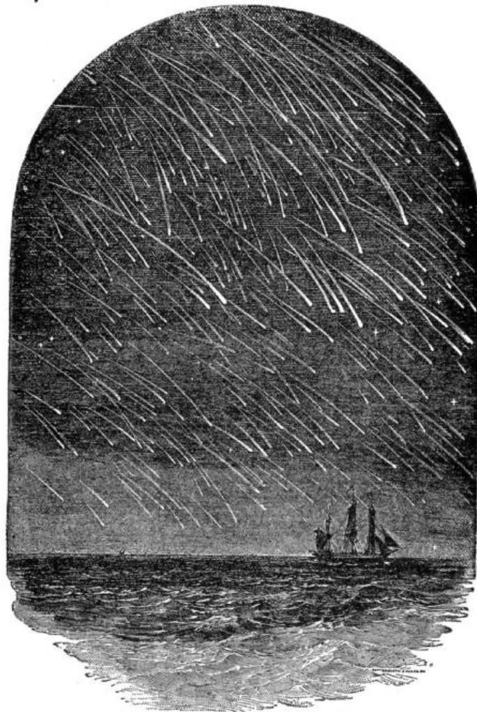
FIG. 55.—Shooting Stars of November 12, 1799. From a contemporary drawing.
