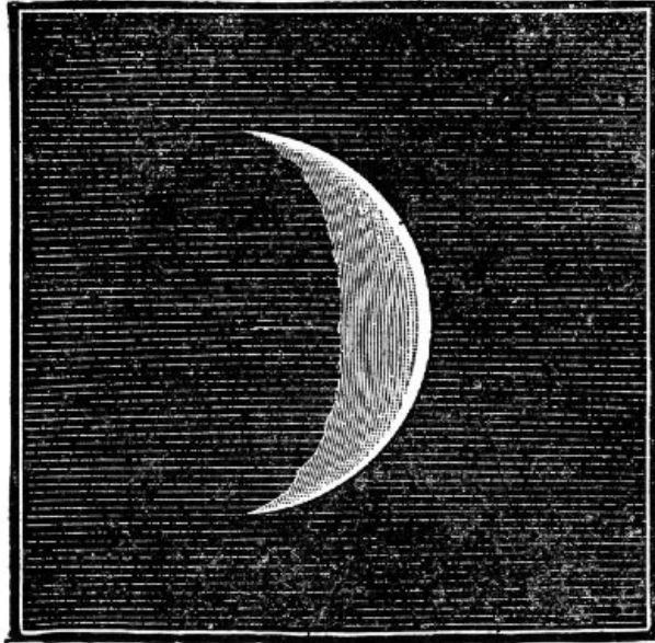
FIG. 38.—Venus at greatest brilliancy.
