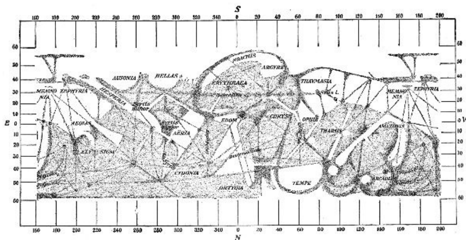
FIG. 43.—Chart of Mars.
