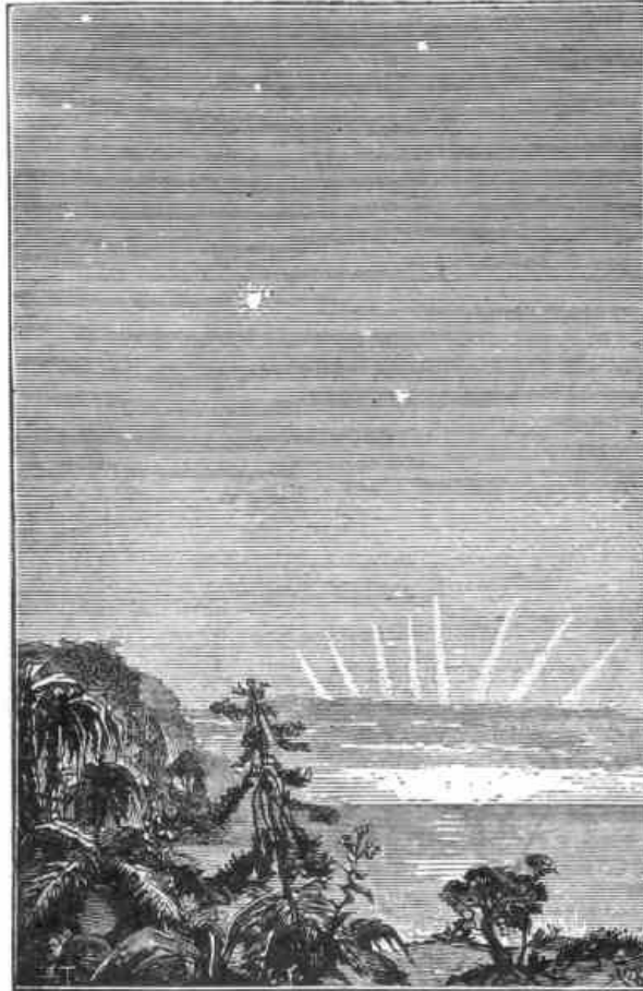
FIG. 44.—The Earth viewed from Mars.
