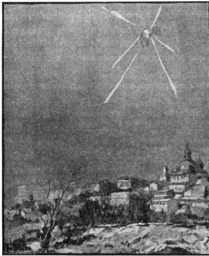
FIG. 57.—Explosion of a Fire-Ball above Madrid, February 10, 1896.
