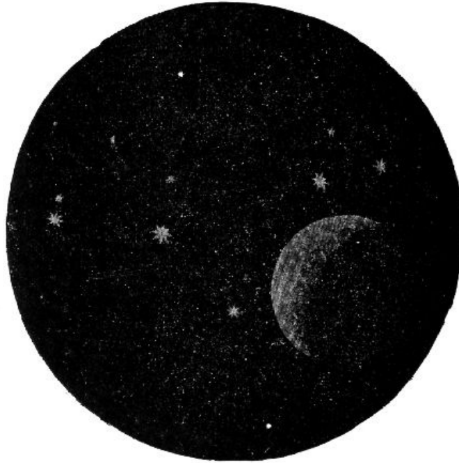
FIG. 26.—Occultation of the Pleiades by the Moon.
