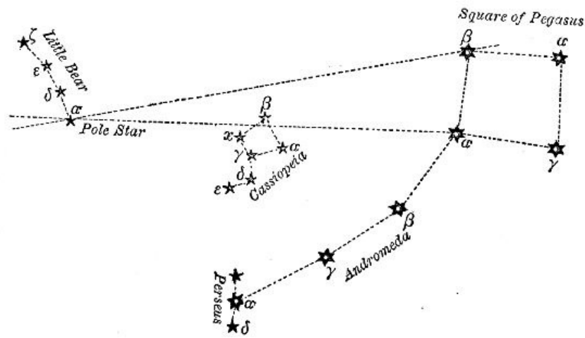
FIG. 6.—To Find Pegasus and Andromeda.
