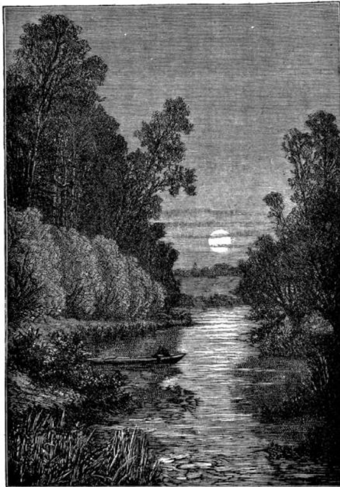
FIG. 64.—The Full Moon slowly rises.
