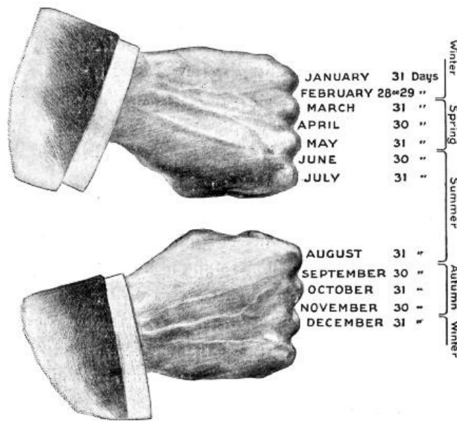
FIG. 63.—To find the long and short months.
