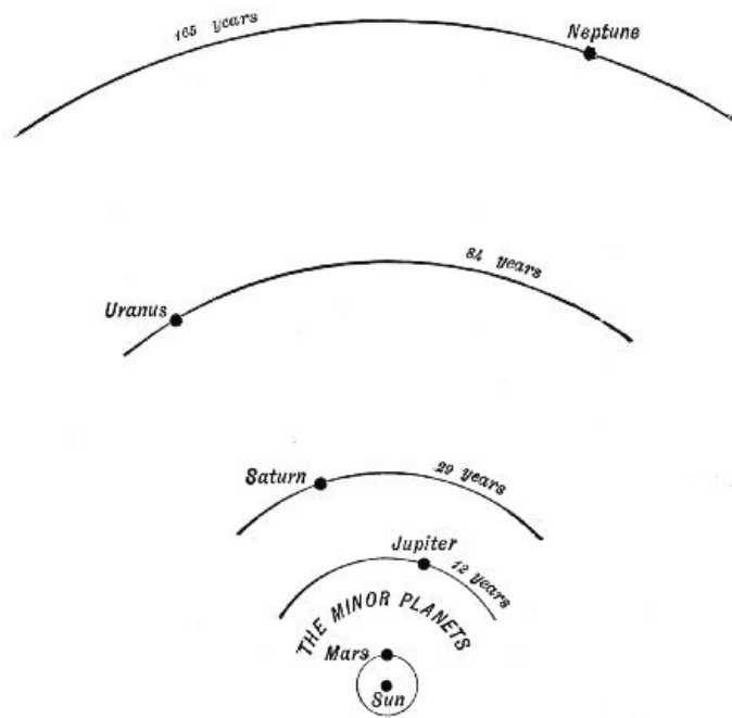
FIG. 33.—Orbits of the four Planets farthest from the Sun.
