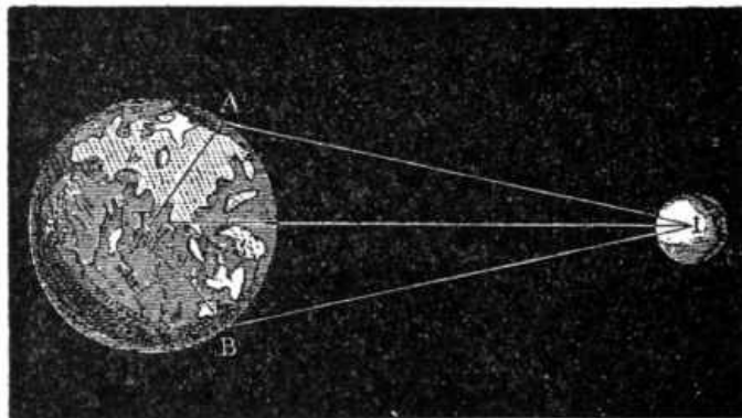
FIG. 82.—Measurement of the distance of the Moon.
