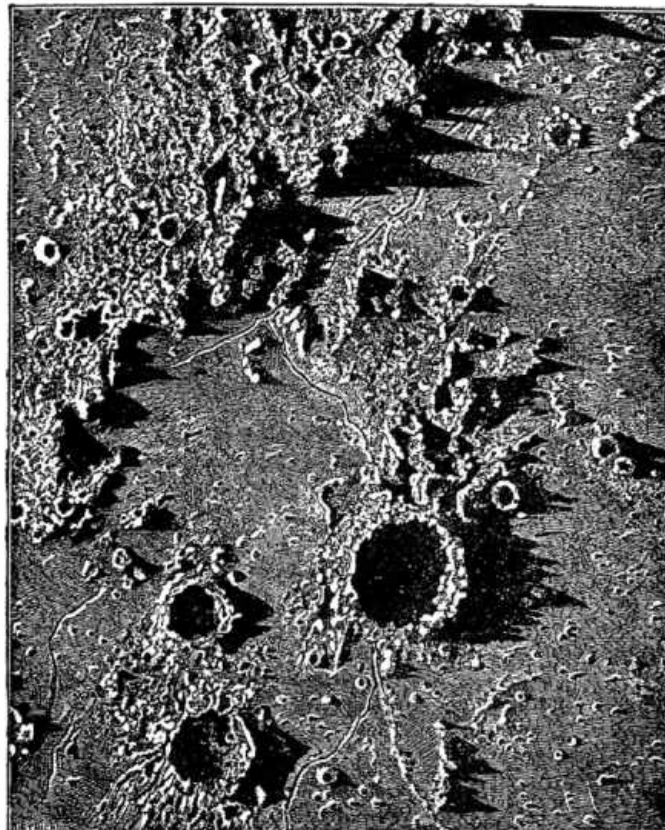
FIG. 72.—The Lunar Apennines.
