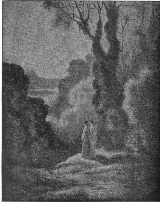
FIG. 36.—The Evening Star.
