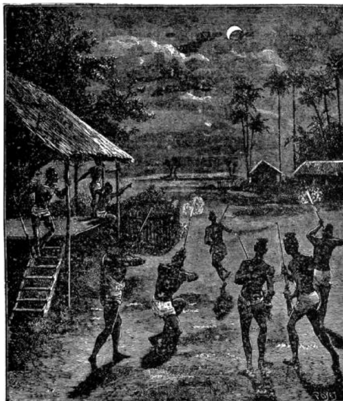
FIG. 76.—Eclipse of the Moon at Laos (February 27, 1877).
