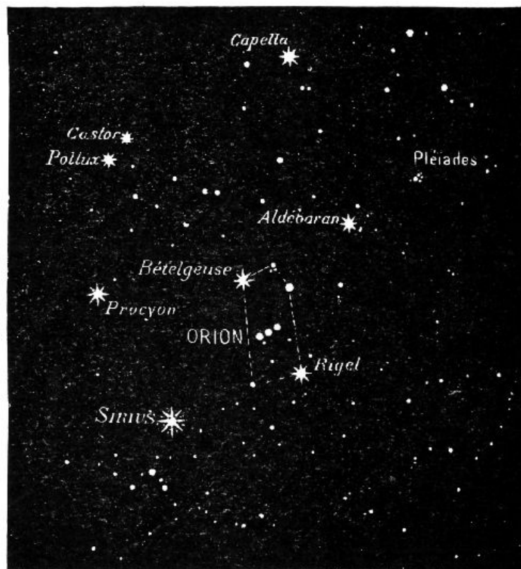
FIG. 12.—Orion and his celestial companions.
