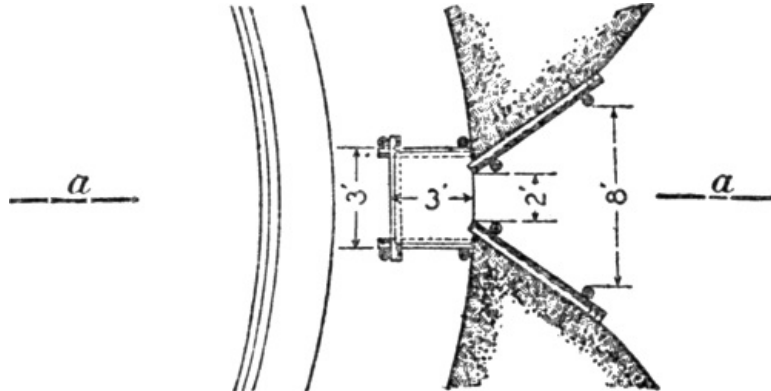
Machine Gun Emplacement: Plan with Cover Removed
