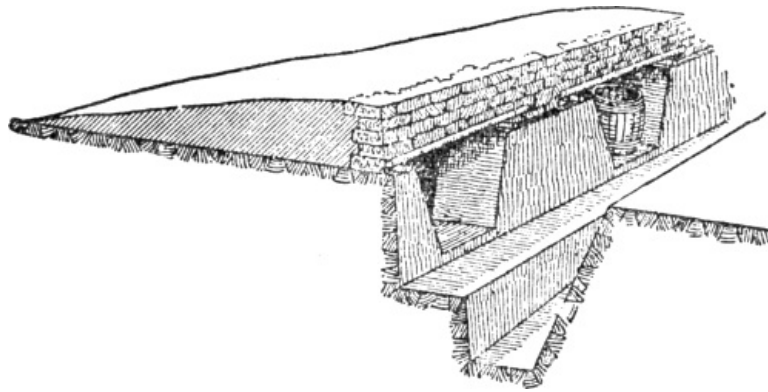
Fig. 18 Store Recesses for Water, Hand-Grenades, Reserve Ammunition, Machine Guns, Range Finders, Blankets, etc. (From Field Entrenchments—Solano.)
