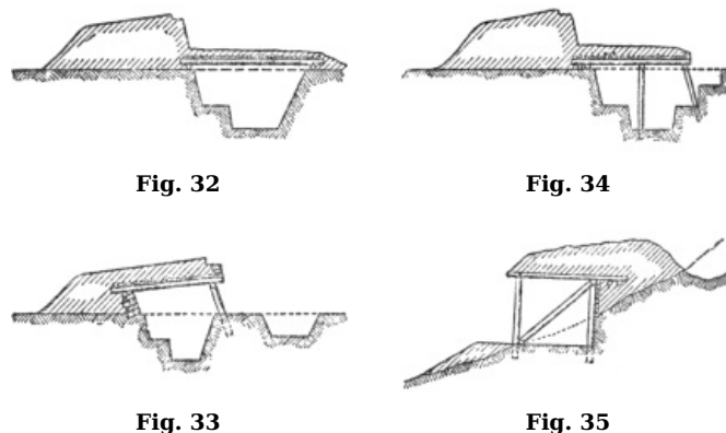
Types of overhead cover.
