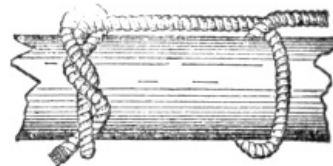
Fig. 29 Timber hitch and half hitch
