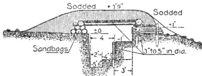
Machine Gun Emplacement: Section aa
