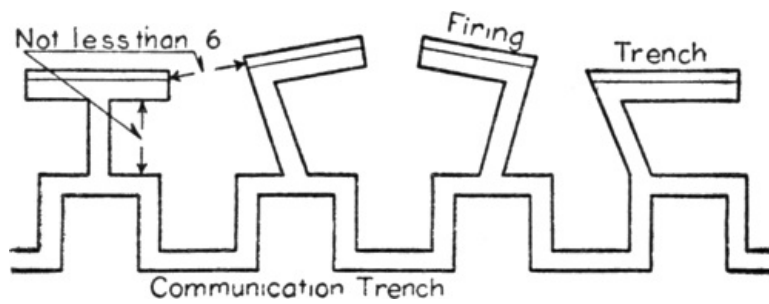
Communication Trenches in rear of Firing Trenches
