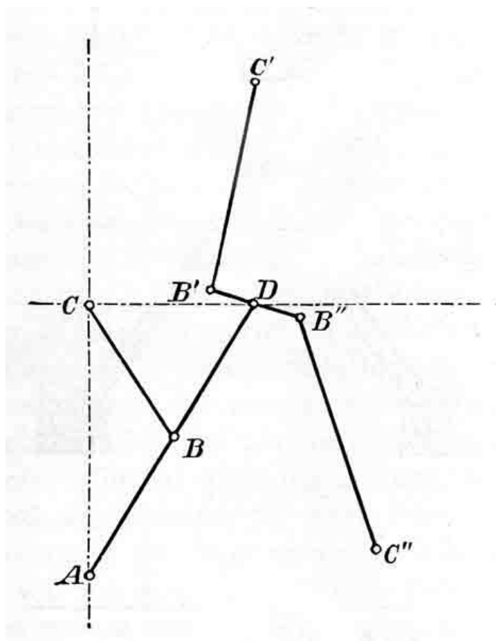
Figure 20.—Chebyshev's combination (about 1867) of Watt's and Evans' linkages to reduce errors
