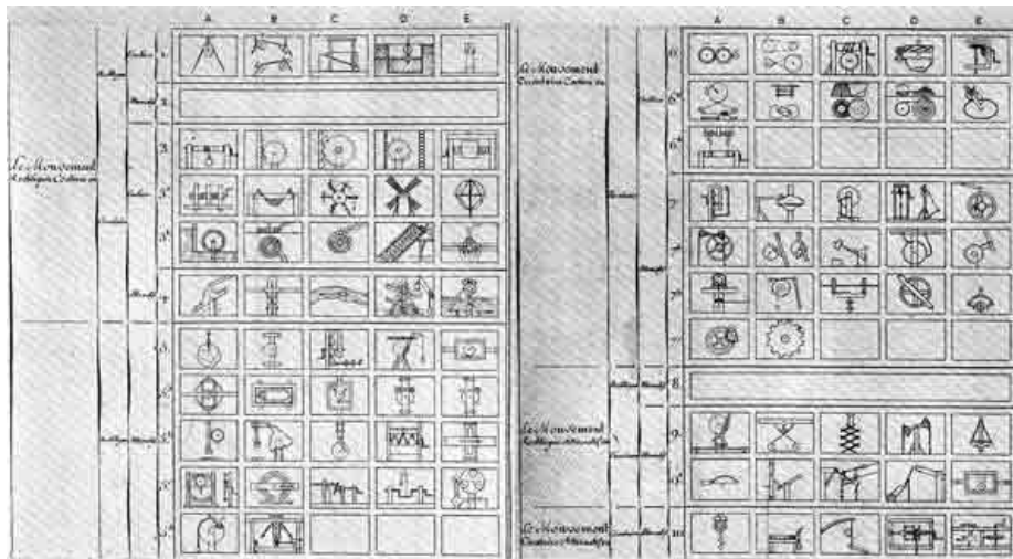
Figure 28.—Hachette's synoptical chart of elementary mechanisms, 1808. This was the first of
