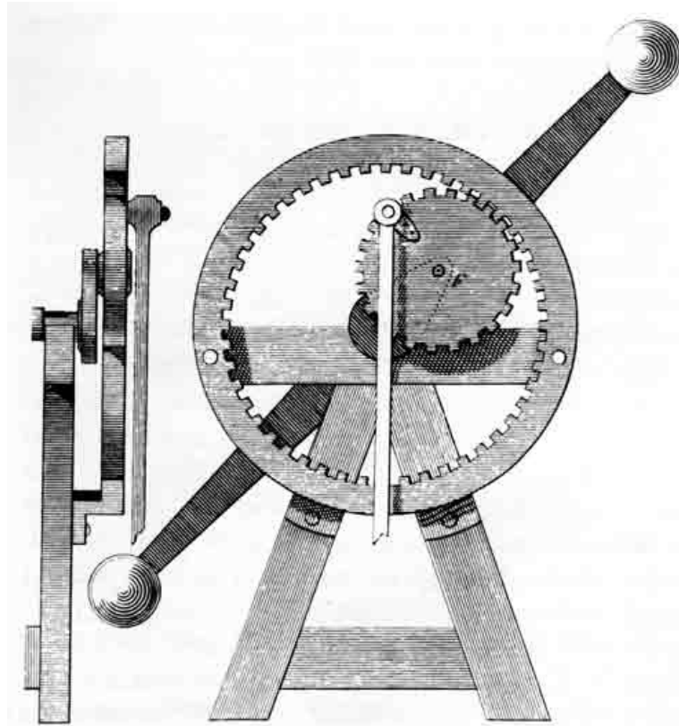
Figure 13.—James White's hypocycloidal straight-line mechanism, about 1800. The fly-weights (at the ends of the diagonal arm) functioned as a flywheel. From James White, A New Century of Inventions (Manchester, 1822, pl. 7).
