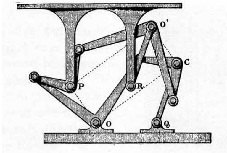
Figure 26.—Sylvester-Kempe translating linkage, 1877. The upper and lower plates remain parallel and equidistant. From A. B. Kempe, How to Draw a Straight Line (London, 1877, p. 37).
