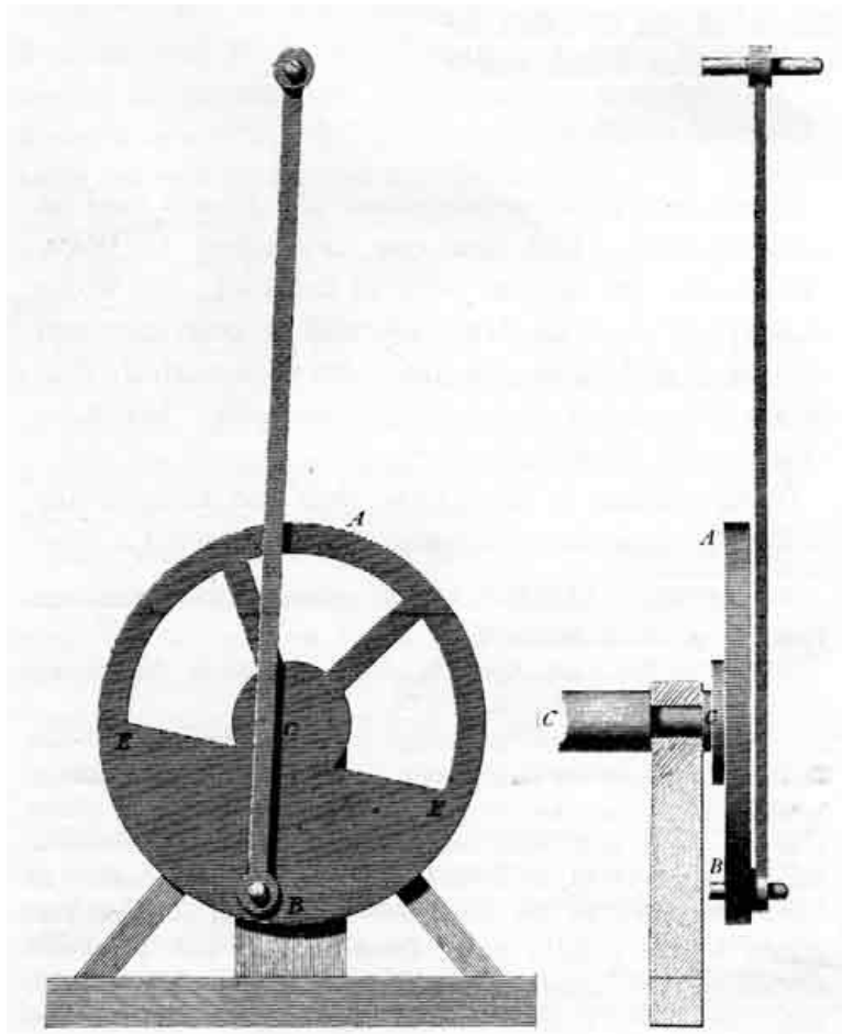
(b) Counterweighted crank wheel.
