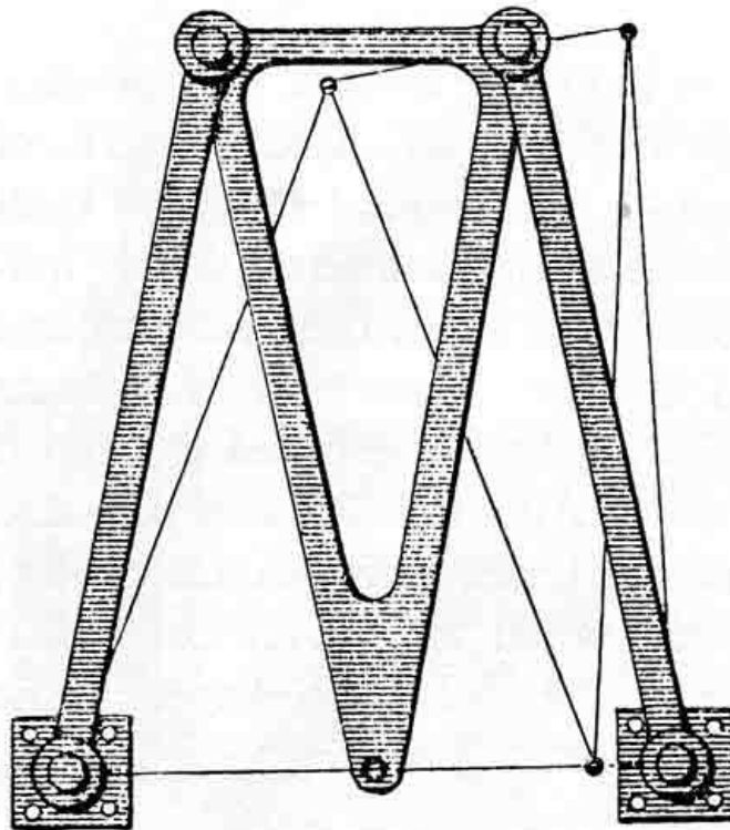
Figure 17.—Straight-line linkage (before 1841) attributed to Richard Roberts by Robert Willis. From A. B. Kempe, How to Draw a Straight Line (London, 1877, p. 10).
