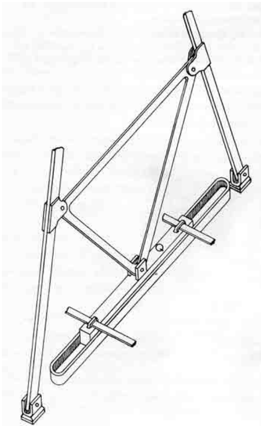
Figure 18.—Machine for sawing off pilings under water, about 1760, designed by De Voglie. The Roberts linkage operates the bar ( Q in detailed sketch on left) at the rear of the machine below the operators. The significance of the linkage apparently was not generally recognized. A similar machine depicted in Diderot's Encyclopédie , published several years later, did not employ the straight-line linkage. From Pierre Patte, Memoirs sur les objets plus importants de l'architecture (Paris, 1769, pl. 11).
