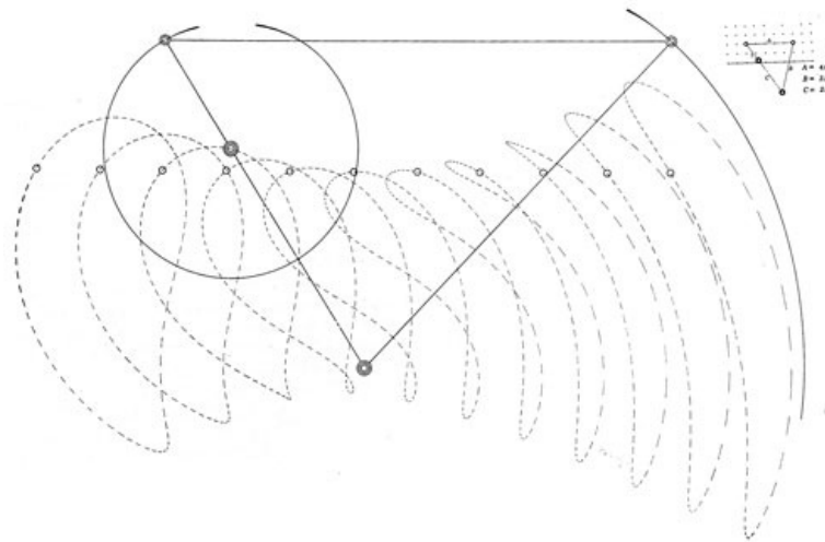
Figure 45.—Paths of 11 points on the coupler (horizontal) link are plotted through one cycle. Dashes indicate equal time intervals. From John A. Hrones and G. L. Nelson, Analysis of the Four Bar Linkage (New York, 1951, p. 635).
