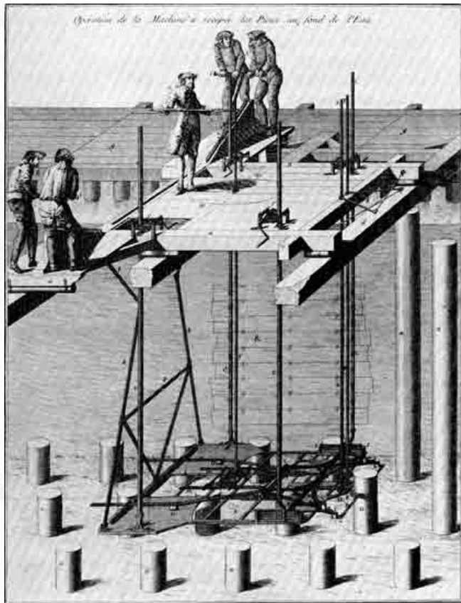
Figure 18.—Machine for sawing off pilings under water, about 1760, designed by De Voglie. The Roberts linkage operates the bar ( Q in detailed sketch on left) at the rear of the machine below the operators. The significance of the linkage apparently was not generally recognized. A similar machine depicted in Diderot's Encyclopédie , published several years later, did not employ the straight-line linkage. From Pierre Patte, Memoirs sur les objets plus importants de l'architecture (Paris, 1769, pl. 11).
