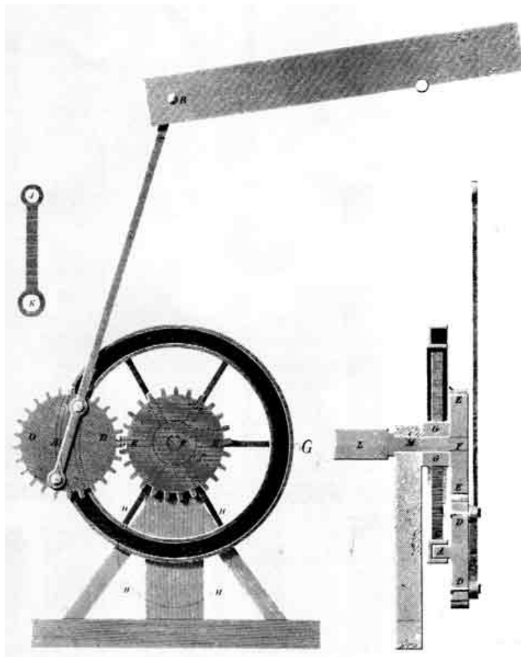
(e) Sun-and-planet gearing. This is the idea actually employed in Boulton and Watt engines. As the optional link JK held the gearwheel centers always equidistant, the annular guide G was not used.
