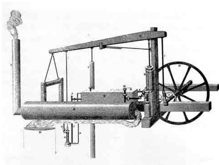
Figure 15.—Oliver Evans' "Columbian" engine, 1813, showing the Evans, or "grasshopper," straight-line linkage. From Emporium of Arts and Sciences (new ser., vol. 2, no. 3, April 1814, pl. opposite p. 380).
