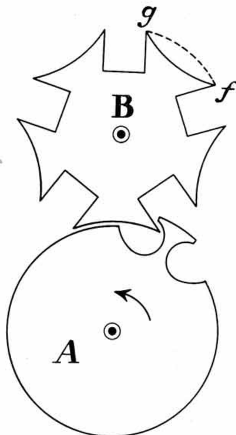
Figure 40.—Geneva stop mechanism first used in Geneva watches to prevent overwinding. The starwheel B had one convex surface ( g-f , dotted) so the wheel could be turned less than a full revolution. After Robert Willis, Principles of Mechanism (London, 1841, p. 266).
