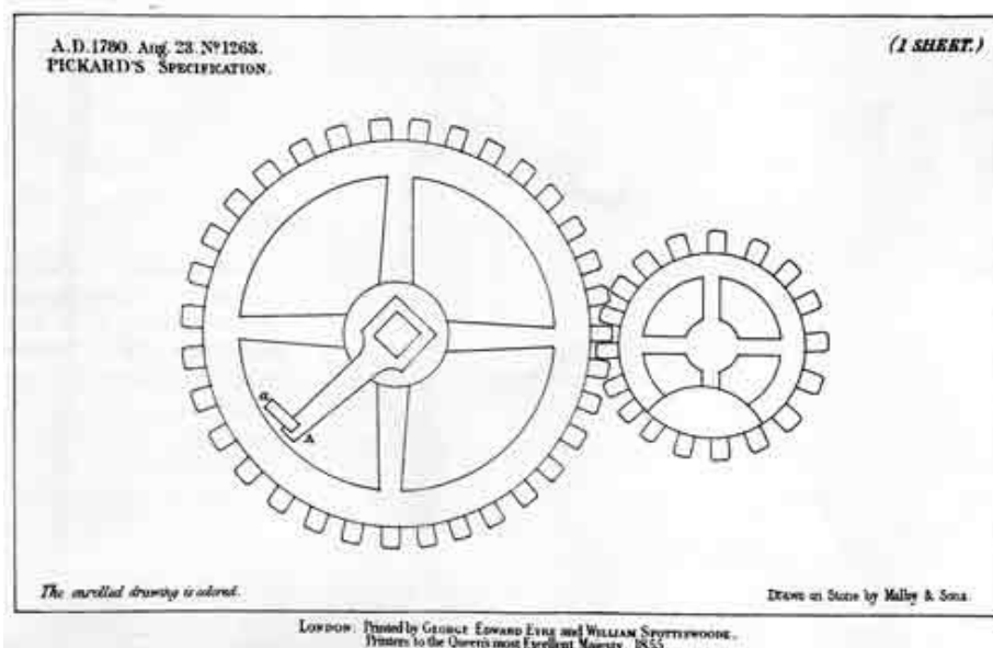
Figure 6.—One of the steam engine "Crank Patents" that hindered James Watt's progress. This patent, granted to James Pickard in 1780, claimed only the arrangement of counterweights, not the crank. The crank pin to which the connecting rod was attached is at Aa. From British Patent 1263, August 23, 1780.
