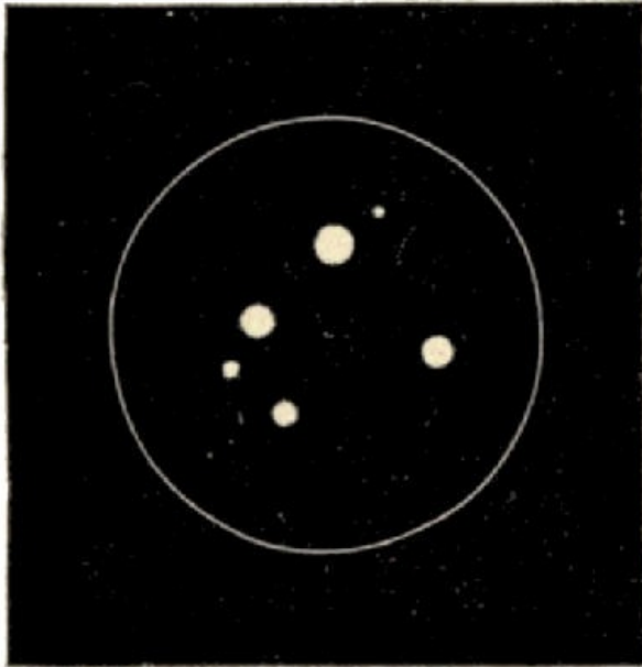
Fig. 98.—The Multiple star ( \theta Orionis) in the Great Nebula of Orion.
