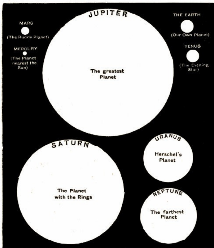
Fig. 35.—Comparative Sizes of the Planets.
