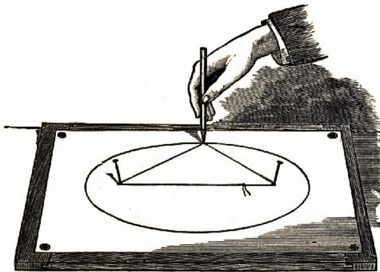
Fig. 37.—Drawing an Ellipse.
