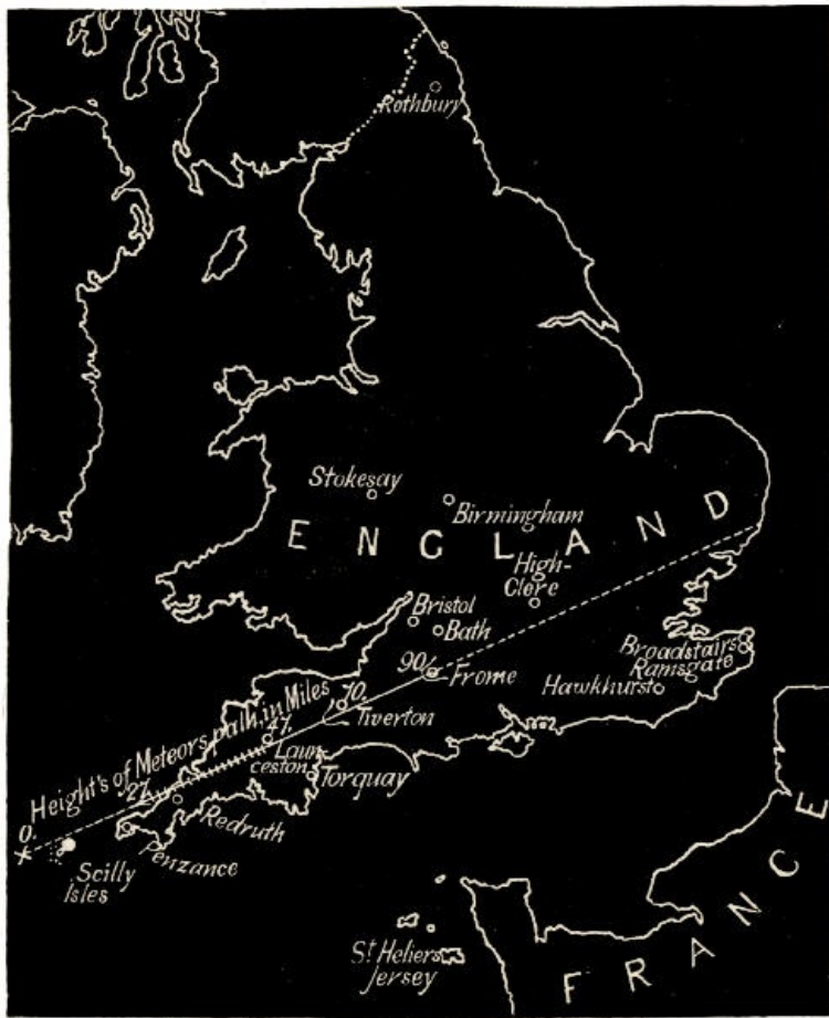
Fig. 75.—The Path of the Fireball of November 6th, 1869.
