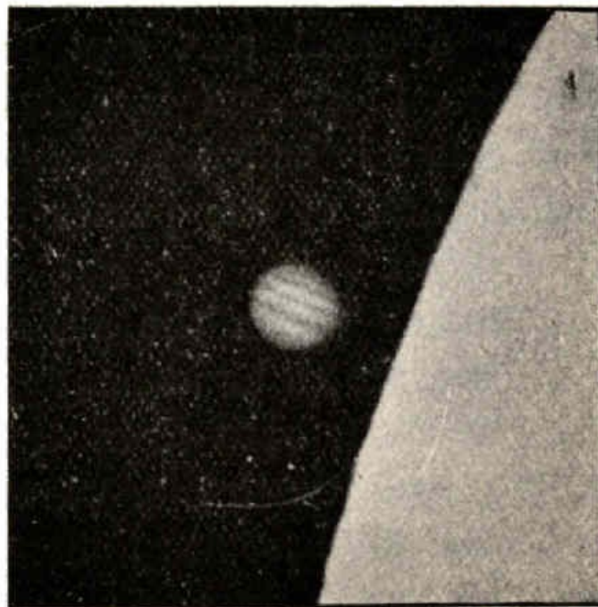
Fig. 57.—The Occultation of Jupiter (1).
