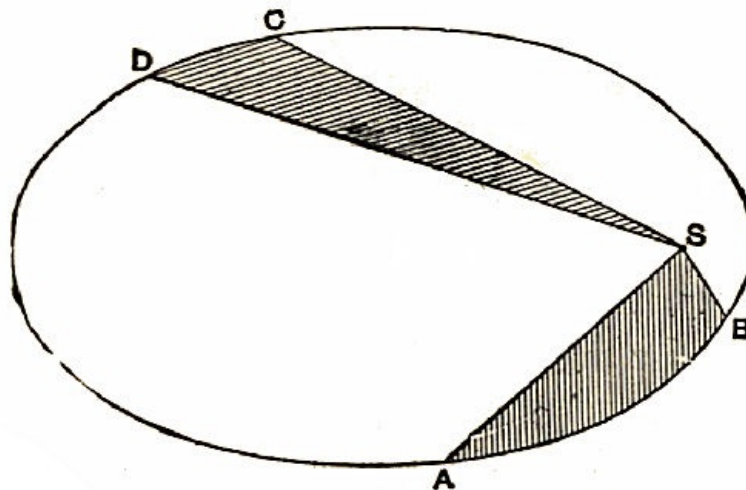
Fig. 39.—Equal Areas in Equal Times.
