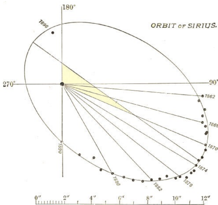
Fig. 92.—The Orbit of Sirius (Professor Burnham).
