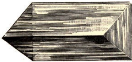
Fig. 17.—The Prism.
