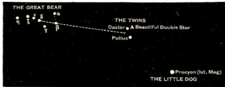
Fig. 86.—Castor and Pollux.
