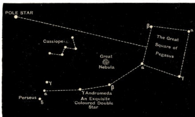
Fig. 82.—The Great Square of Pegasus.
