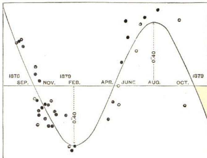
Fig. 95.—Parallax in Declination of 61 Cygni.
