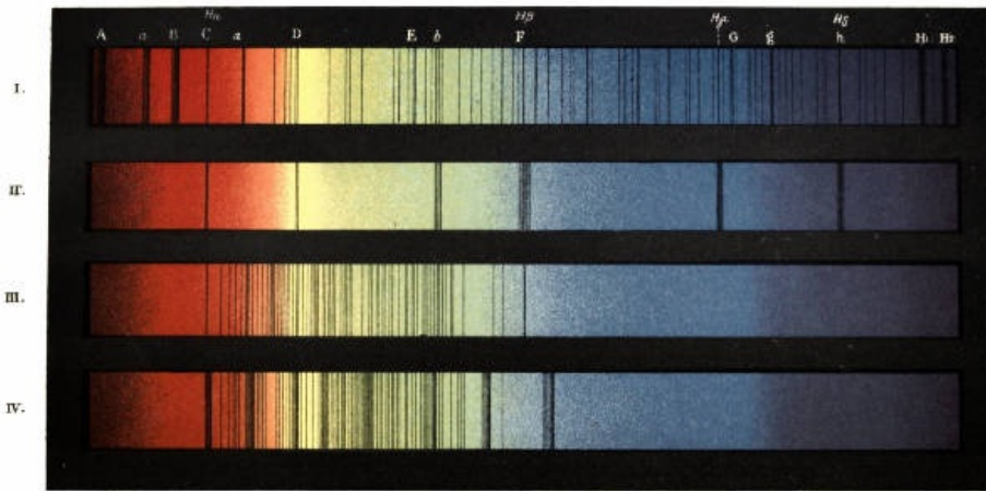
PLATE XIII. SPECTRA OF THE SUN AND STARS. I. SUN. II. SIRIUS. III. ALDEBARAN. IV. BETELGEUZE.
