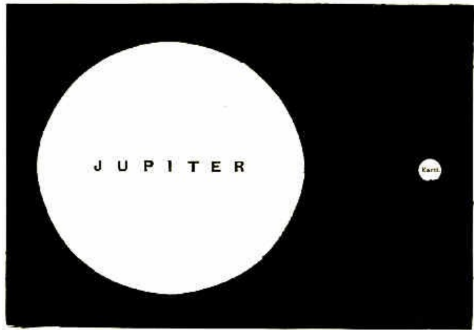
Fig. 56.—The Relative Dimensions of Jupiter and the Earth.
