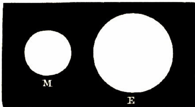
Fig. 50.—Relative Sizes of Mars and the Earth.
