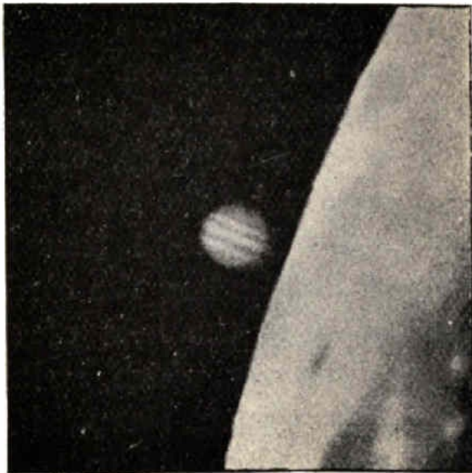
Fig. 58.—The Occultation of Jupiter (2).
