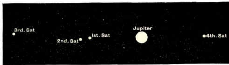
Fig. 61.—Jupiter and his Four Satellites as seen in a Telescope of Low Power.
