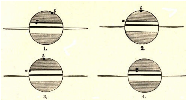
Fig. 68.—Transit of Titan and its Shadow, by F. Terby Louvain, 12th April, 1892.
