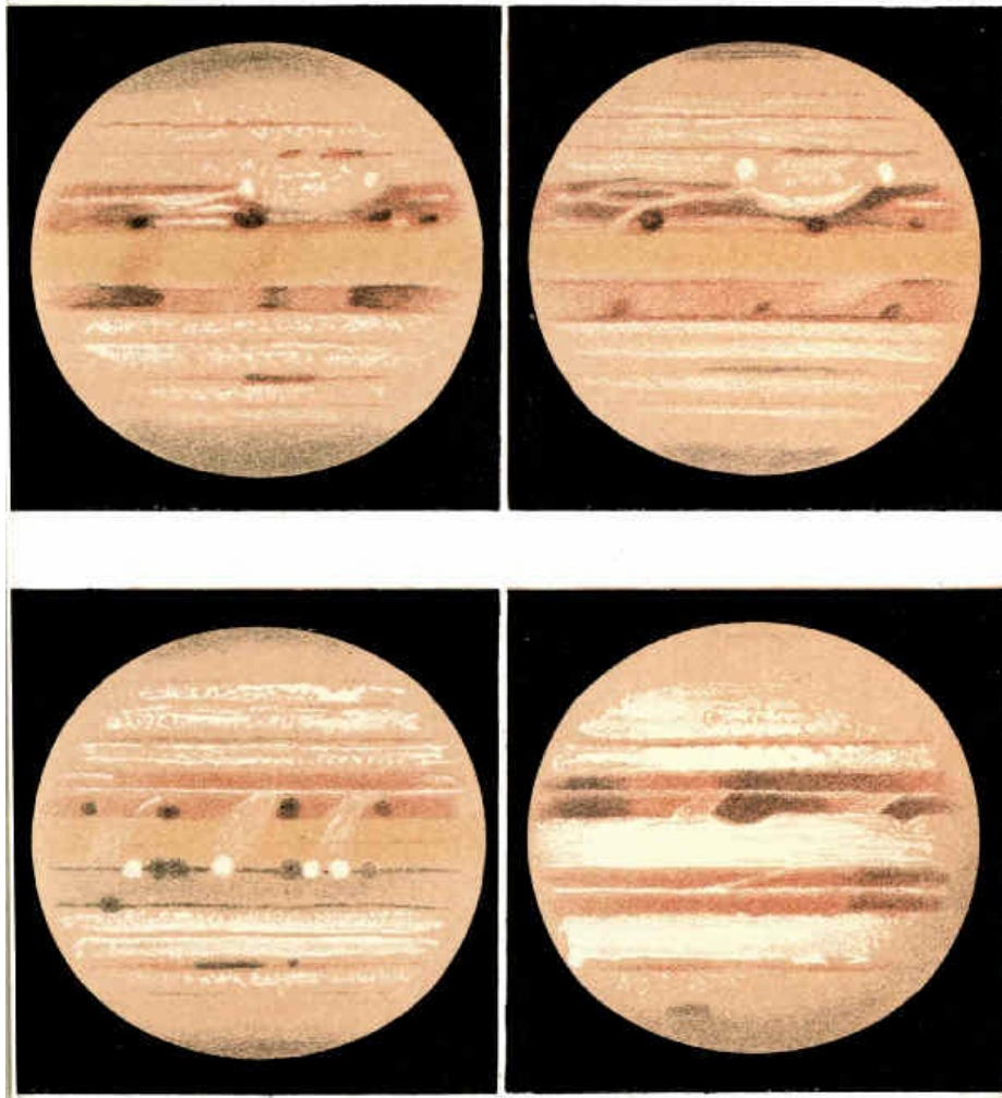
PLATE XI. Feb. 2nd. Feb. 4th. Feb. 12th. Feb. 28th. THE PLANET JUPITER. 1897.
