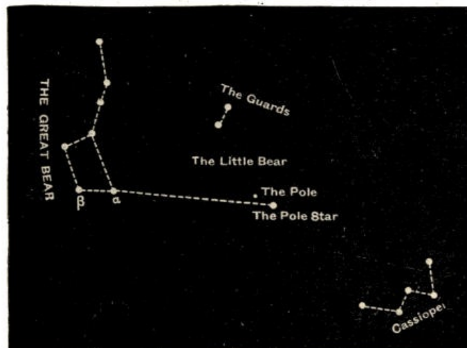
Fig. 81.—The Great Bear and Cassiopeia.
