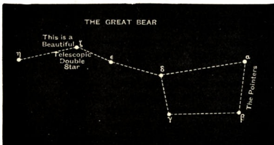
Fig. 9.—The Great Bear.
