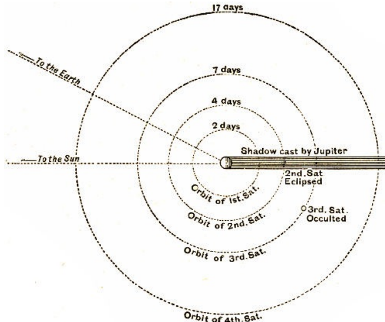
Fig. 62.—Disappearances of Jupiter's Satellites.
