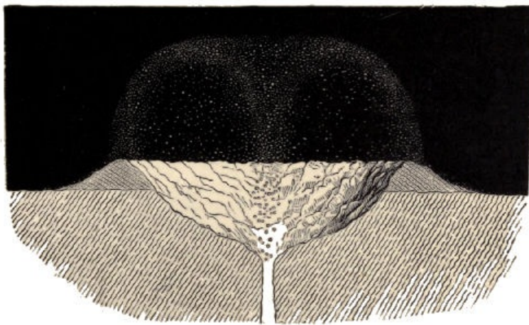
Fig. 28.—Volcano in Activity.
