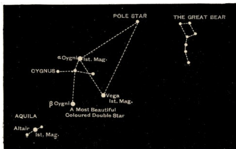
Fig. 91.—Vega, the Swan, and the Eagle.
