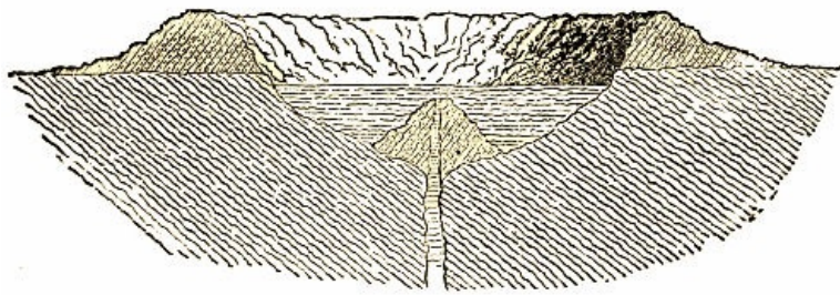
Fig. 30.—Formation of the Level Floor by Lava.
