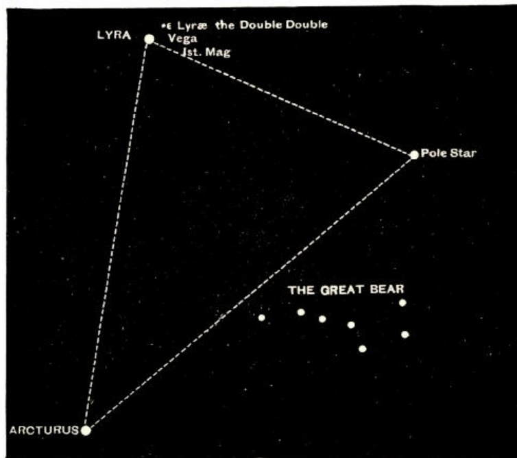
Fig. 90.—The Constellation of Lyra.
