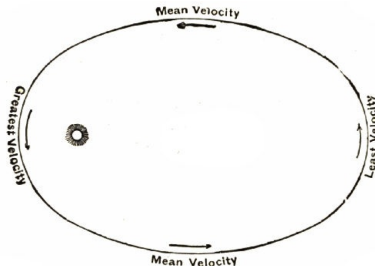
Fig. 38.—Varying Velocity of Elliptic Motion.
