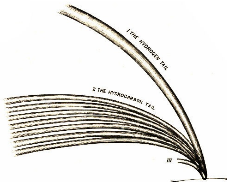
Fig. 72.—Bredichin's Theory of Comets' Tails.
