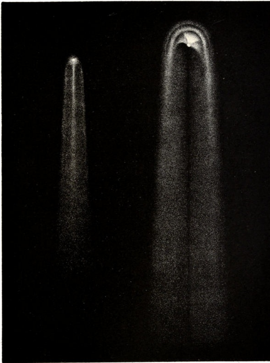
PLATE XII. COGGIA'S COMET.
