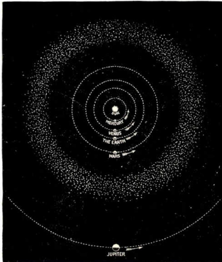
Fig. 55.—The Zone of Minor Planets between Mars and Jupiter.
