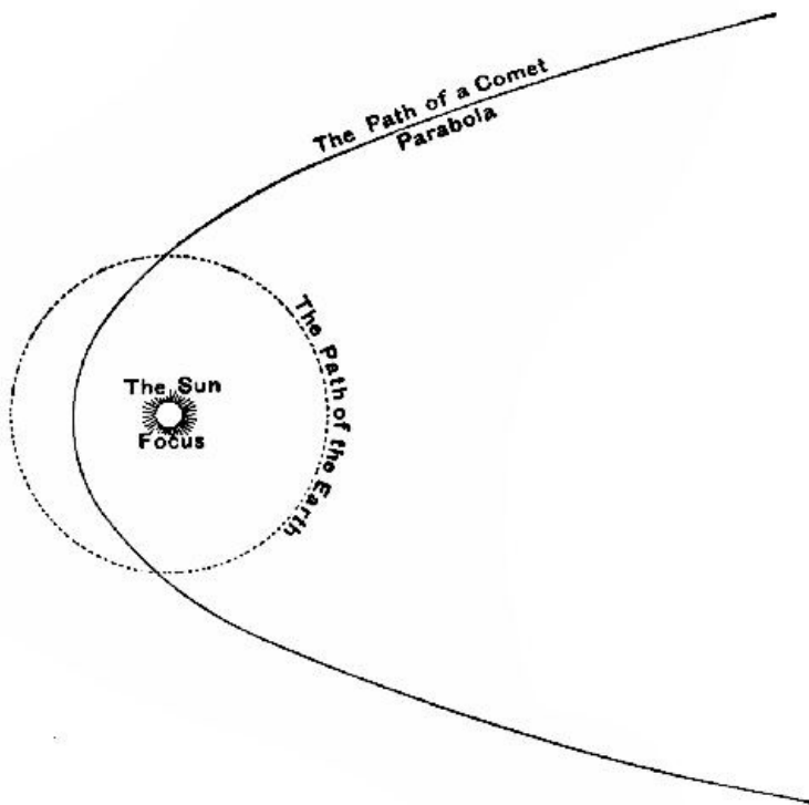
Fig. 69.—The Parabolic Path of a Comet.
