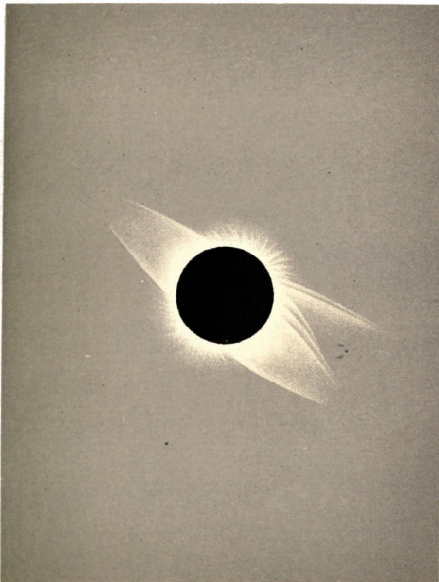
Fig. 20.—View of the Corona (and a Comet) in a Total Eclipse.
