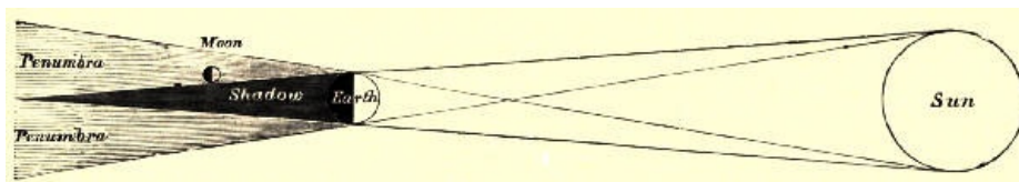
Fig. 26.—Form of the Earth's Shadow, showing the Penumbra, or partially shaded region. Within the Penumbra, the Moon is visible; in the Shadow it is nearly invisible.
