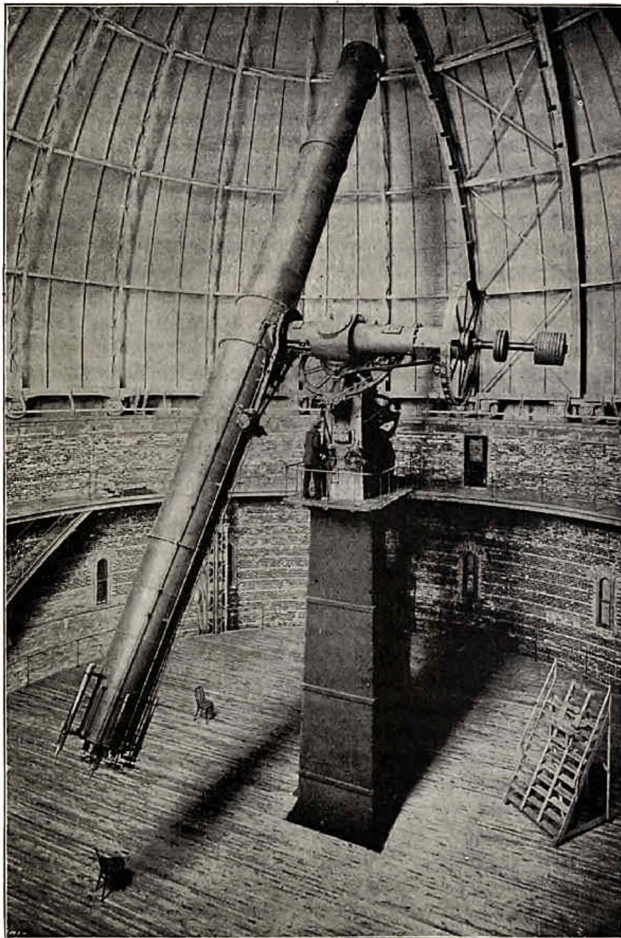
Fig. 4.—The Telescope at Yerkes Observatory, Chicago. (From the Astrophysical Journal , Vol. vi., No. 1.)
