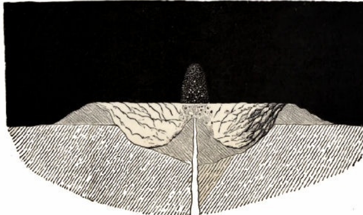
Fig. 29.—Subsequent Feeble Activity.
