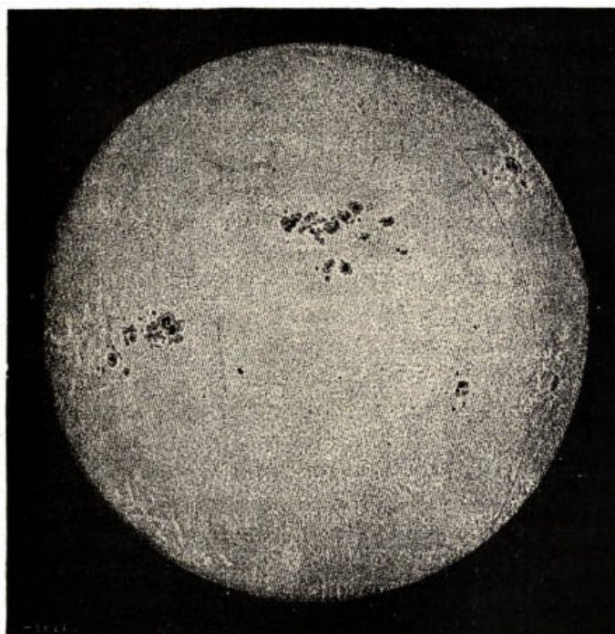
Fig. 11.—The Sun, photographed on September 22, 1870.
