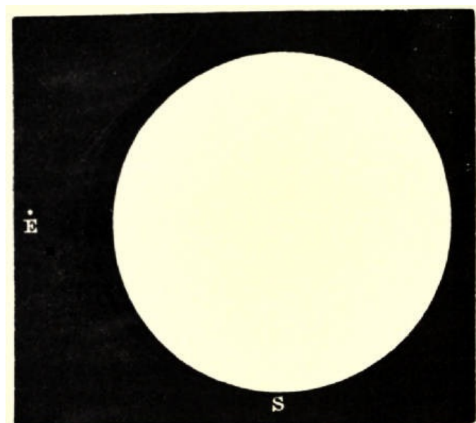
Fig. 10.—Comparative Size of the Earth and the Sun.
