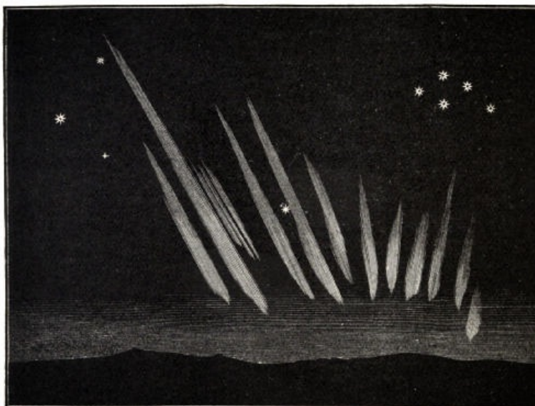
Fig. 74.—The Comet of 1744.
