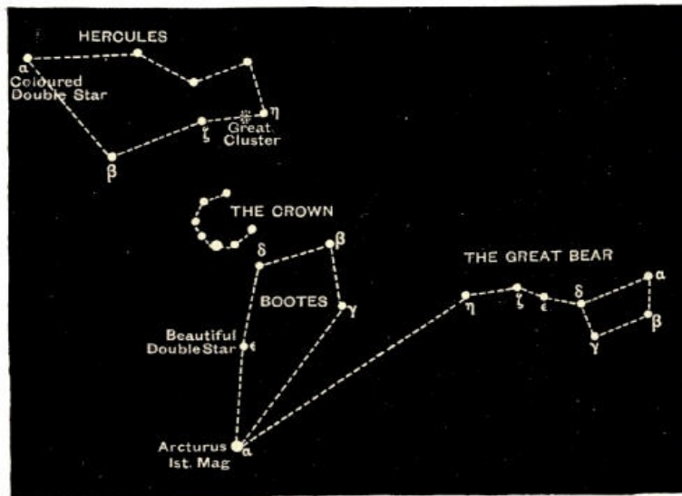
Fig. 88.—Boötes and the Crown.
