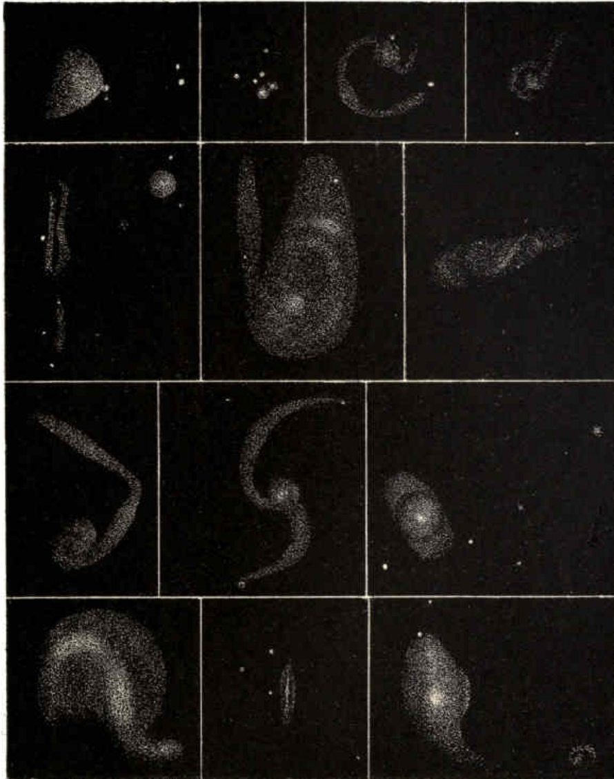
PLATE XVI. NEBULÆ OBSERVED WITH LORD ROSSE'S GREAT TELESCOPE.
