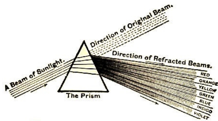
Fig. 18.—Dispersion of Light by the Prism.
