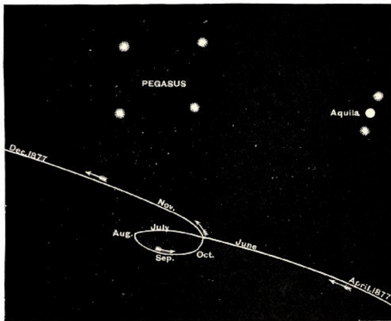
Fig. 49.—The Apparent Movements of Mars In 1877.
