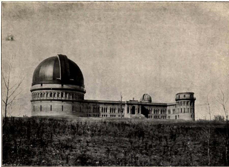
Fig. 6.—South Front of the Yerkes Observatory, Chicago. (From the Astrophysical Journal , Vol. vi., No. 1.)
