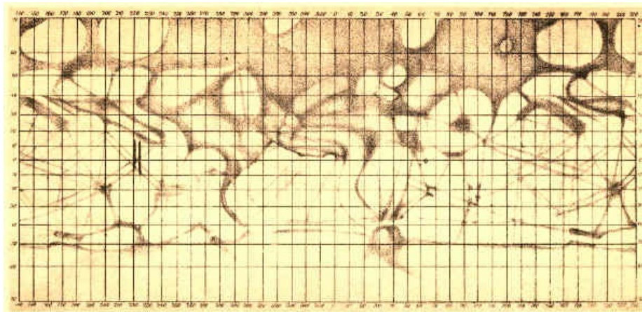
PLATE XVIII. SCHIAPARELLI'S MAP OF MARS IN 1881-82.
