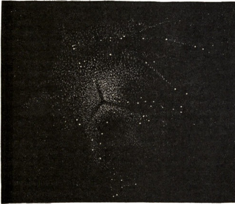
Fig. 96.—The Globular Cluster in Hercules.
