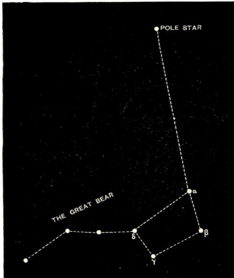
Fig. 80.—The Great Bear and Pole Star.
