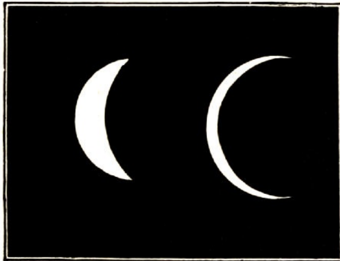
Fig. 42.—Mercury as a Crescent.
