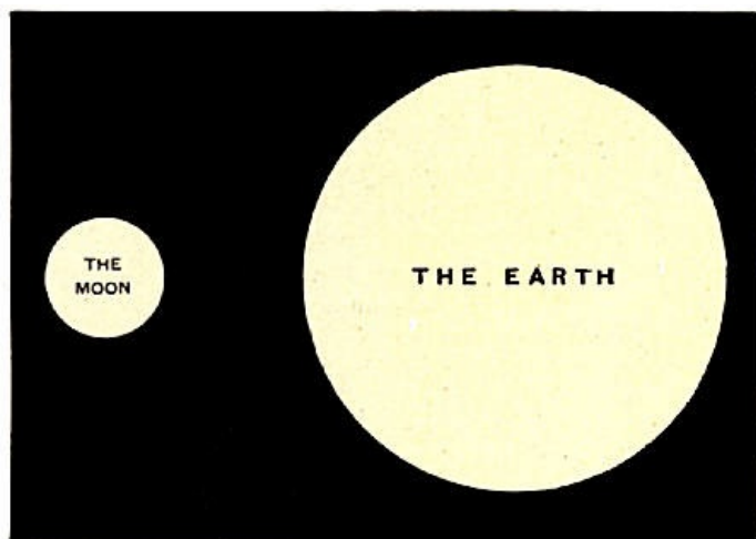
Fig. 23.—Comparative Sizes of the Earth and the Moon.
