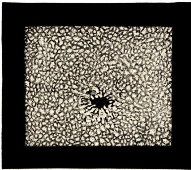
Fig. 16.—The Texture of the Sun and a small Spot.
