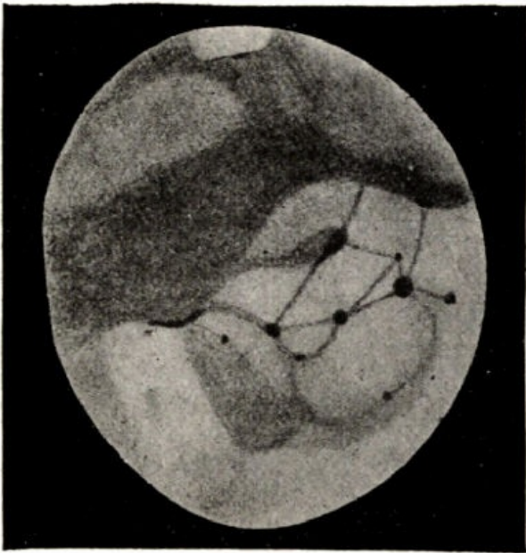
Fig. 51.—Drawing of Mars (July 30th, 1894).
