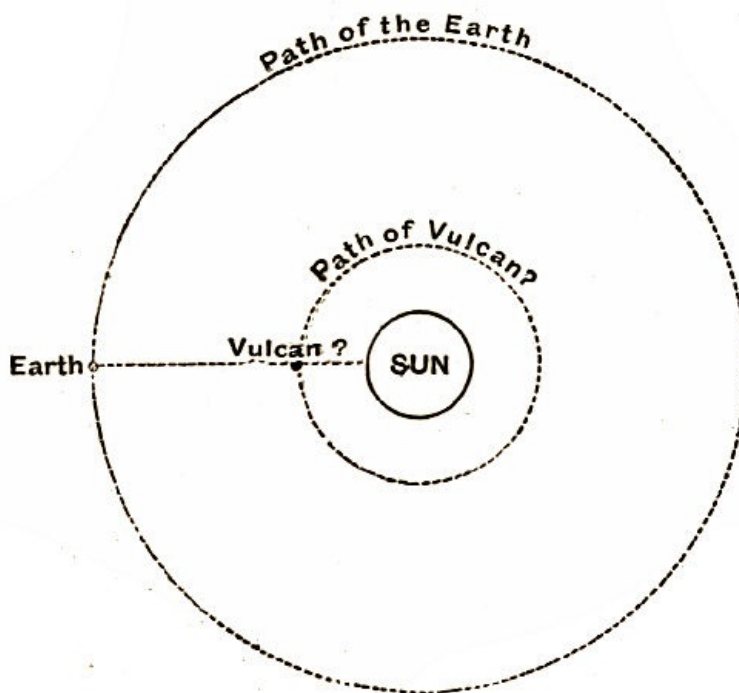
Fig. 40.—The Transit of the Planet of Romance.
