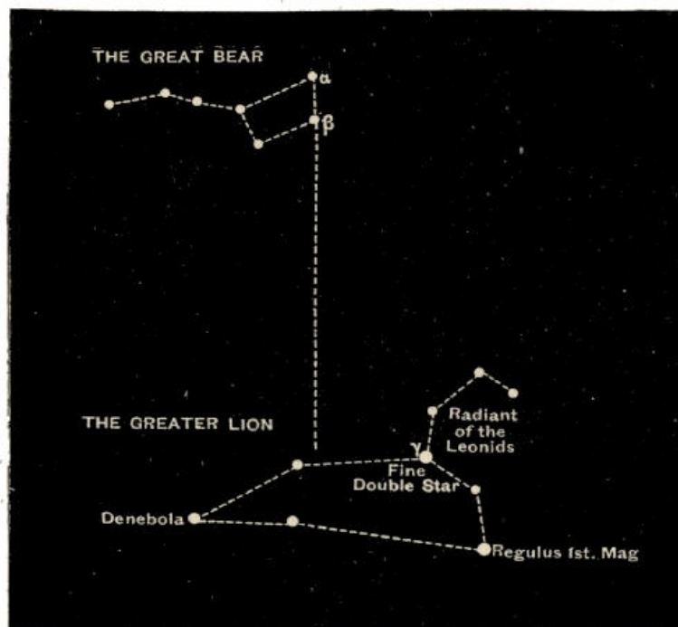
Fig. 87.—The Great Bear and the Lion.
