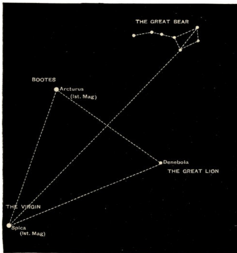
Fig. 89.—Virgo and the neighbouring Constellations.
