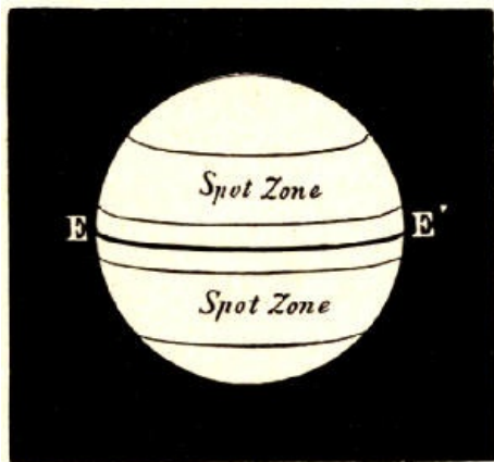
Fig. 15.—Zones on the Sun's Surface in which Spots appear.
