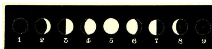
Fig. 25.—The Phases of the Moon.
