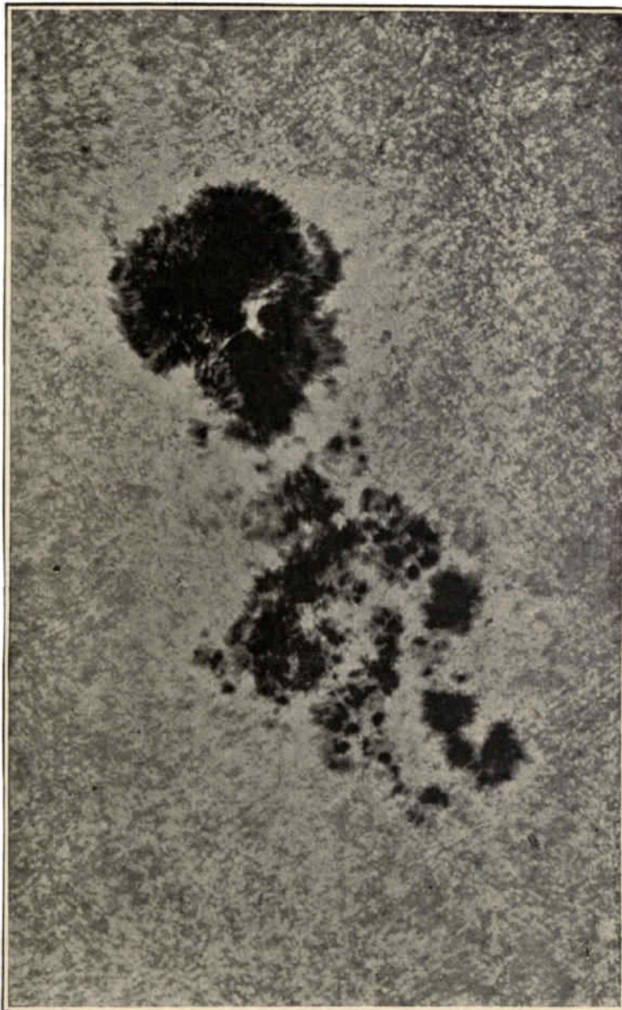
Fig. 12.—Photograph of the Solar Surface.
