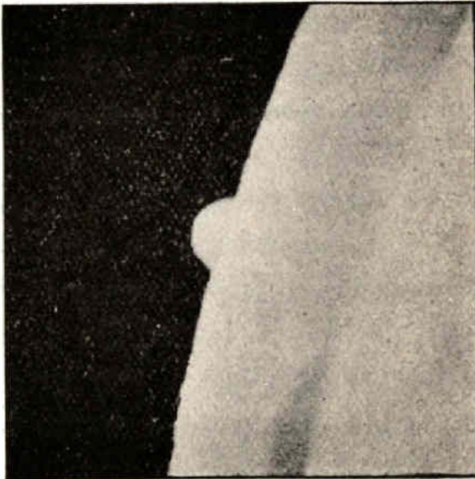
Fig. 59.—The Occultation of Jupiter (3).
