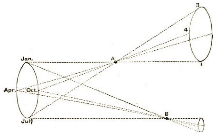
Fig. 93.—The Parallax Ellipse.
