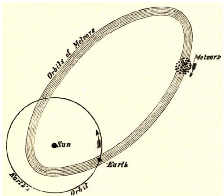
Fig. 76.—The Orbit of a Shoal of Meteors.
