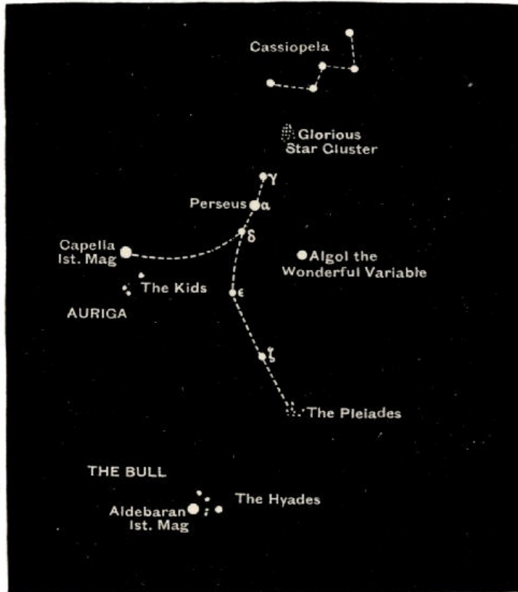
Fig. 83.—Perseus and its Neighbouring Stars.
