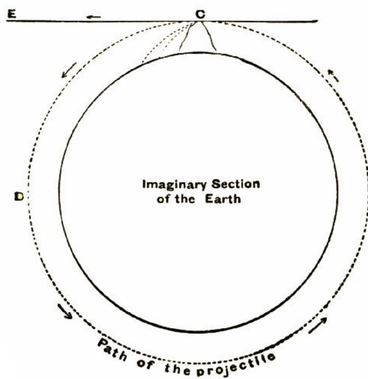
Fig. 36.—Illustration of the Moon's Motion.
