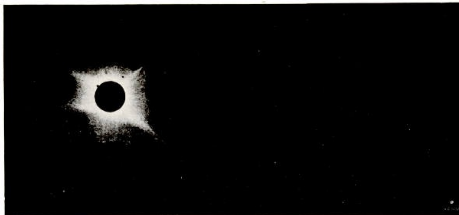
Fig. 21.—View of Corona during the Eclipse of Jan. 22nd, 1898 (Reproduced by kind permission of Mr. and Mrs. Maunder and of the proprietors of "Knowledge.")
