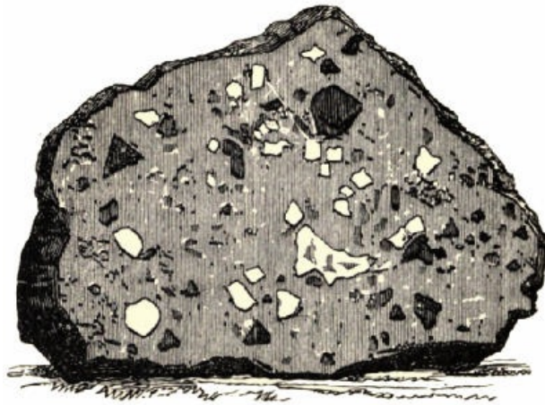
Fig. 79.—Section of the Chaco Meteorite.
