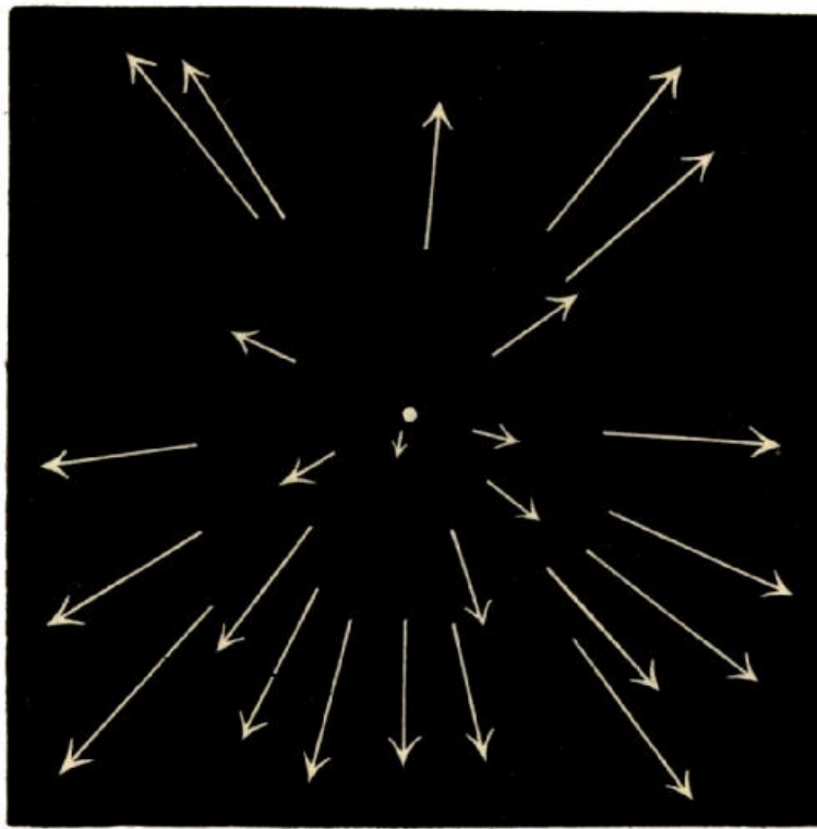
Fig. 77.—The Radiant Point of Shooting Stars.
