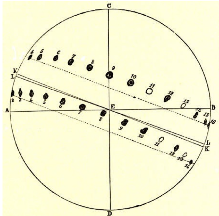
Fig. 14.—Scheiner's Observations on Sun-spots.
