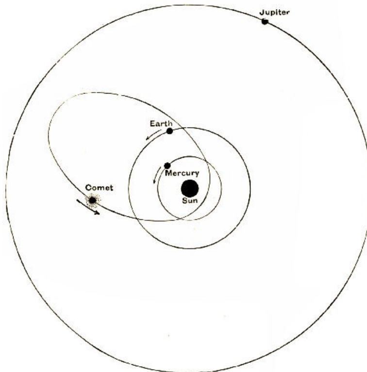
Fig. 70.—The Orbit of Encke's Comet.
