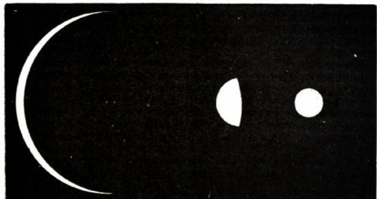
Fig. 44.—Different Aspects of Venus in the Telescope.
