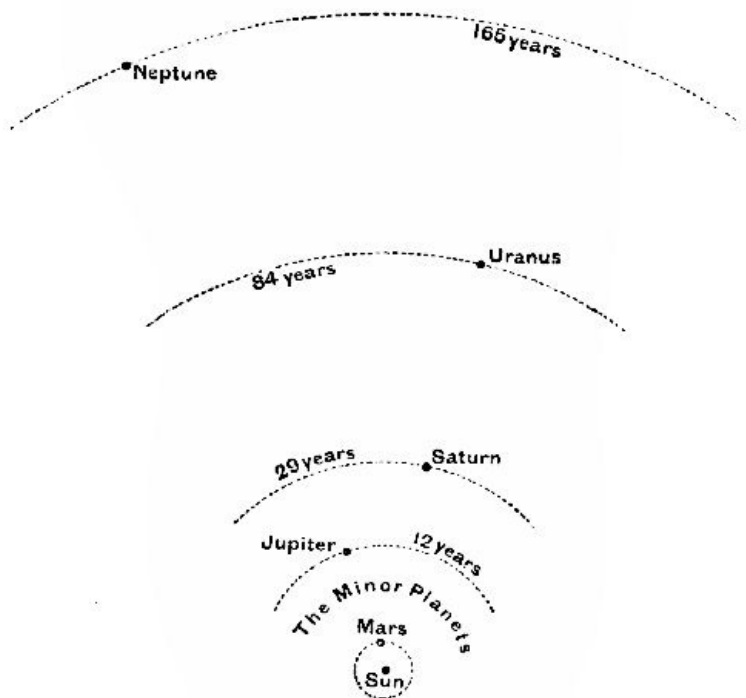
Fig. 33.—The Orbits of the Four Giant Planets.
