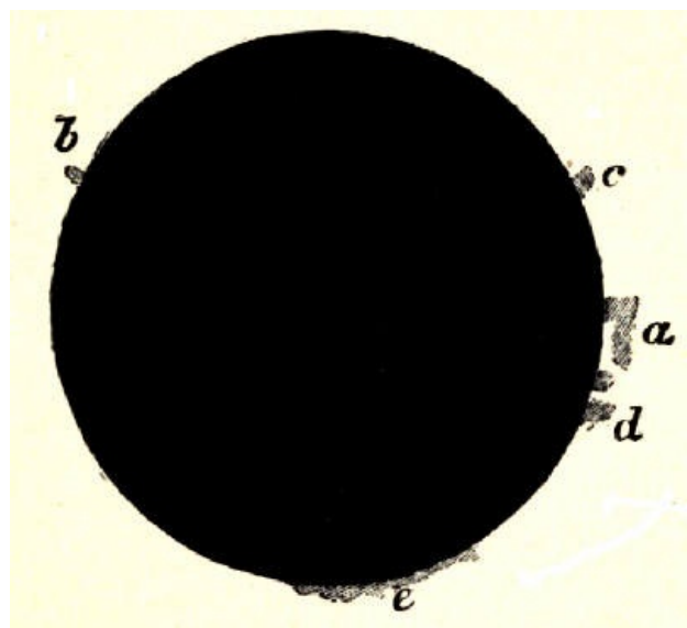
Fig. 19.—Prominences seen in Total Eclipse.
