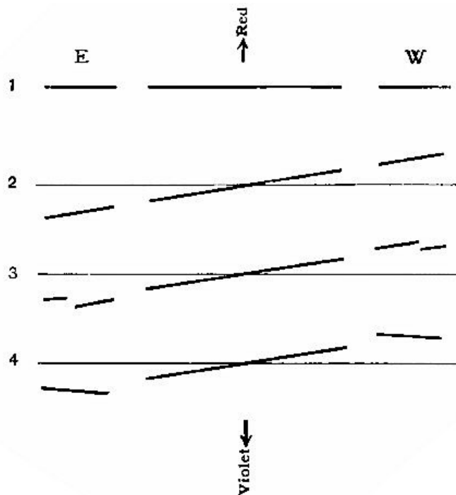
Fig. 67.—Prof. Keeler's Method of Measuring the Rotation of Saturn's Ring.
