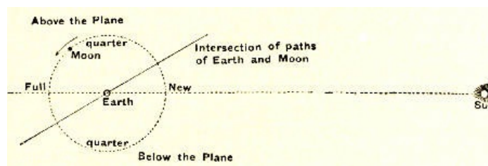
Fig. 24.—The Moon's Path around the Sun.
