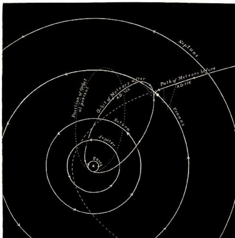
Fig. 78.—The History of the Leonids.
