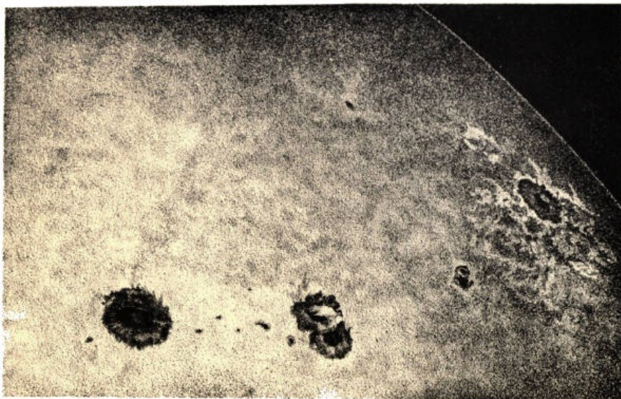
PLATE III. SPOTS AND FACULÆ ON THE SUN. (FROM A PHOTOGRAPH BY MR. WARREN DE LA RUE, 20TH SEPT., 1861.)
