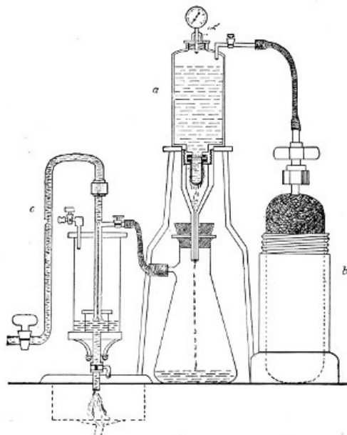
Fig. 38.—Pakes' filtering reservoir— pressure and aspiration.
