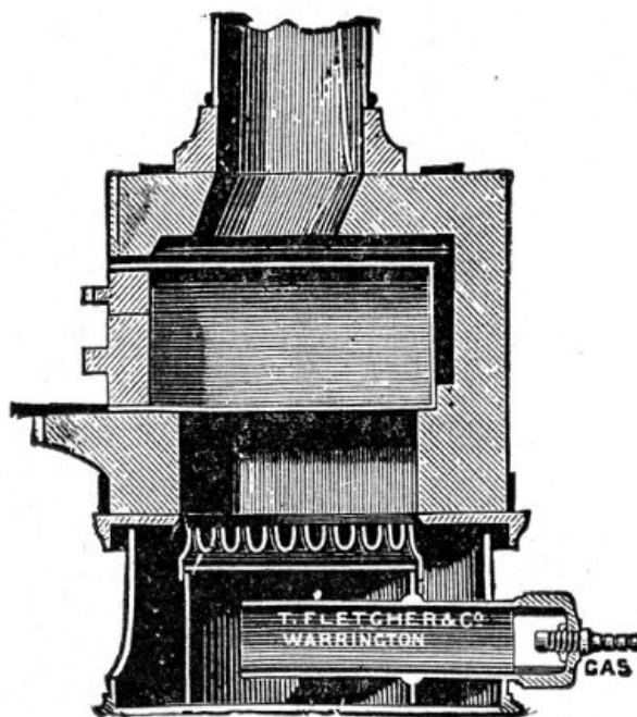
Fig. 25.—Muffle furnace.
