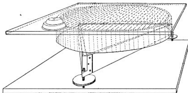
Fig. 122.—Plate-levelling stand.
