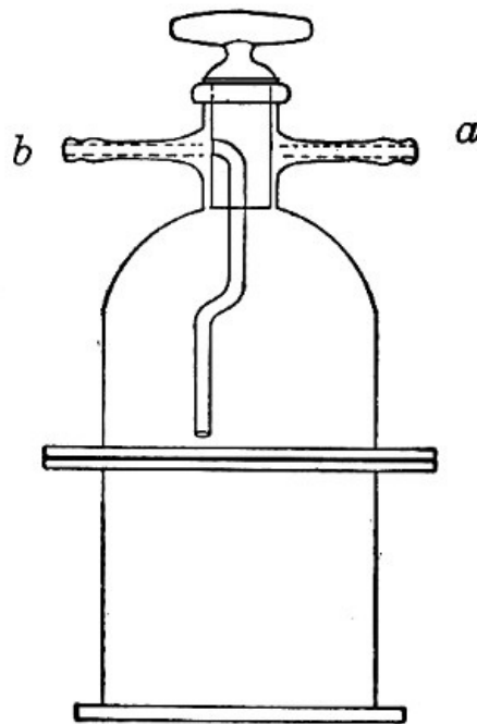
Fig. 135.—Novy's jar for plate cultivations.
