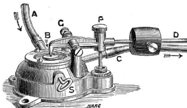
Fig. 116.—Capsule thermo-regulator.
