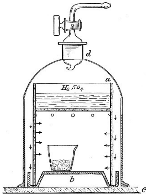
Fig. 157.—Mueller's desiccator.
