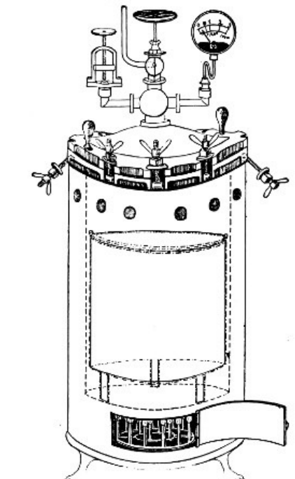
Fig. 30.—Chamberland's Autoclave.
