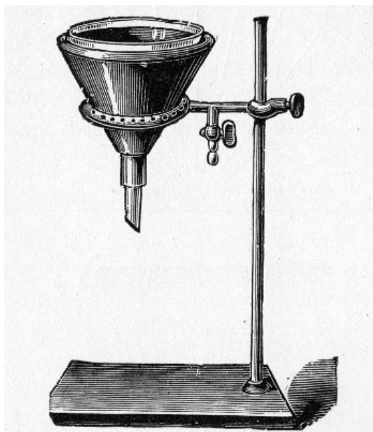
Fig. 101.—Hot-water filter funnel and ring burner.
