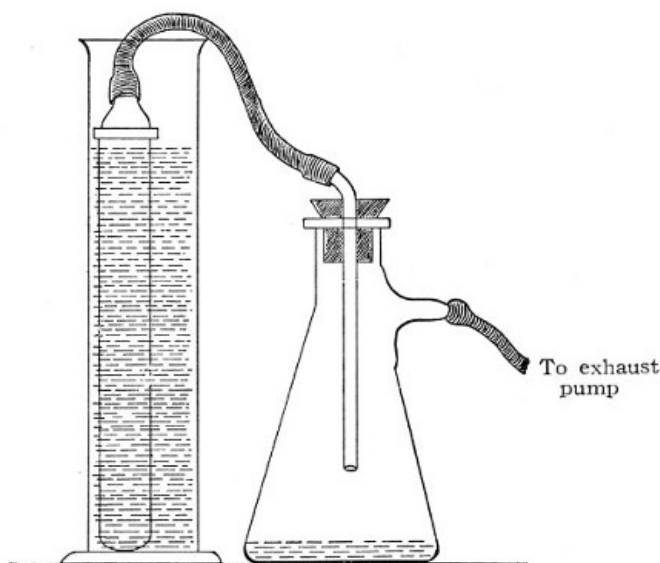
Fig. 39.—Closed candle arranged for filtering.
