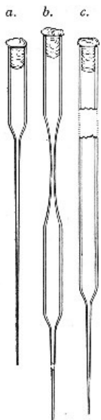
Fig. 13.—Capillary pipettes. a, b, c.
