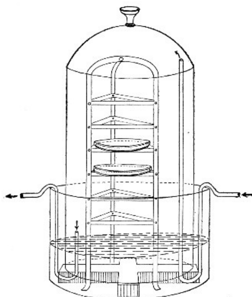
Fig. 134.—Botkin's apparatus.
