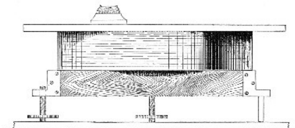
Fig. 123.—Plate-levelling stand, side view.
