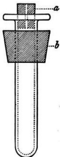
Fig. 34.—Porcelain filter candle.
