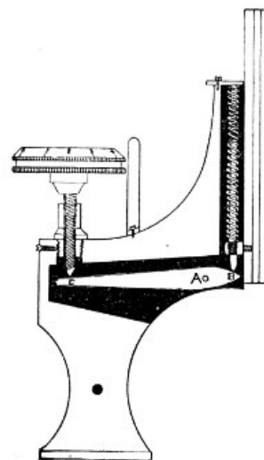
Fig. 43.—Fine adjustment.
