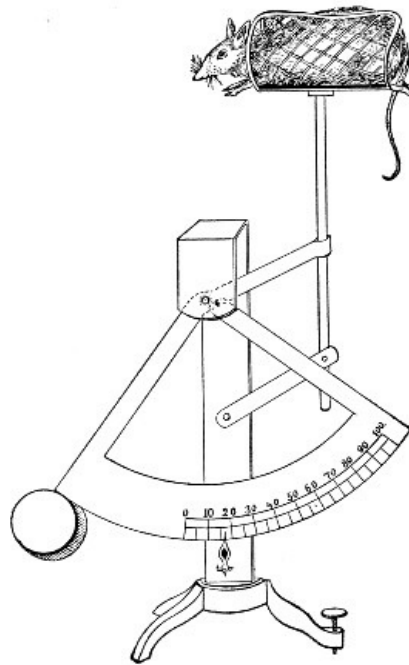
Fig. 167.—Mouse scales
