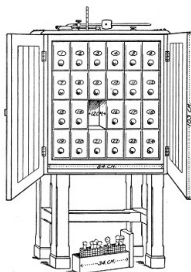
Fig. 114.—Cellular incubator.
