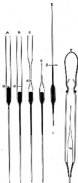
Fig. 19.—Making throttle pipettes—large capacity
