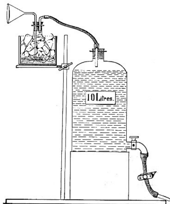
Fig. 216.—Arrangement of apparatus for air analysis.
