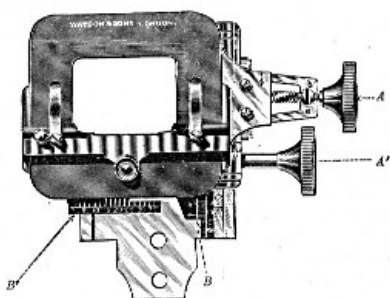
Fig. 45.—Mechanical stage.
