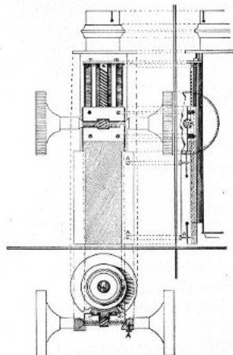
Fig. 42.—Coarse adjustment.
