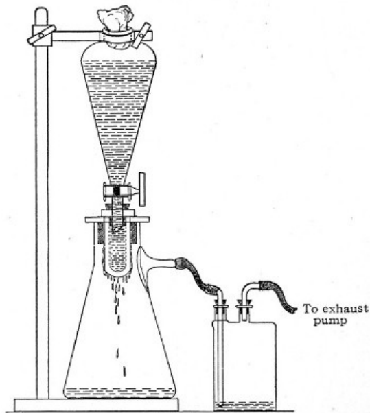
Fig. 37.—Apparatus arranged for filtering—aspiration.
