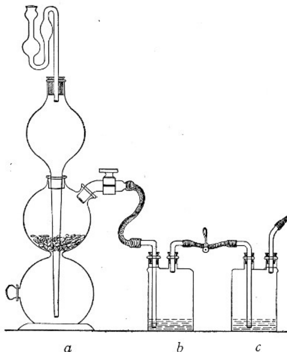
Fig. 132.—Kipp's hydrogen apparatus, (a) connected up to two washing bottles containing (b) lead acetate 10 per cent. solution, to remove H 2 S and (c) silver nitrate solution to remove AsH 3 . A third washing bottle containing pyrogallic acid 10 per cent. solution, rendered alkaline, to remove any trace of oxygen, is sometimes introduced.
