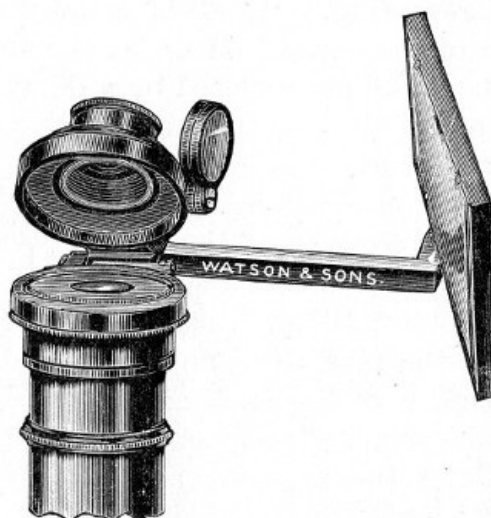
Fig. 55.—Camera lucida, Abbé pattern.
