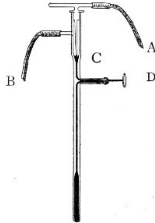
Fig. 115.—Reichert's thermo-regulator.
