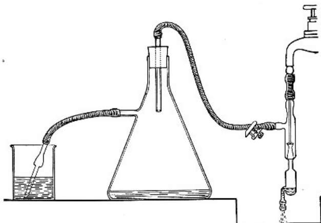
Fig. 22.—Cleaning blood pipettes.
