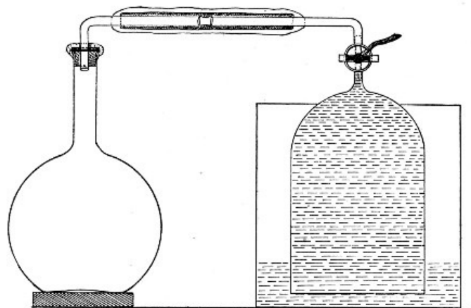
Fig. 153.—Gas-collecting apparatus.
