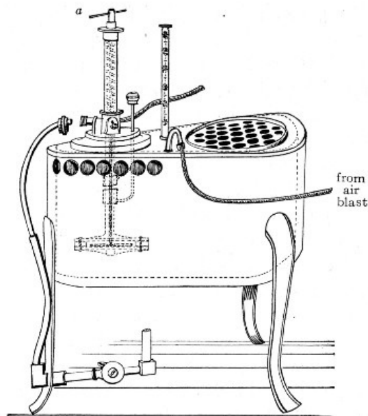
Fig. 155.—Hearson's water-bath.
