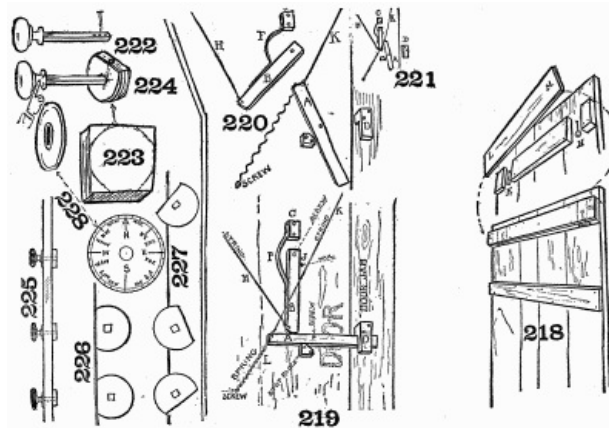
Home-made cabin door-locks.
