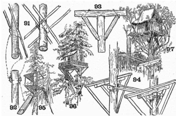
Details of tree-top houses.
