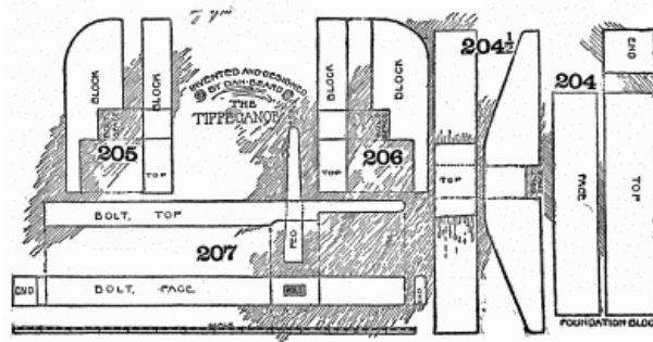
Detail parts of Tippecanoe door-latch.
