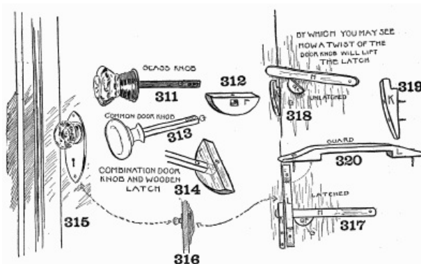
Details of combined door-knob and wooden latch.
