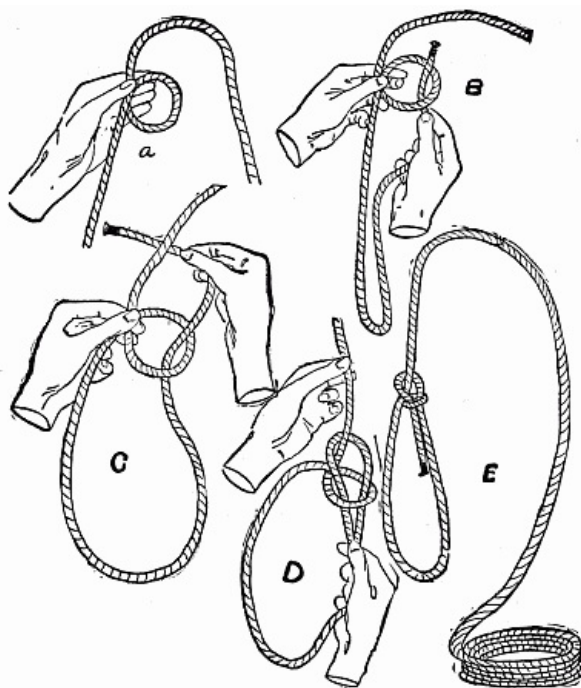
3. Bowline
