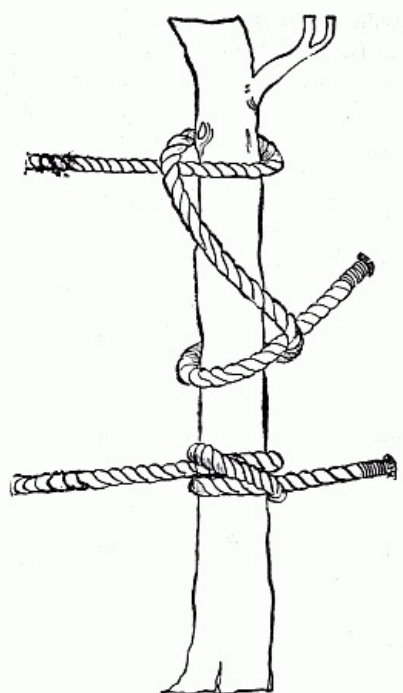
5. Clove-Hitch
