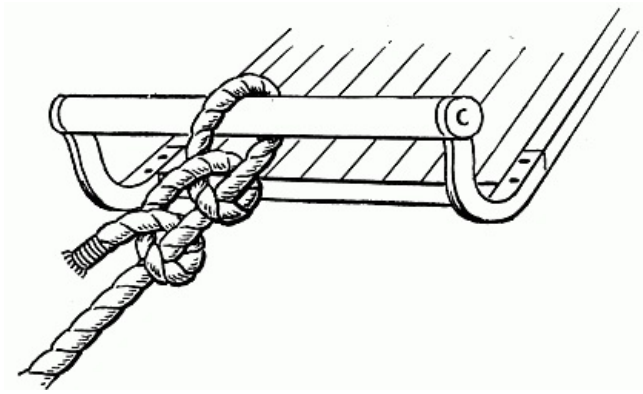
4. Two Half-Hitches
